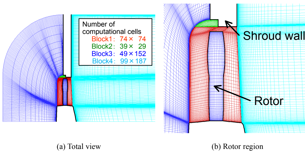
Fig. 7 Computational grid for half-ducted propeller fan.
