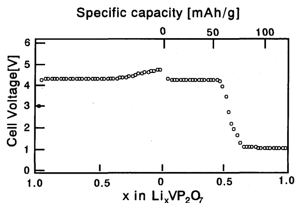
Fig. 4 Quasi-open circuit voltage profile of \text{LiVP}_2\text{O}_7 .
