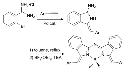
Scheme 2. Synthesis of aza-BODIPY derivative via aminoisoindoline.
