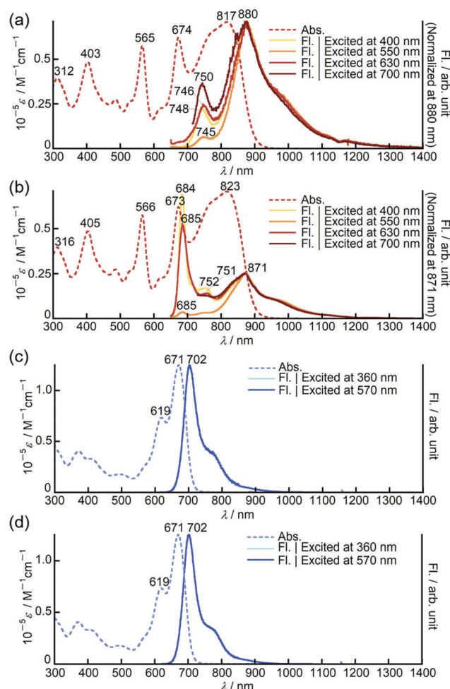
Fig. 26. UV/vis/NIR absorption (dashed lines) and fluorescence (solid lines) spectra of 38 in (a) \text{CHCl}_3 and (b) viscous solvents and 40 in (c) \text{CHCl}_3 and (d) viscous solvents. Reprinted with permission from ref. 56 Copyright 2018 RSC.
