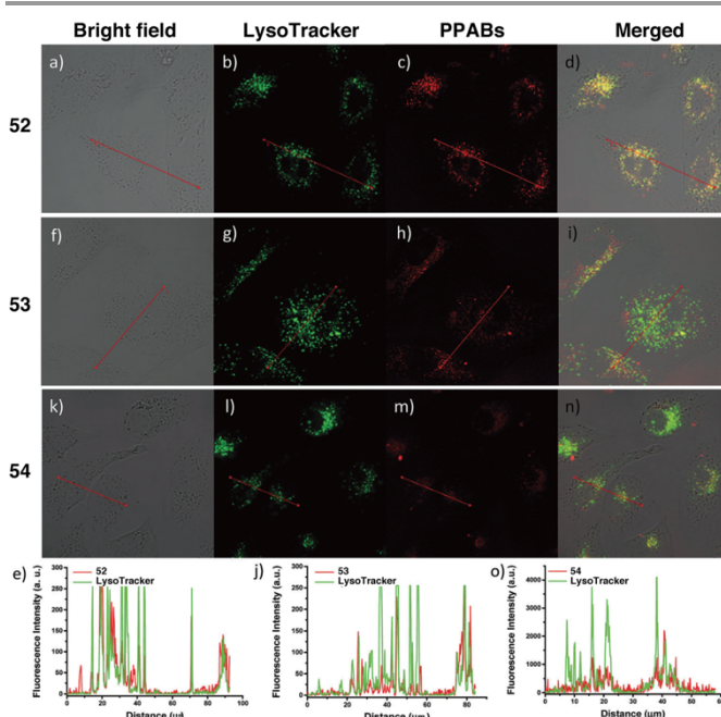
Fig. 36. Visualisation of the intracellular fluorescence of 52–54 (2 \mu\text{M} ) after 4 h incubation and LysoTracker Green (1.5 \mu\text{M} ) after 20 min incubation in HeLa cells: panels (a), (f) and (k): bright field images, panels (b), (g) and (l): fluorescence of LysoTracker Green, panels (c), (h) and (m) fluorescence of 52–54 and panels (d), (i) and (n) super imposed images. Panels (e), (j) and (o): fluorescence intensity profiles of PPABs (red line) and LysoTracker Green (green line) traced along the red lines in the corresponding images above. Redrawn with permission from ref. 71 Copyright 2018 RSC.
