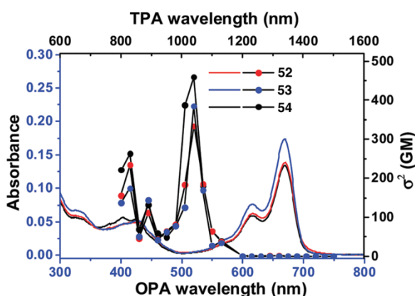
Fig. 35. Two-photon (segmented lines) and one-photon (solid lines) absorption spectra of 52–54 in deionised water containing 0.3% v/v Tween 80 and 1% v/v DMF. Redrawn with permission from ref. 71 Copyright 2018 RSC.
