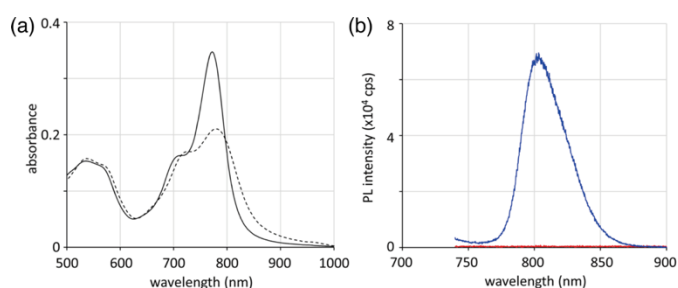
Fig. 39. (a) vis/NIR absorption spectra (0.1 mg/mL) of 55 in DMF (solid line) and water (dashed line). (b) Photoluminescence spectra ( \lambda_{\text{ex}} = 720 nm) of 55 in DMF (blue line) and water (red line). Redrawn with permission from ref. 77 Copyright 2017 ACS.
