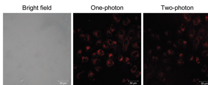
Fig. 37. One-photon ( \lambda_{\text{ex}} = 633 \text{ nm} , \lambda_{\text{em}} = 650\text{--}735 \text{ nm} ) and two-photon ( \lambda_{\text{ex}} = 633 \text{ nm} , \lambda_{\text{em}} = 650\text{--}735 \text{ nm} ) images of HeLa cells stained by 54 . Reprinted with permission from ref. 71 Copyright 2018 RSC.
