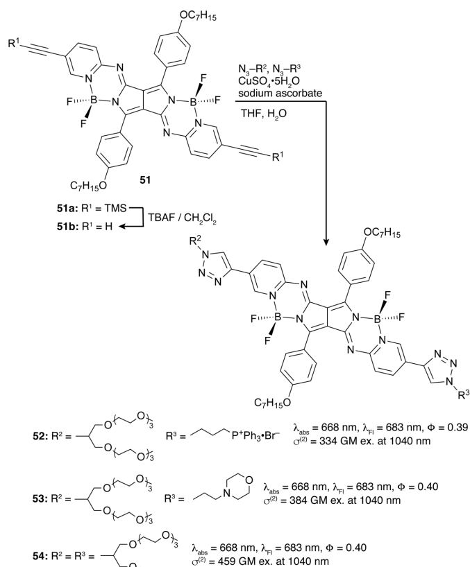
Scheme 14. Synthesis of hydrophilic PPABs 52–54 and optical properties in deionised water (with 0.3% v/v Tween 80 and 1% v/v DMF).
