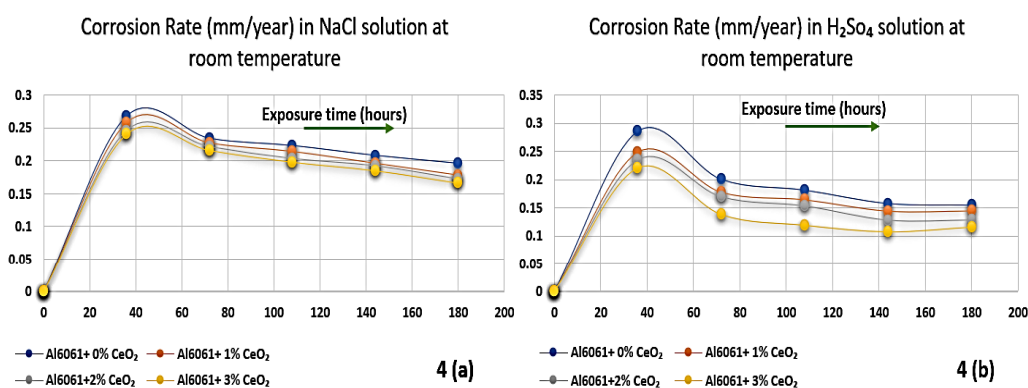
Figure 4 (a and b): COR of AlMMNCs samples at room temperature in aqueous solutions
