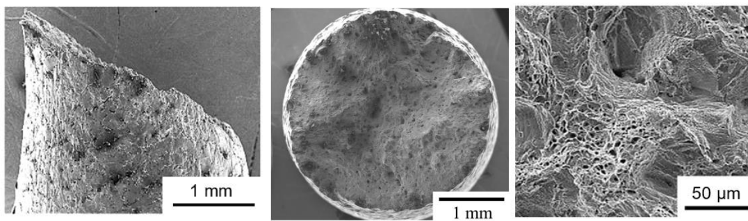
(b) \sigma = 310 \text{ MPa} , t_r = 43 \text{ h}
