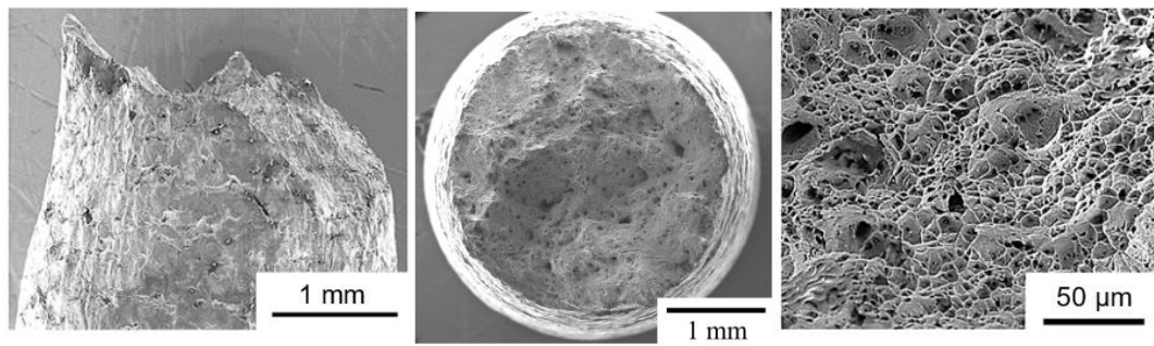
(a) \sigma = 320 \text{ MPa} , t_r = 9.9 \text{ h}
