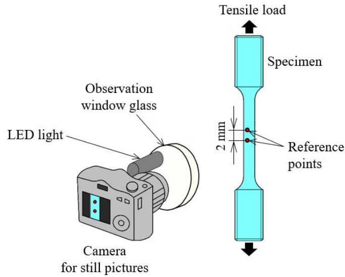
Figure 2.12 Strain measurement by the DIC method in this study.
