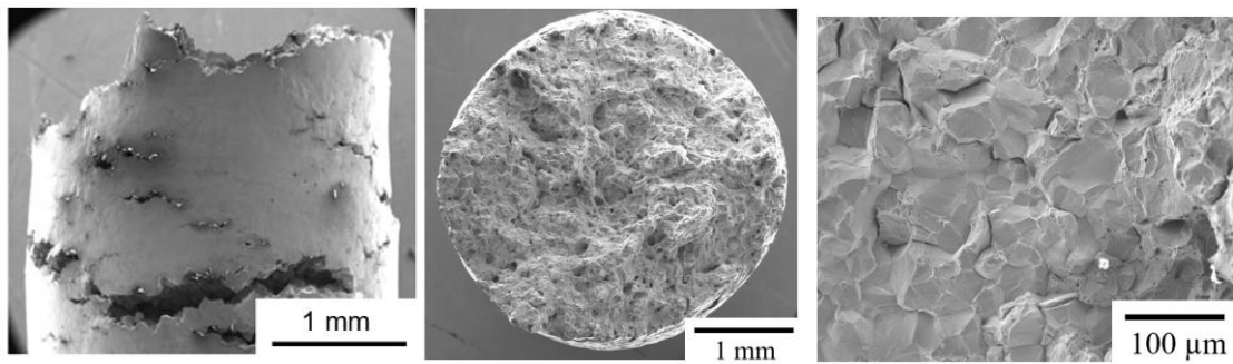
(c) \sigma = 270 \text{ MPa} , t_r = 208 \text{ h}
