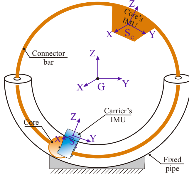
Figure 3.1: Experimental setup and frame transformations.
