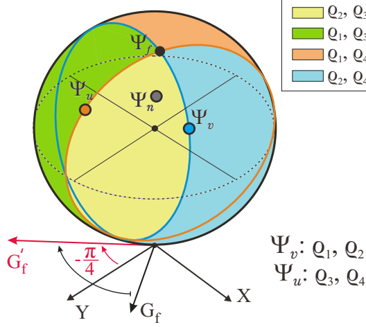
Figure B.3: Sectioned sphere based on the \Psi_v and \Psi_u cutting planes for directional updates of \zeta_q . Note that \Psi_v and \Psi_u are on \varrho_2 and \varrho_3 as an example.
