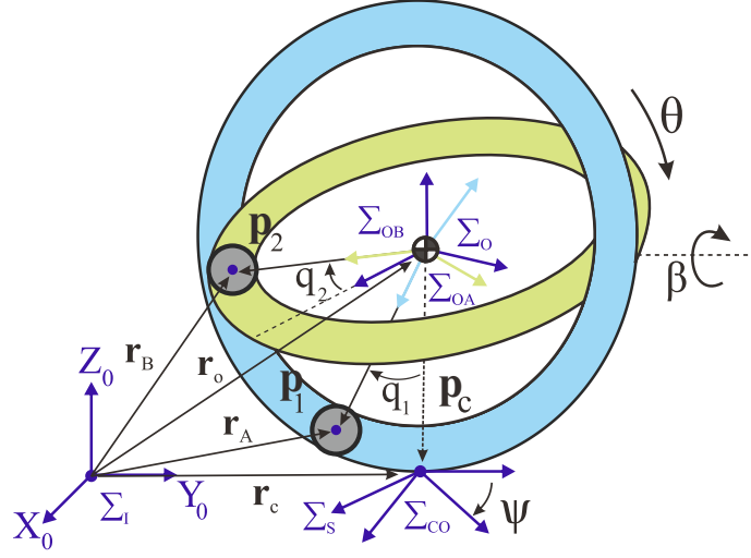
Figure 2.2: The rolling robot with introduced basic vectors.
