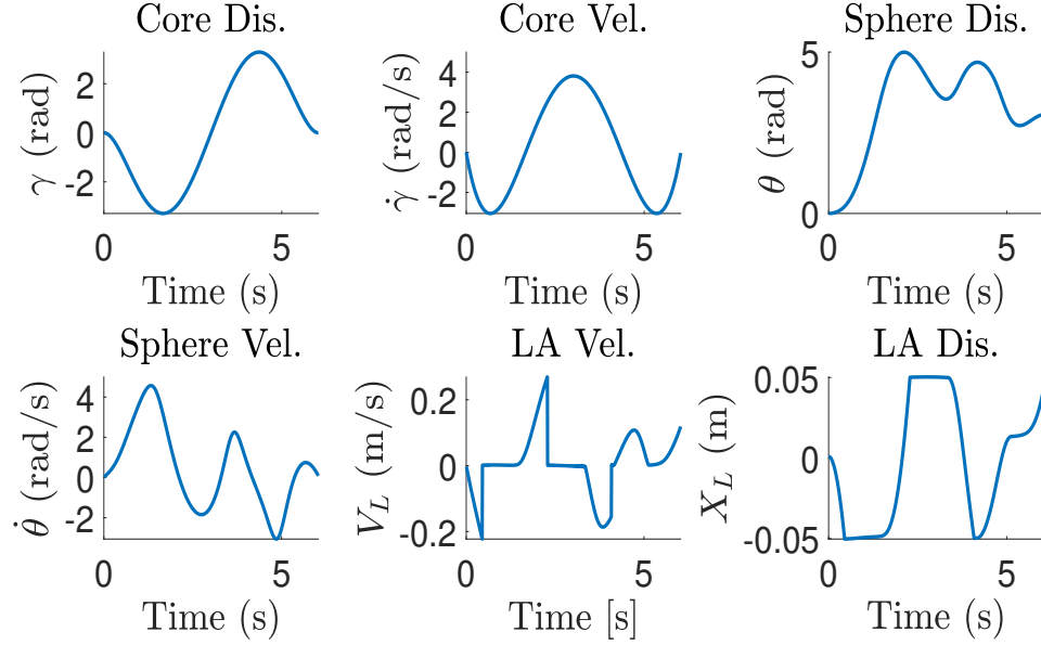
Figure 2.20: Results of inverse dynamics in simulation of the first case.
