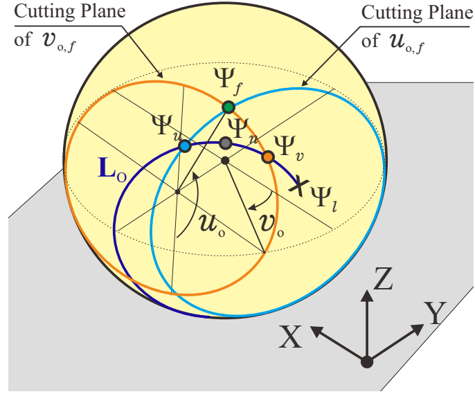
Figure 5.11: Parametrization of the curve \mathbf{L}_o by cutting planes of u_{o,f} and v_{o,f} .
