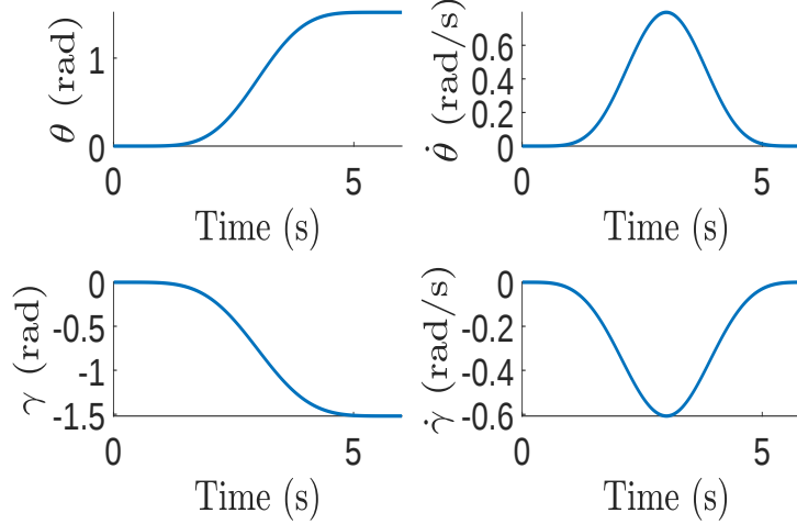
Figure 4.4: Example simulation for passive carrier \{\theta, \dot{\theta}\} and rotating mass-point \{\gamma, \dot{\gamma}\} states by the modified model.
