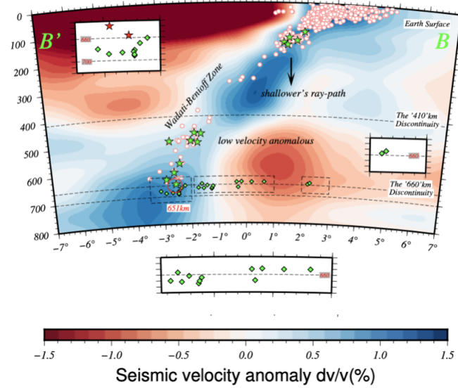
Figure 10: Cross Sections AA' (upper) and BB' (lower) of Kurile Region. Blue and red background colors correspond to high and low-speed anomalies through the tomography models. Red circles represent the earthquakes and those S660P are observed ones are shown by green stars. S-to-P conversion points are shown by green squares, areas surrounded by dotted lines are expanded in the insert figures with same coordinates.
