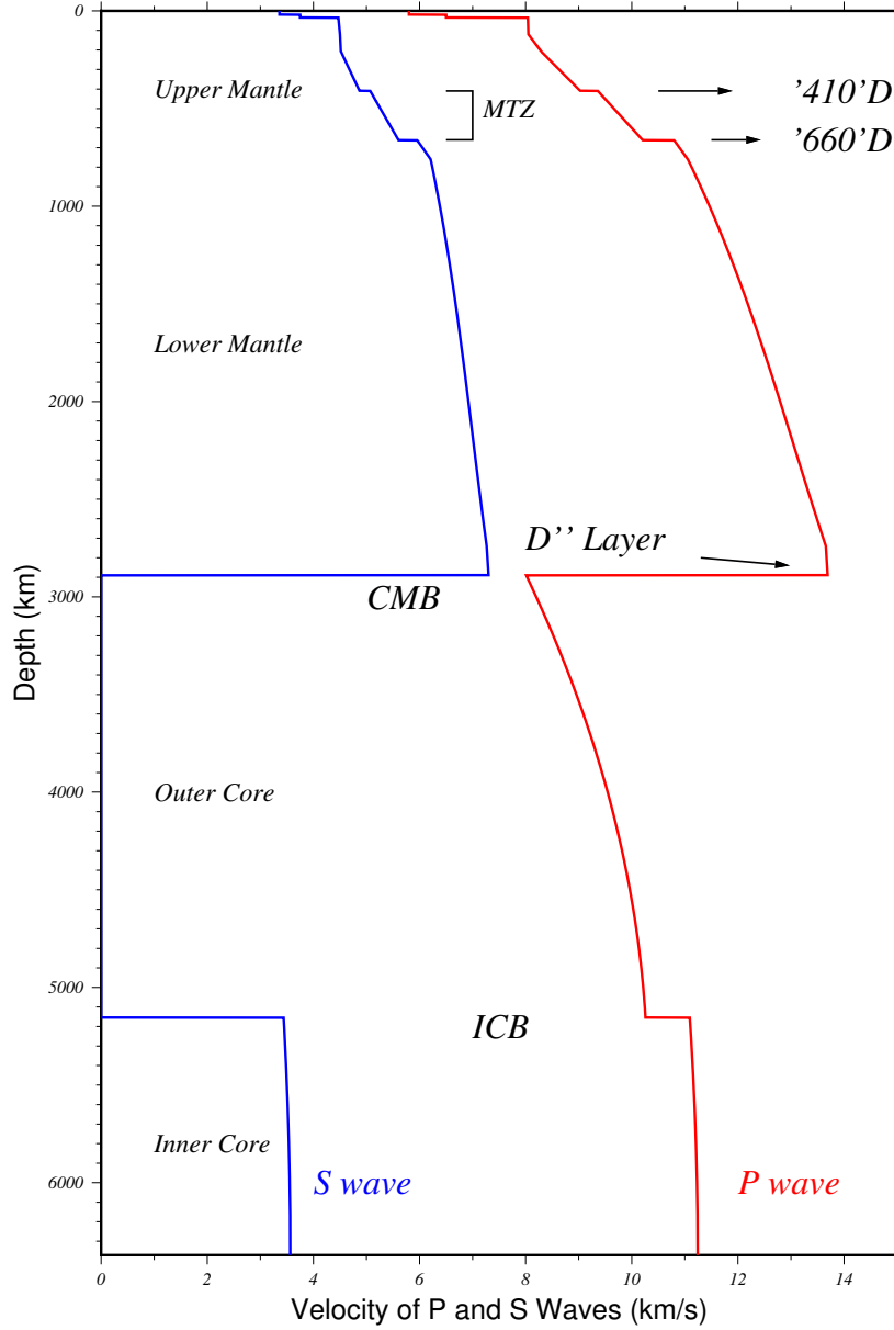
Figure 1: The seismic wave velocity model: IASP91 [Kennett and Engdahl, 1991] shows the two main discontinuities in the upper mantle at the depth of 410 and 660 km which sketch the range of the mantle transition zone (MTZ). As going deeper, the D'' layer with a 1.5 ~ 3 % velocity discontinuities 150~300 km above the CMB.
