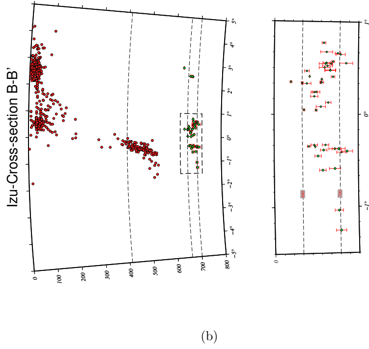
Figure 18: Cross sections with error-bars in Izu-Bonin region.
