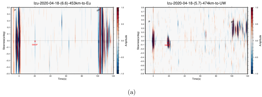
Figure 44: Events which S660P are observed in Izu-Bonin region.(Continued)
