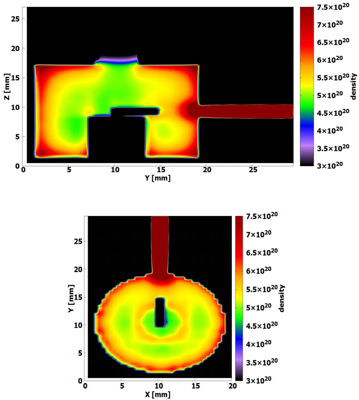
Figure. 2.8: Density Distribution of Neutrals for the One Horizontal Inlet
