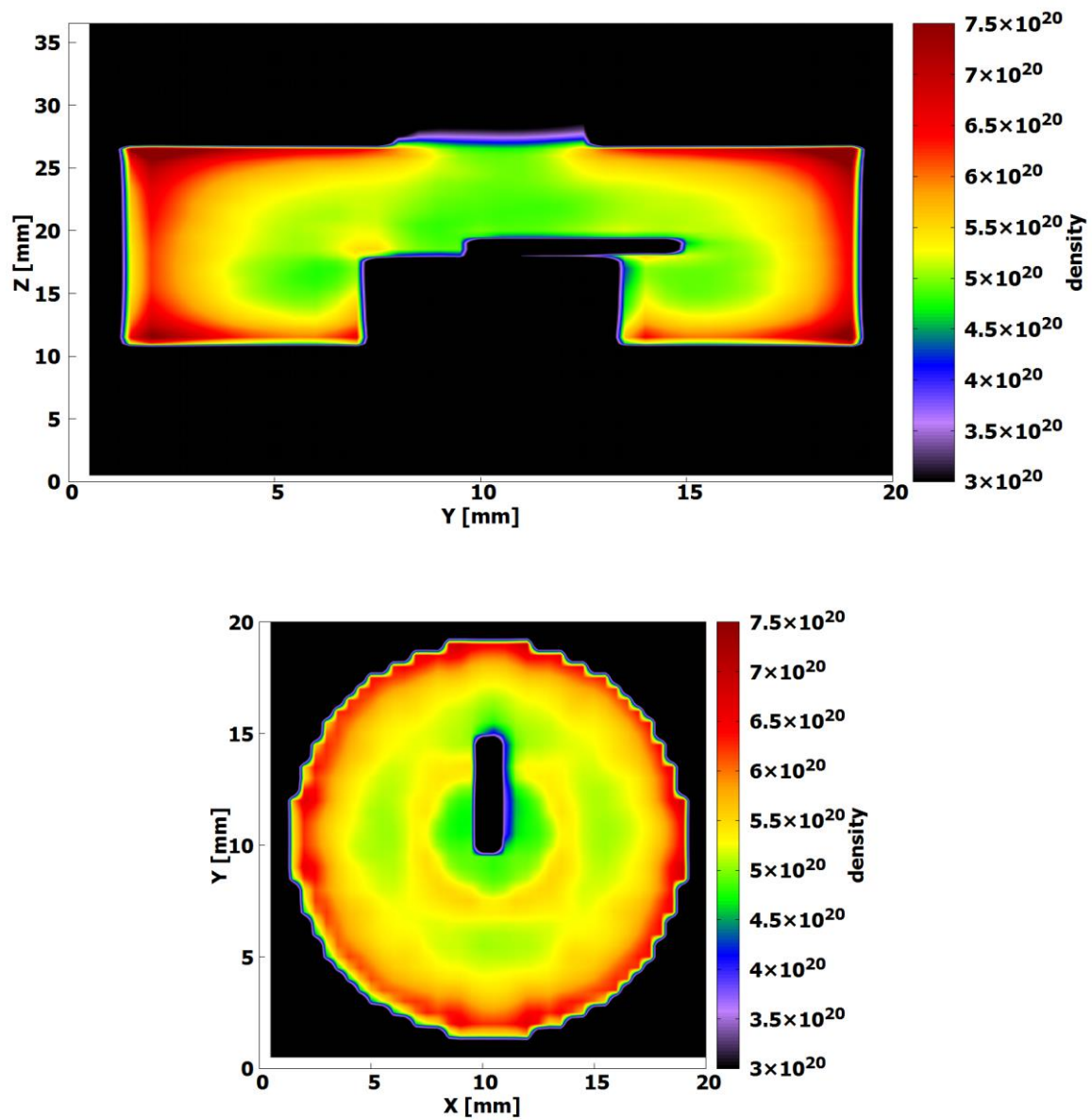
Figure. 2.6: Density Distribution of Neutrals for the 16 Bottom Inlets
