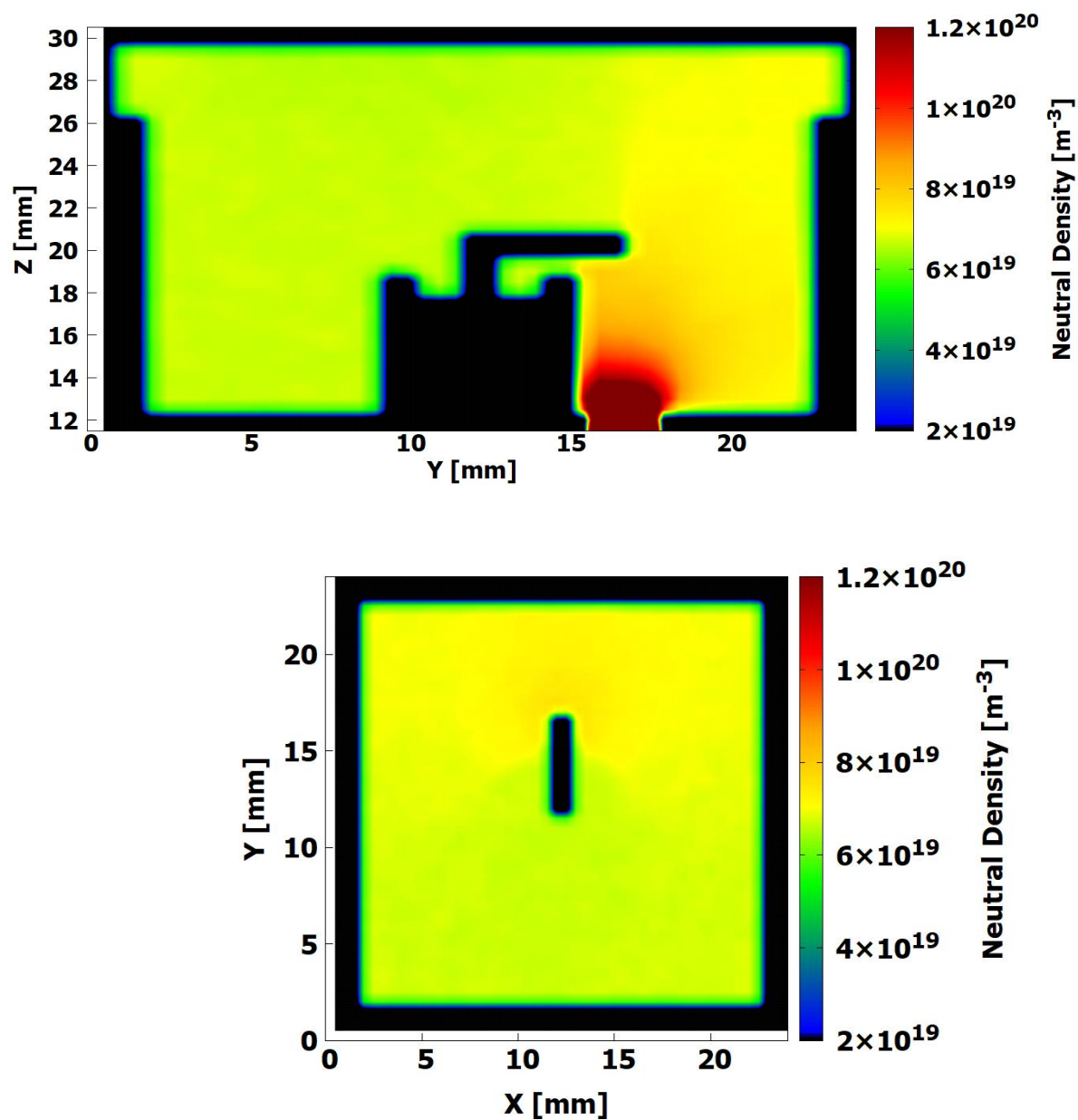
Figure. 4.25: Neutral density distribution for the bottom inlet configuration: (top) Y-Z plane and (bottom) X-Y plane.
