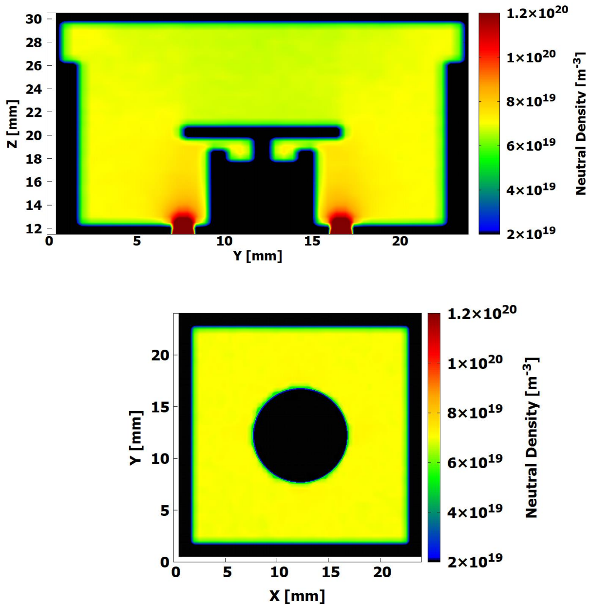
Figure. 4.45: Neutral density distribution for the four bottom inlet configuration: (top) Y-Z plane and (bottom) X-Y plane.
