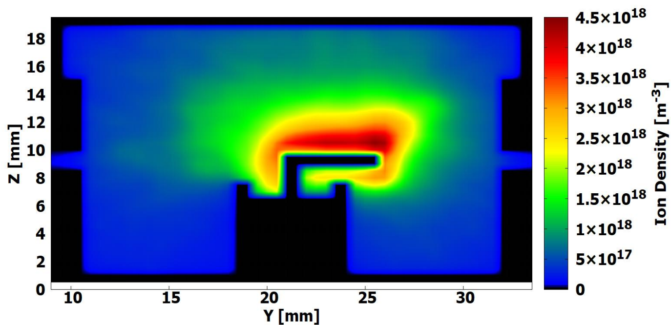
Figure. 4.36: Average Ion Density in the four horizontal inlet configuration
