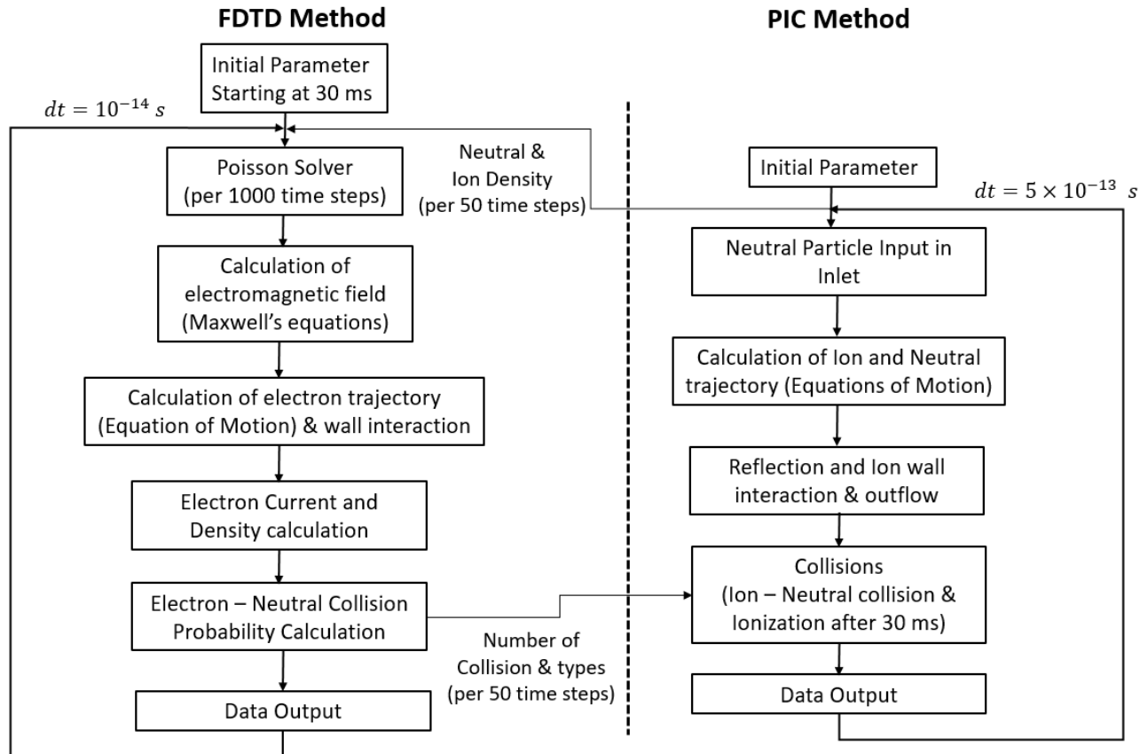
Figure. 4.22: Flowchart of the coupled FDTD-PIC
