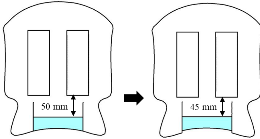
Figure 3-14. A modified model for Type R-1 with h_{s-w} length adjusted (the L_d value is 794 mm)
