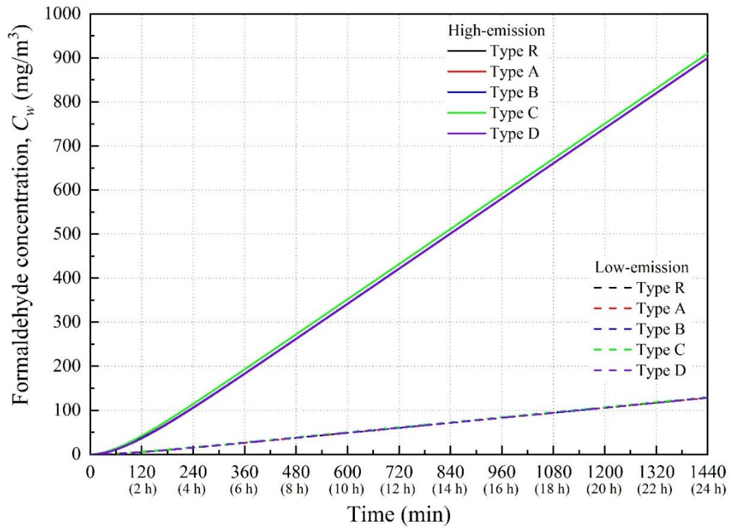
Figure 3-9. Time-series of volume-averaged formaldehyde concentration in the water ( C_w ) for five different desiccators in case of the inner diffusion control type material
