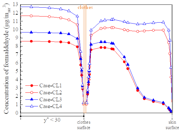
Figure 4-14. The formaldehyde concentration at H1.4 and H1.1: (a) Case-CL and (b) Case-N
