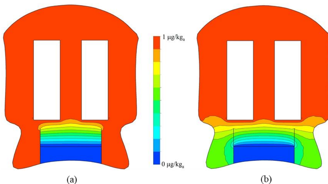
Figure 3-13. Result of the formaldehyde concentration distribution in a modified model without considering for the edge of the crystal dish (Type R): (a) previous model, and (b) modified model
