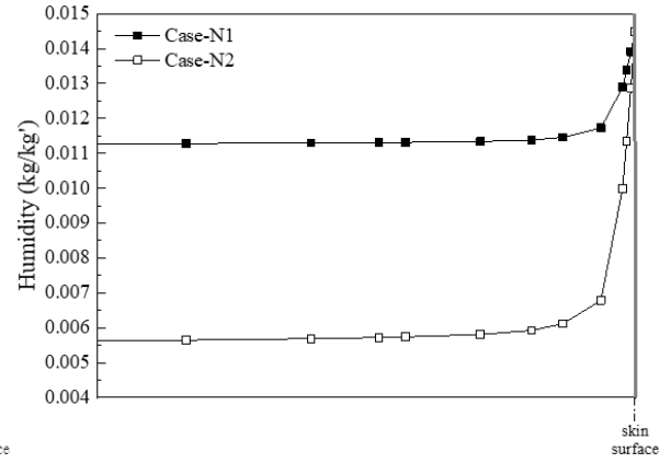
Figure 4-13. The humidity at H1.4 and H1.1: (a) Case-CL and (b) Case-N
