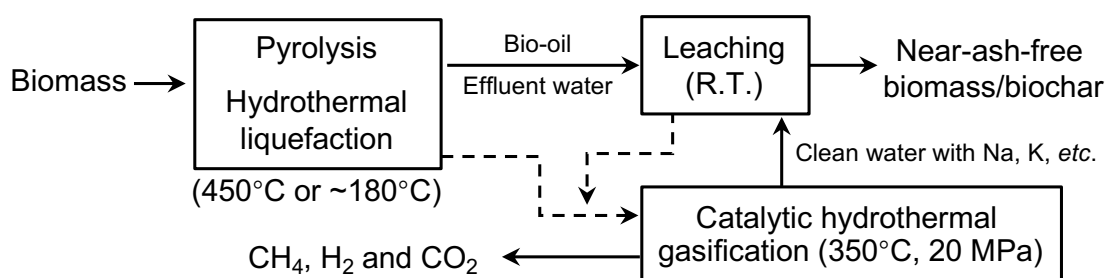
Scheme 3.1. Conceptual diagram for combined leaching and CHTG for conversion of biomass into syngas and clear char.
