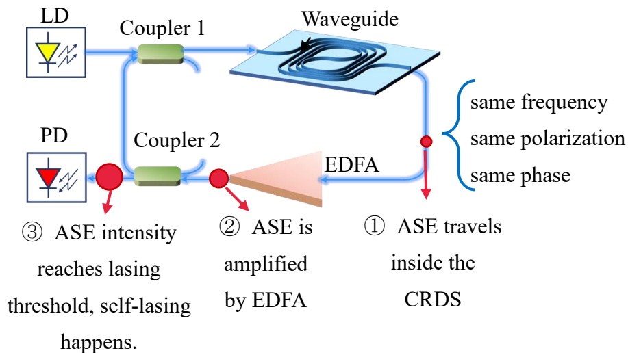
Fig. 3.8 The schematic of self-lasing in amplifier-assisted CRDS. ASE that is generated by EDFA travels inside the CRDS and be amplified by EDFA. When the ASE intensity reaches lasing threshold, self-lasing happens.
