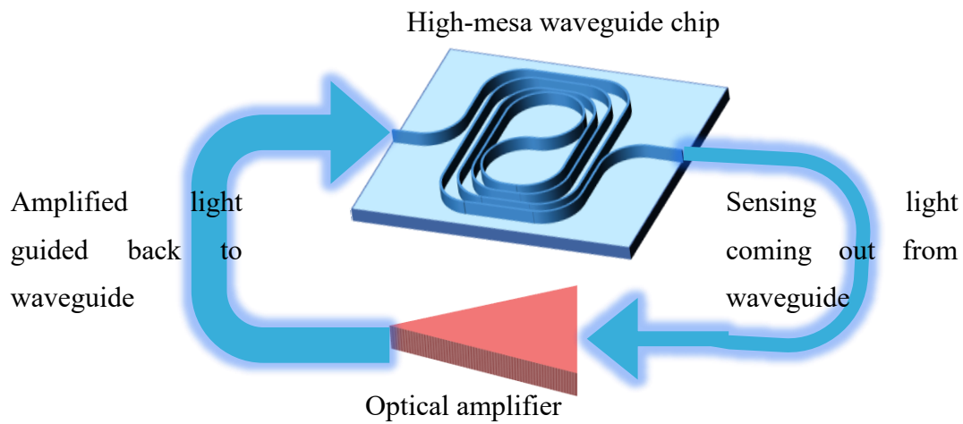
Fig. 2.3 Amplifier-assisted waveguide CRDS schematic configuration. Optical amplifier is used to compensate the waveguide propagation loss. The amplified sensing light is guided back to waveguide for gas absorption.
