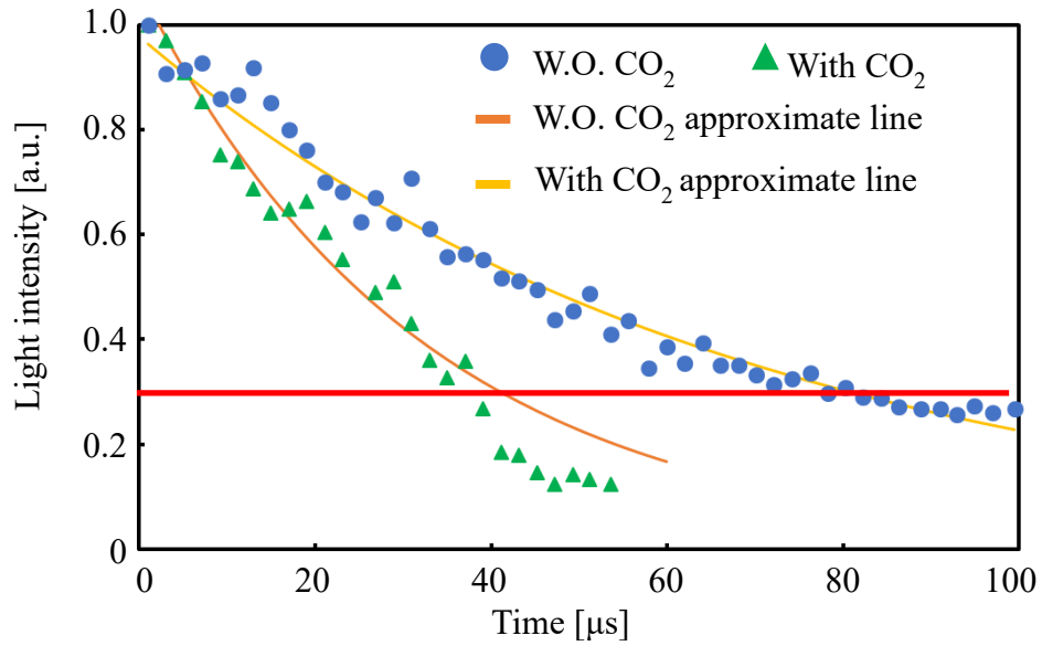
Fig. 4.8 Light intensity peak points and the approximate line of 3% CO 2 sensing result. The cavity ring-down times are estimated as 41 μs and 80.7 μs for “with” and “without” CO 2 condition, respectively.
