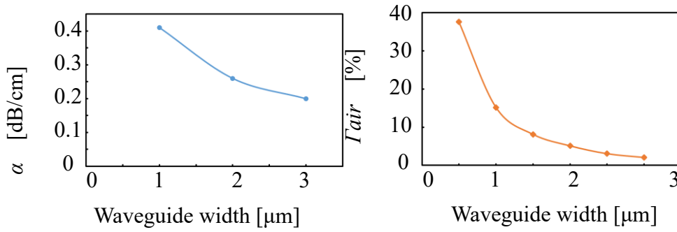
Fig. 1.10 Silicon high-mesa waveguide \alpha and \Gamma_{air} as a function of waveguide width [87, 91]. Silicon high-mesa waveguide has a high \Gamma_{air} as to 37%. Meanwhile, its \alpha is as large as 0.4 dB/cm.
