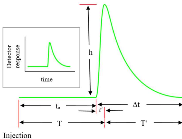
Fig. 1.3 Typical FI Agram for flow injection analysis showing the detector [8]
