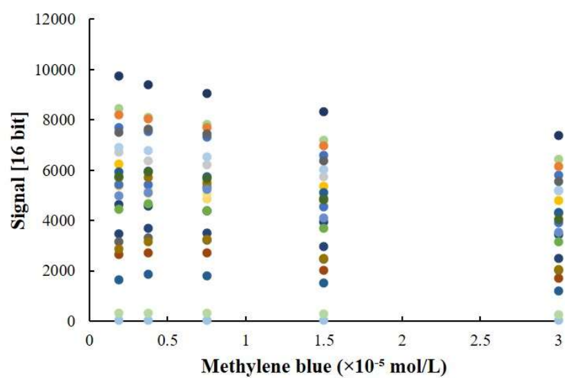
Fig. 3.5 Optical signals for all wells in the 24-well plate investigated by the fabricated compact device
