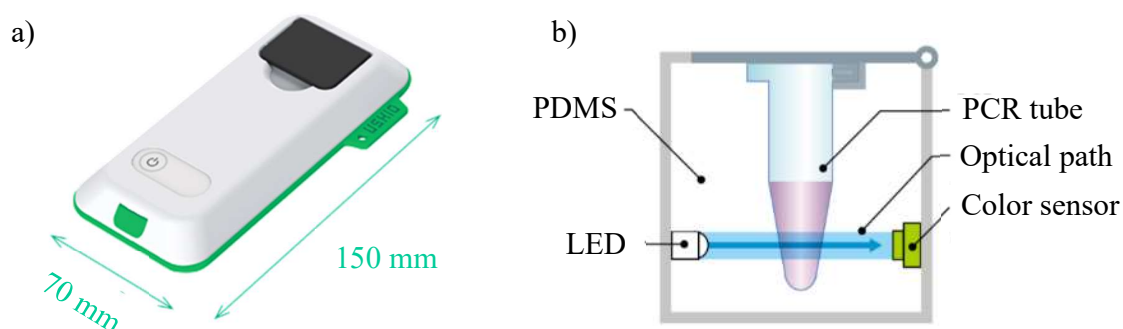
Fig. 2.4 a) Appearance of Ushio picoexplorer™ model PAS-110 absorbance sensor b) Schematic of detector of the Ushio picoexplorer [9].
