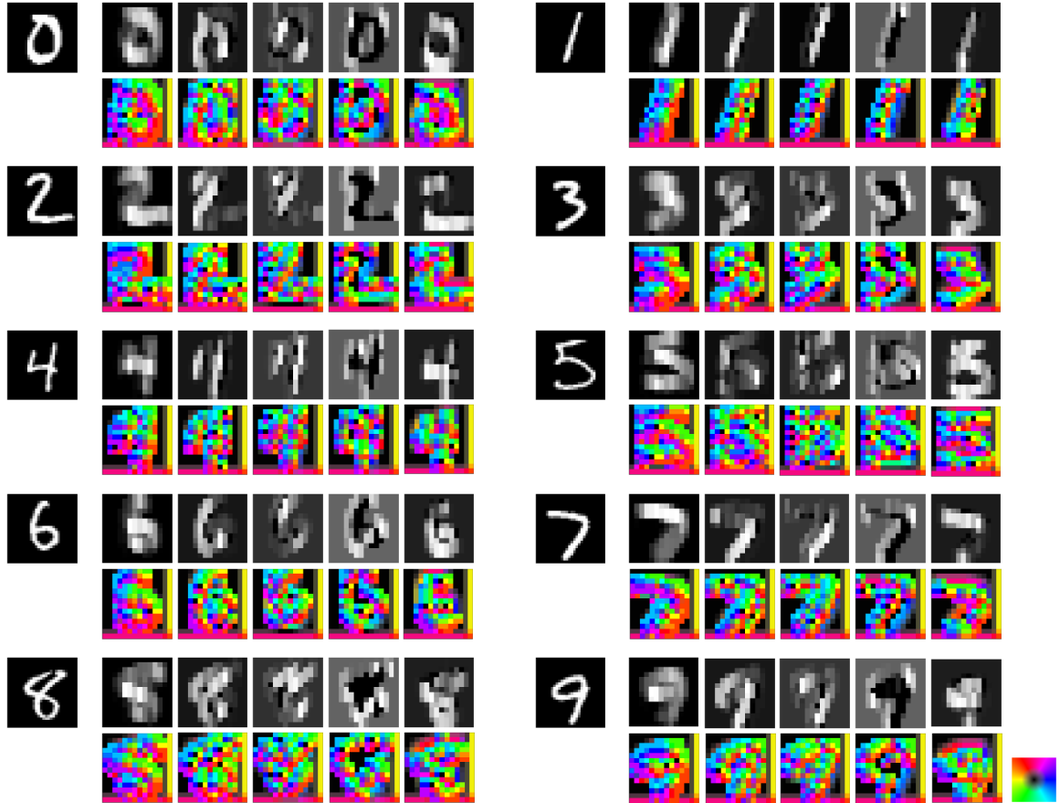
Figure 4-7: Visualization of the displacement features on the different samples that are in the different classes on MNIST dataset. Here, the pooling size is 3 \times 3 . Each column represents one convolutional filter.
