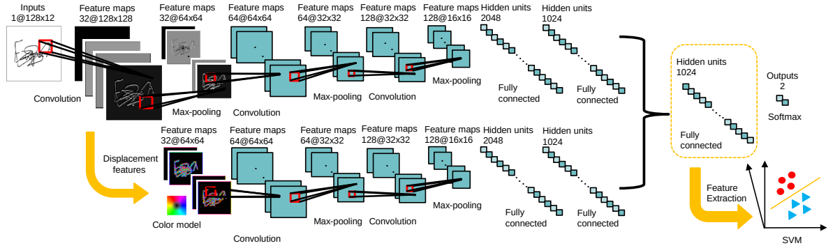
Figure 5-2: The procedure of feature extraction and verification.
