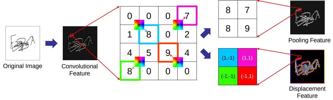
Figure 5-1: Extracting the pooling features and the displacement features simultaneously. Here, the pooling size is 2 \times 2 with stride 2. The displacement features capture micro differences within the pooling window. The displacement vector (-1,1) means that the vertical displacement from the center to the maximum value is -1 and the horizontal displacement is 1.
