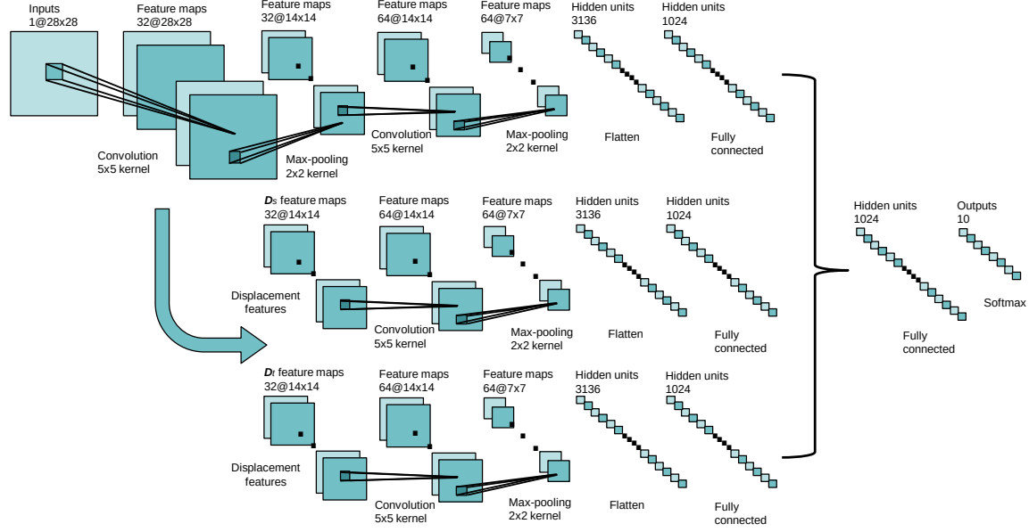
Figure 4-1: The architecture of the proposed method that combining the displacement features and pooling features in a CNN-based architecture. Here, D_s and D_t represent the horizontal and vertical directions of the displacement features.
