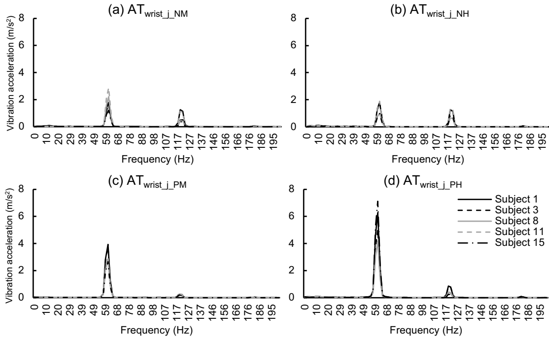
Figure 4.4. Frequency spectra of the total vibration acceleration measured on the wrist.
