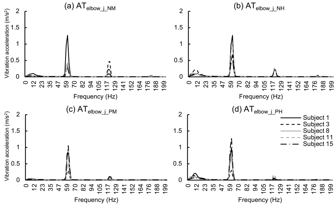
Figure 4.5. Frequency spectra of the total vibration acceleration measured on the elbow.
