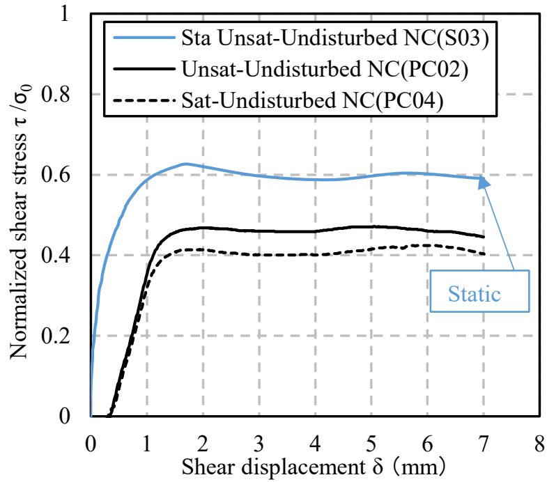
Fig 3.19 Relationship of normalized shear stress and shear displacement of overconsolidated samples (static and post cyclic)
