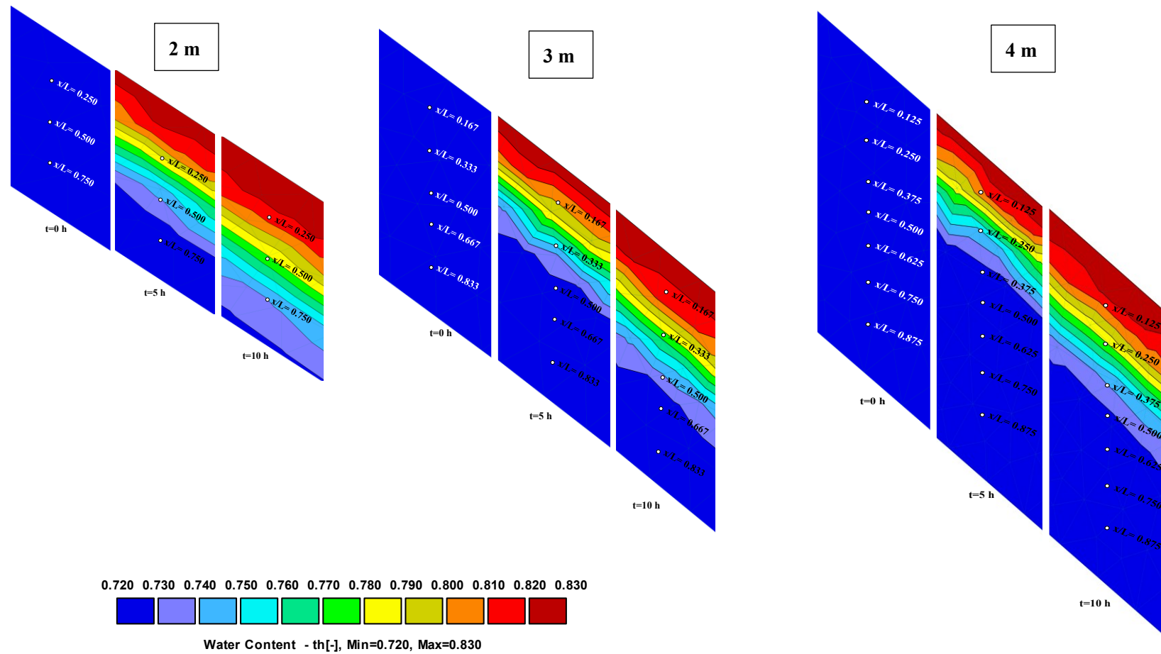
Fig 6.16 The volumetric water content development with time
