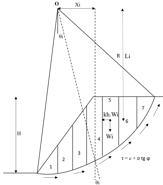
Fig 6.5 The circular slope stability analysis with the seismic intensity.
