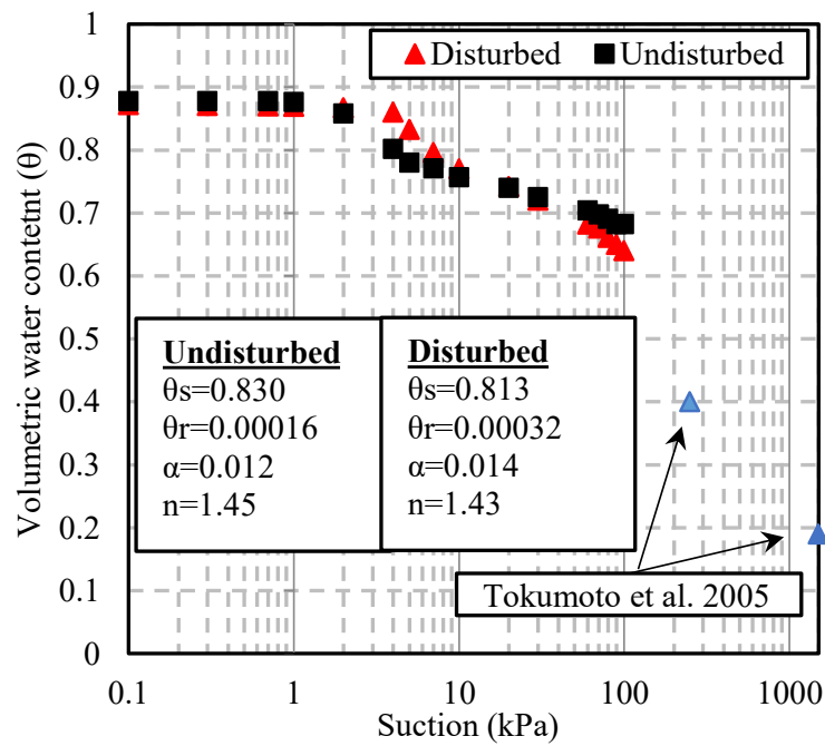
Fig 6.19 SWCC of disturbed and undisturbed samples.
