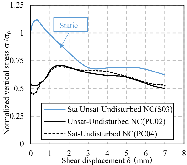
Fig 3.23 Relationship of normalized vertical stress and shear displacement of normally consolidated samples (static and post cyclic)
