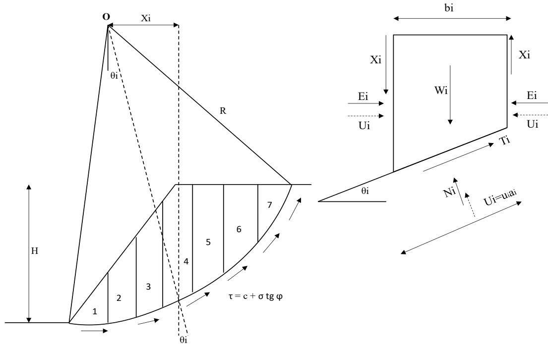
Fig 6.4 The circular slope stability analysis
