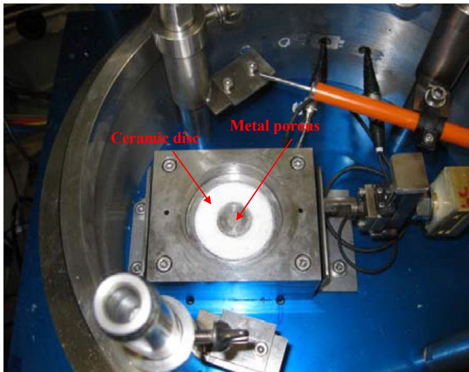
Fig 5.3 Photograph of ceramic disk and metal porous.
