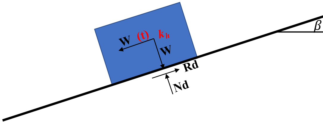
Fig 2.15 Forces acting on a block resting on an inclined plane dynamic condition
