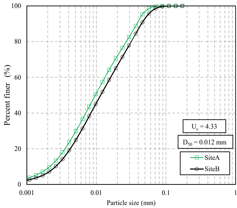
Fig 3.3 Particle size distribution
