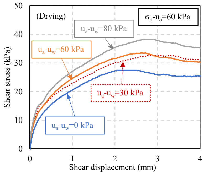
Fig. 5.24 Effects of the suction on (a) shear stress–shear displacement behavior; (b) volumetric behavior (net normal stress 40 kPa)
