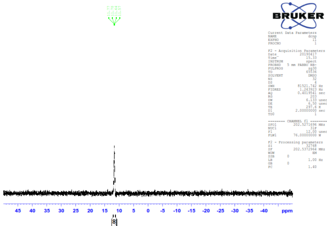
Figure 2.4. ^{31}\text{P} -NMR spectra of DCNP
