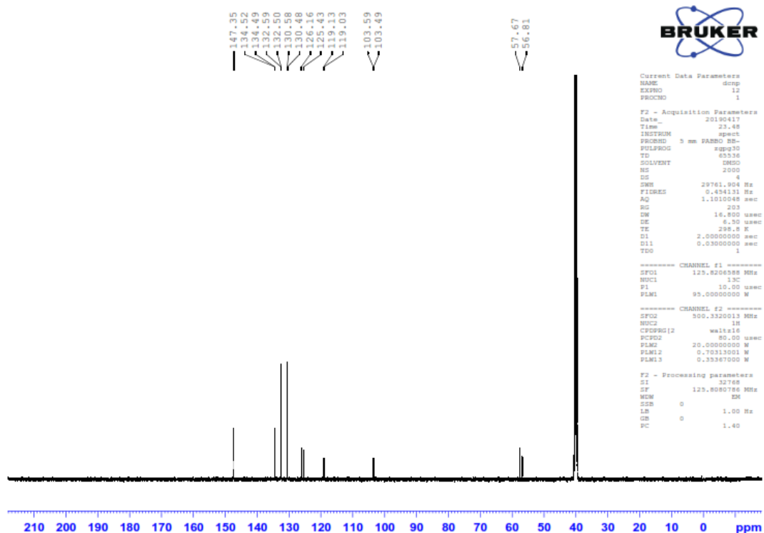
Figure 2.3. ^{13}\text{C} -NMR spectra of DCNP
