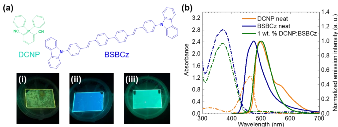
Figure 2.9. (a) Molecular structures of DCNP and BSBCz and photographs of (i) a DCNP neat film, (ii) a BSBCz neat film and, (iii) a 1 wt. %-DCNP-doped BSBCz film (200 nm) fabricated on quartz substrates under UV light irradiation ( \lambda_{\text{ex}} = 356 nm). DCNP easily crystallized in neat films [see (i) in (a)]. However, this crystallization was suppressed by doping DCNP into BSBCz [see (iii) in (a)] because BSBCz forms stable amorphous films without crystallization [see (ii) in (a)]. (b) Absorbance and normalized emission spectra of these samples. The excitation wavelength used for the PL measurement was \lambda_{\text{ex}} = 337 nm.
