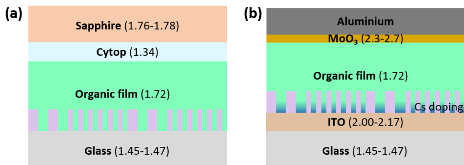
Appendix Figure 3. Schematic representation of refractive index of each layer for my DFB laser devices, (a) device for optical pumping (b) device for current injection OSLED.
