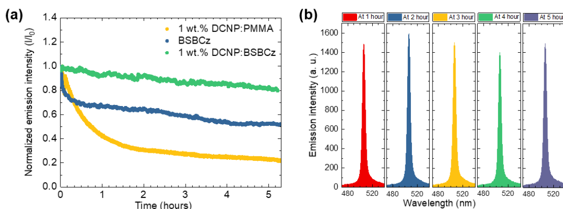
Figure 2.20. ASE decay profile measured in nitrogen at room temperature ( \lambda_{\text{ex}} = 337 nm). (a) Normalized emission intensity versus time, (b) Respective emission spectra with time for 1 wt.-%-DCNP:BSBCz film.
