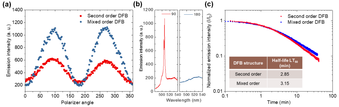
Figure 2.30. Optically pumped lasing under true-CW excitation ( \lambda_{ex} = 355 nm); polarization of output laser beam (excitation intensity = 3536 \text{ W cm}^{-2} ); (a) emission intensity as a function of polarization angle (b) respective emission spectra. Optical stability; (c) intensity/initial intensity versus operation-time (d-inset) table of estimated half-life.
