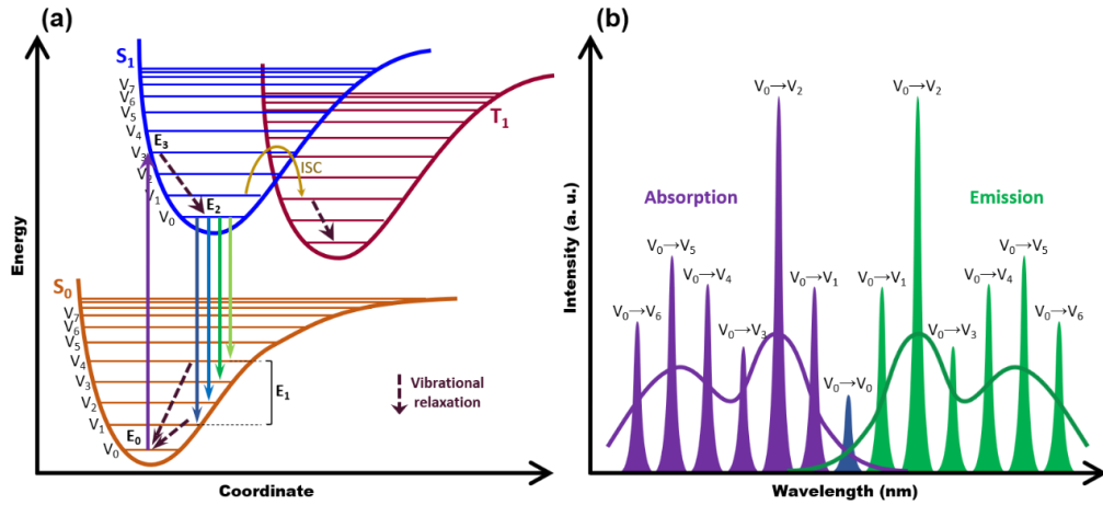
Figure 1.3. (a) Frank-Condon energy level diagram of a four-level organic fluorescent laser gain material. (b) Respective absorption and emission spectra showing vibrational peaks [16] .
