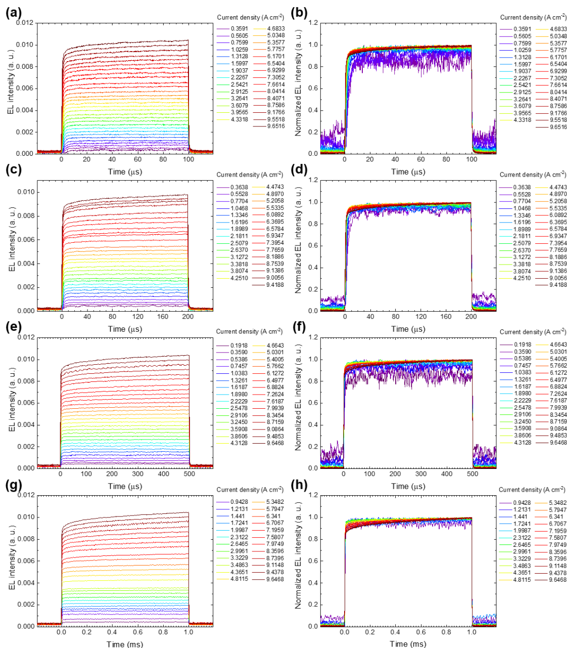
Figure 3.7. Transient EL responses of OLEDs with the BSBCz host layer. Temporal profiles of EL intensity when the pulse widths were (a,b) 100 \mu\text{s} , (c,d) 200 \mu\text{s} , (e,f) 500 \mu\text{s} , (g,h) 1 \text{ ms} . The EL intensities of (a,c,e and g) were normalized in (b,d,f and h) respectively to make it easy to see the response shapes.
