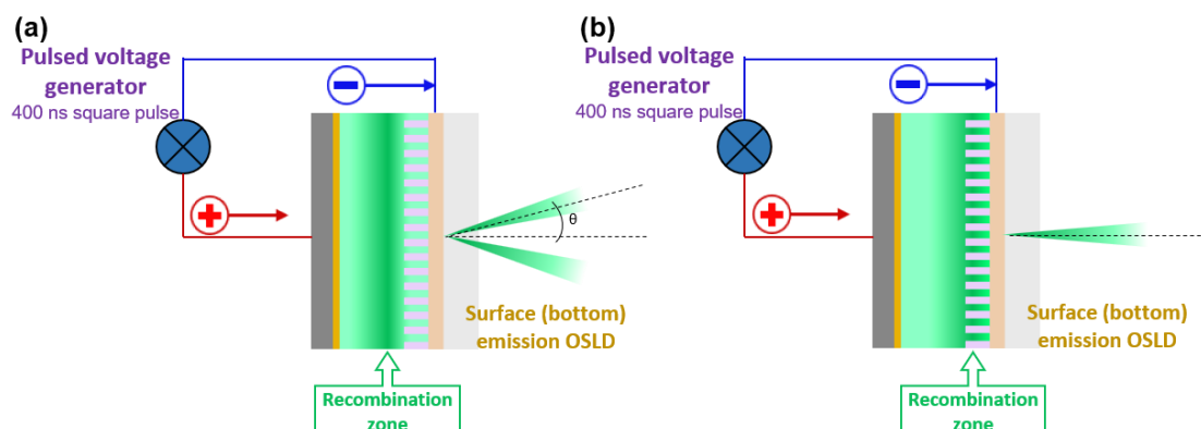
Figure 4.3. Proposed model of shifting charge recombination zone for stimulated emission enhancement.
