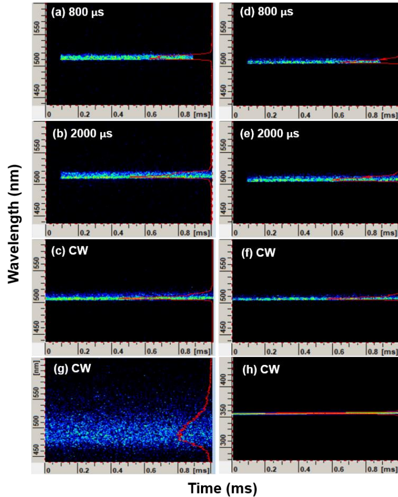
Figure 2.31. Streak camera images of long-pulsed (quasi-CW) and true-CW excitation ( \lambda_{ex} = 355 nm, excitation intensity = 3536 \text{ W cm}^{-2} ); second-order DFB (a) at 800 \mu\text{s} (b) at 2000 \mu\text{s} (c) at true CW, mixed-order DFB (d) at 800 \mu\text{s} (e) at 2000 \mu\text{s} (f) at true-CW, (g) outside of DFB at true CW and (h) excitation laser of true CW.
