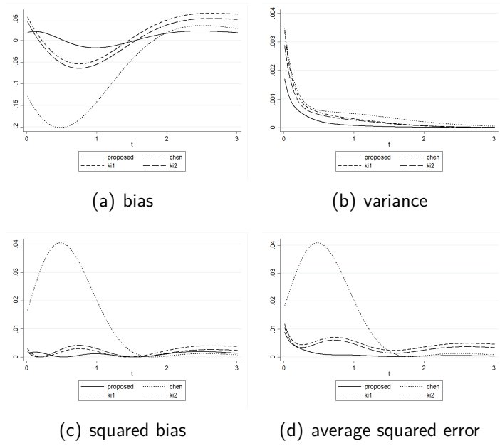
Figure 2.3: Comparison of the point-wise bias, variance, and ASE of \tilde{f}_X(x) , \hat{f}_C(x) , \hat{f}_{K11}(x) , and \hat{f}_{K12}(x) for estimating density of abs.N(0,1) with sample size 150.
