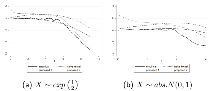
Figure 5.2: Simulated bias comparisons of m_n(t) , \widehat{m}_X(t) , \widetilde{m}_{X,1}(t) , and \widetilde{m}_{X,2}(t) for several distributions, with sample size n = 50 and 500 repetitions.
