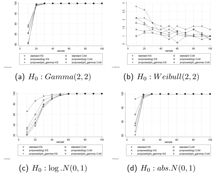
Figure 4.3: Simulated percentage (%) of rejecting null hypothesis when the samples were drawn from \text{Weibull}(2, 2) .
