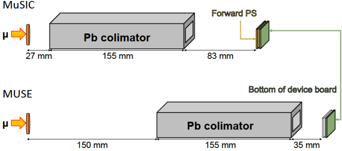
Figure 4.1: Comparison of the experimental setup at MuSIC and MUSE. There are three differences between them; the shape of the muon beam (Gaussian-distribution of \sigma_x = \sigma_y = 21 mm at MuSIC and square of x = y = 10 mm at MUSE), distance among the beam exit, collimator and device board and whether the forward PS was used or not. In PHITS simulation, the momentum distribution in the bottom of the device board at MuSIC and MUSE was calculated.
