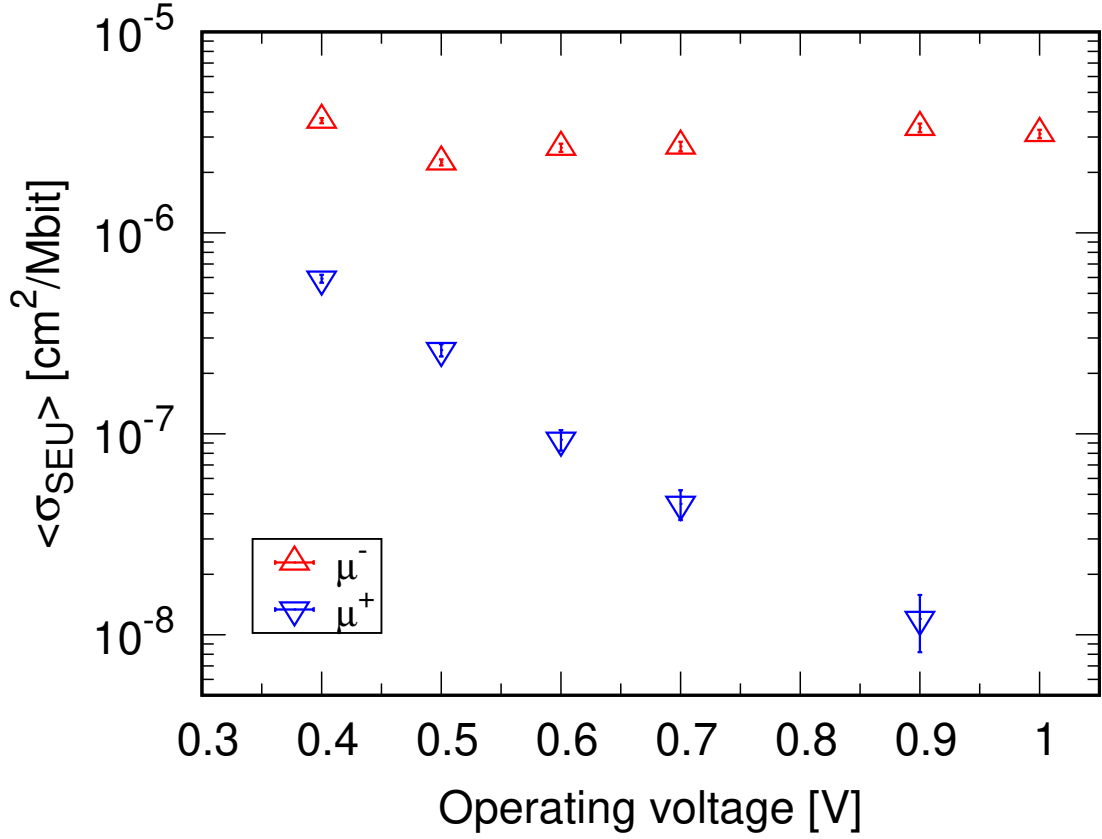
Figure 1.9: Operating voltage dependence of muon-induced SEU cross sections obtained at MUSE [15], [17]. The mean momentum of muons is 36.5 MeV/c.
