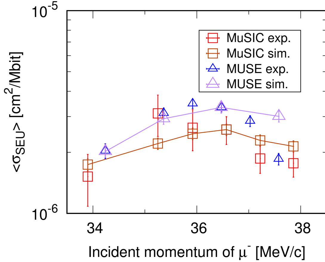
Figure 5.2: Comparison of the SEU cross sections simulated by PHITS with the experimental result obtained in the present work at MuSIC and previous work at MUSE.
