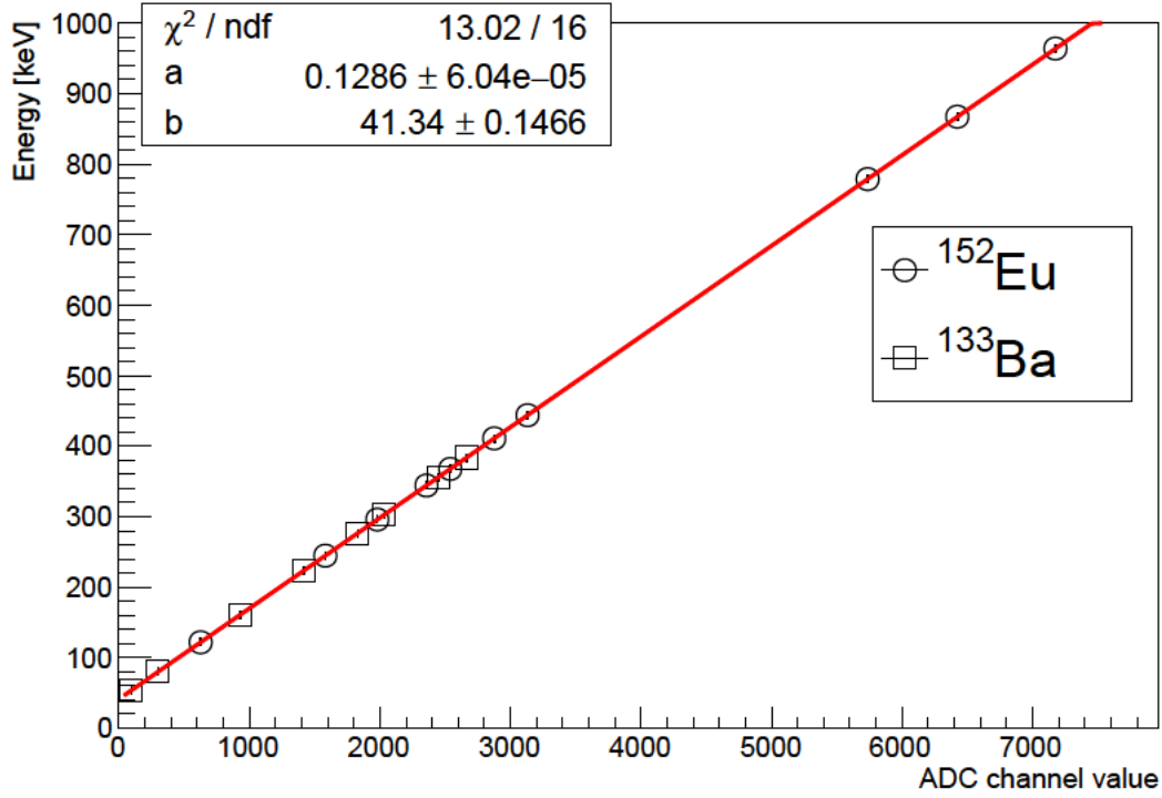
Figure 3.5: Energy calibration line for Ge detector with points which represent the energy and ADC channel value of \gamma -rays from the standard sources, ^{152}\text{Eu} and ^{133}\text{Ba} .
