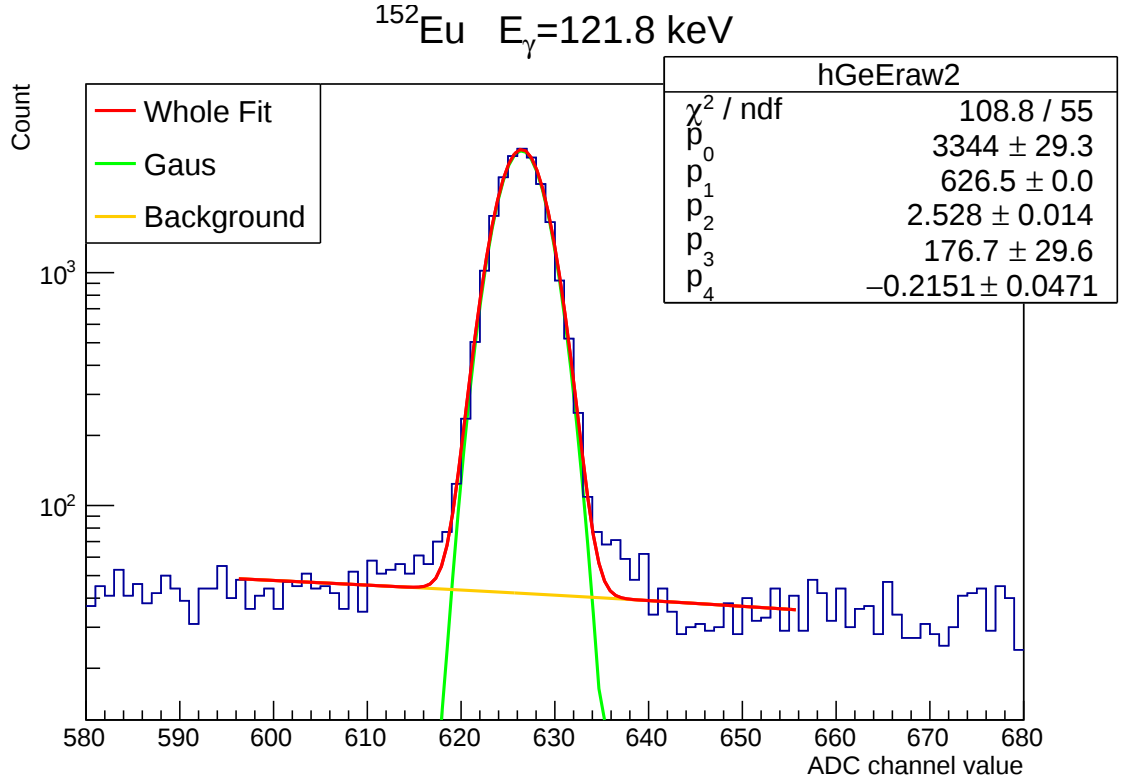
Figure 3.4: An example of fitting for \gamma -ray with energy 121.8 keV from ^{152}\text{Eu} . The red line (Whole Fit) represents the fitting result according to Eq. (3.5). The green (Gaus) and yellow (Background) ones represent the Gaussian and linear part in Eq. (3.5), respectively.
