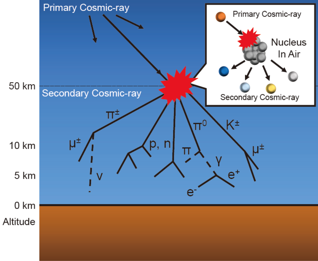
Figure 1.4: Generation process of secondary cosmic-rays.
