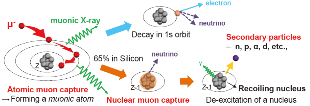
Figure 1.6: Schematic illustration of the negative muon capture process.
