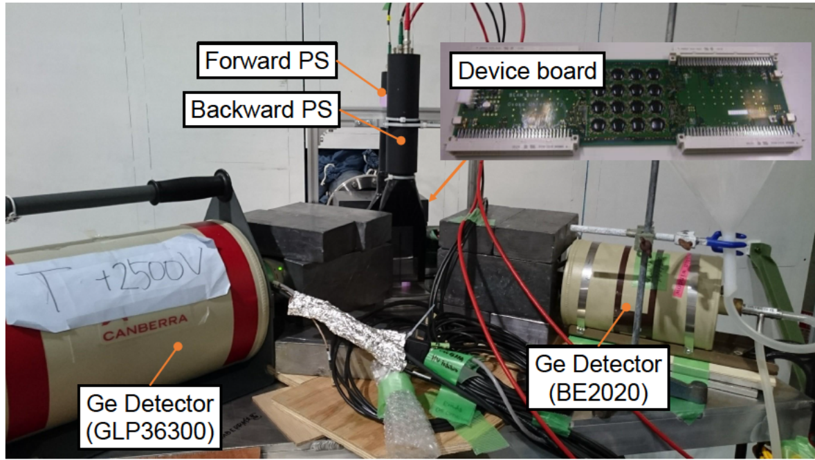
Figure 2.4: A photograph of the experimental setup from downstream.
