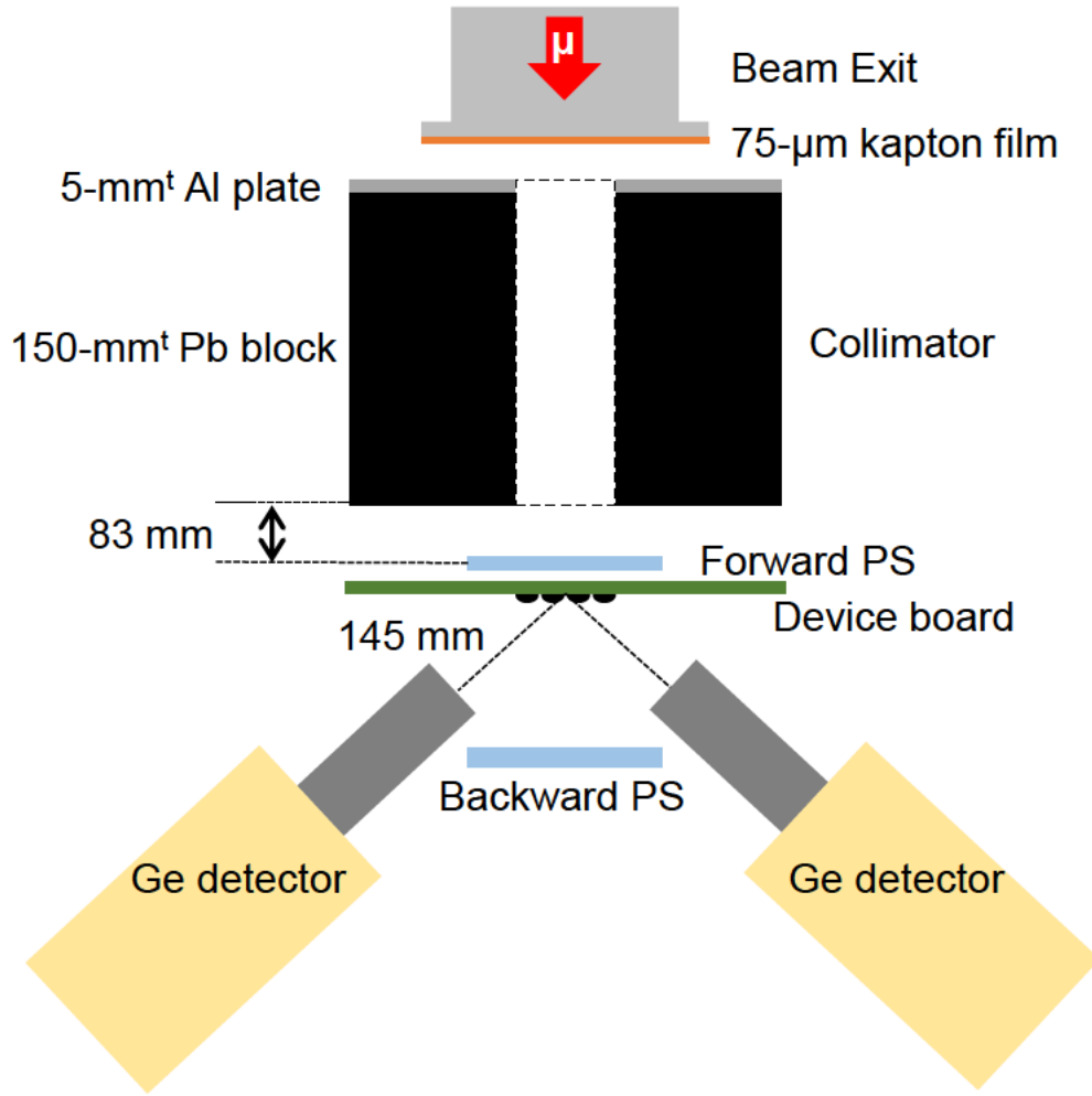
Figure 2.5: Configuration of muon irradiation and arrangement of detectors.
