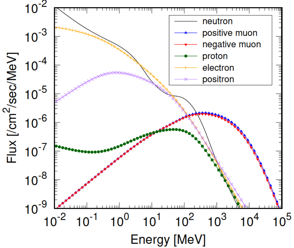
Figure 1.5: Energy spectra of secondary cosmic-rays at ground level calculated by EXPACS ver. 3.03. This figure shows the energy-spectra at Fukuoka, Japan.
