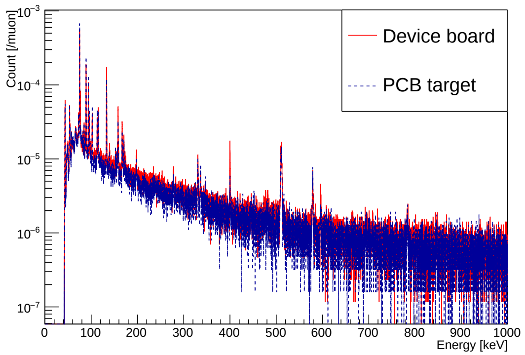
Figure 3.8: Comparison of energy spectra of muonic X-rays from device board and PCB target.
