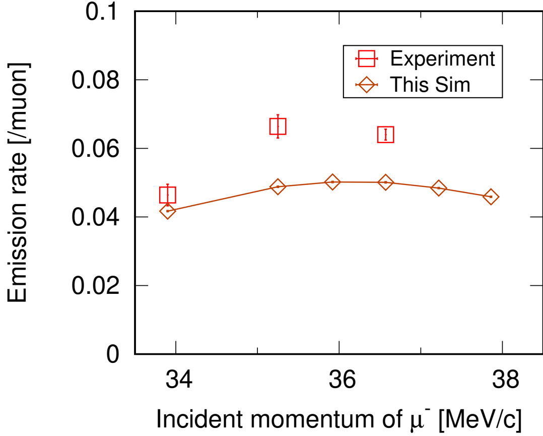
Figure 5.3: Comparison of the emission rate of muonic X-rays from chip part simulated by PHITS with the experimental result obtained in the present work at MuSIC.
