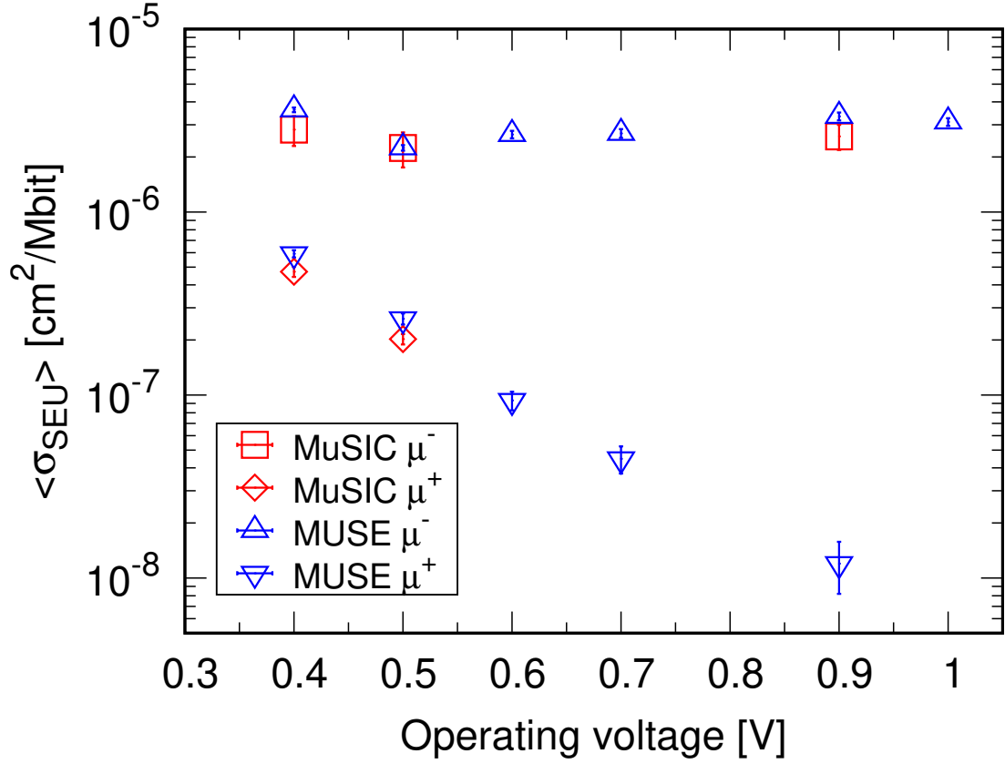
Figure 4.5: Comparison of the operating voltage dependence of the negative and positive muon-induced SEU cross sections measured at MuSIC and MUSE. The data at MUSE was obtained from [15], [17]. The means of momentum of muons are 36.6 MeV/c at MuSIC and 36.5 MeV/c.
