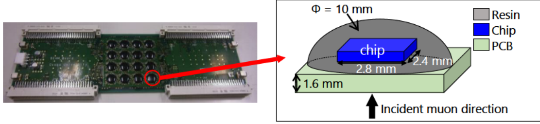
Figure 2.3: Structure of the test device board. 16 chips on the 1.6-mm-thick PCB. The thickness of tested chips approximately 0.34 mm.
