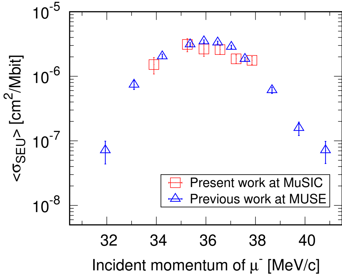
Figure 4.4: Comparison of the incident momentum dependence of the negative muon-induced SEU cross sections measured at MuSIC and MUSE. The data at MUSE was obtained from [14], [15]. The SRAM chips were operated at the voltage of 0.9 V.
