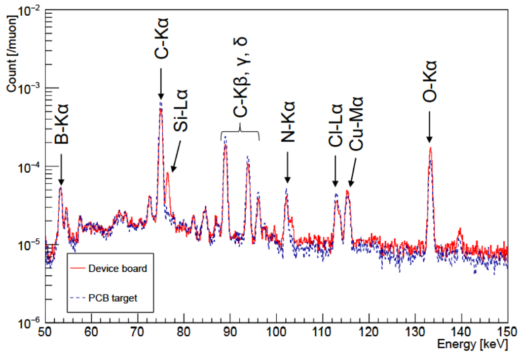
Figure 3.9: Comparison of energy spectra of muonic X-rays from device board and PCB target in the range of 50 keV~150 keV.
