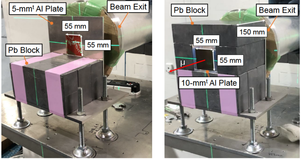
Figure 2.6: Photographs of the beam collimator.
