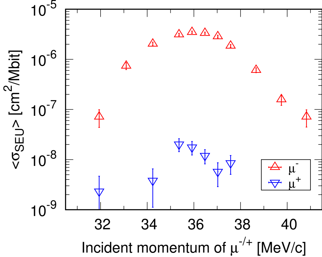
Figure 1.8: Incident momentum dependence of muon-induced SEU cross sections obtained at MUSE [15], [17]. The SRAM chips were operated at the voltage of 0.9 V. The negative muon-induced SEU cross sections are about 100 times larger than the positive muon-induced ones.
