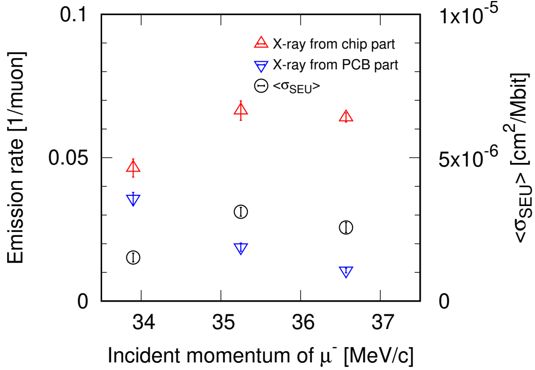
Figure 4.6: The relationship between the emission rate of muonic X-rays from chips or resin and the negative muon SEU cross section. The SEU cross section was measured for the 65-nm bulk SRAMs at the operating voltage of 0.9 V.
