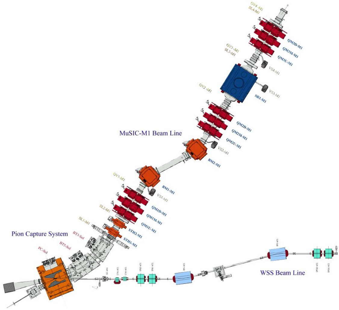
Figure 2.2: Schematic view of MuSIC-M1 beam line. WSS Beam Line mentions a beam line of protons. The figure is obtained from Figure 1 in [30]
