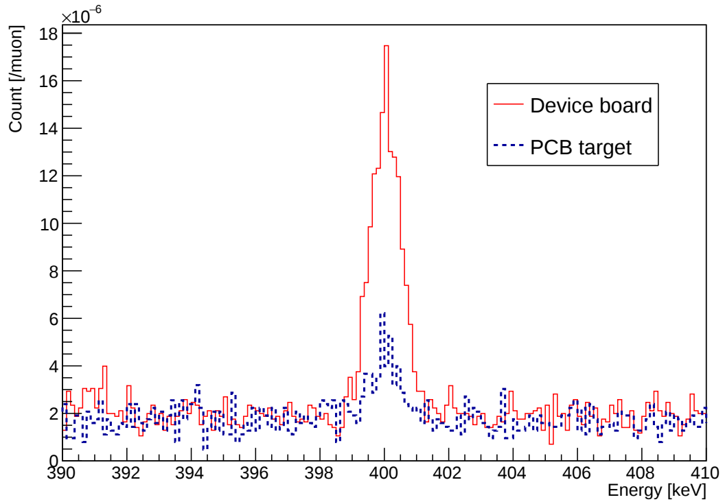
Figure 3.10: The energy spectra of muonic X-rays emitted from the device board (red solid line) or the PCB alone (blue dot line). The incident muon incident momentum is 38.9 MeV/c at beam exit. The energy of silicon K\alpha muonic X-ray is about 400 keV.
