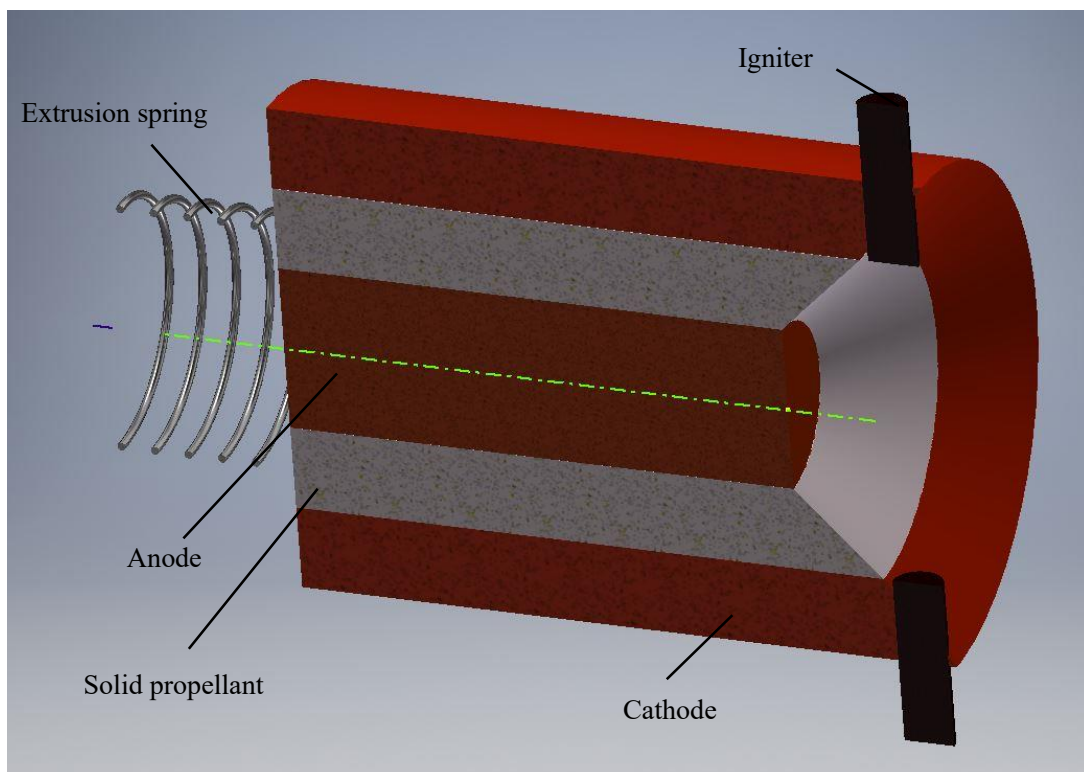
Figure 1.3. Coaxial type PPT
