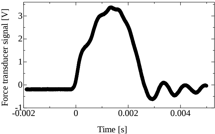
Figure 2.9. Example of calibration data of force
