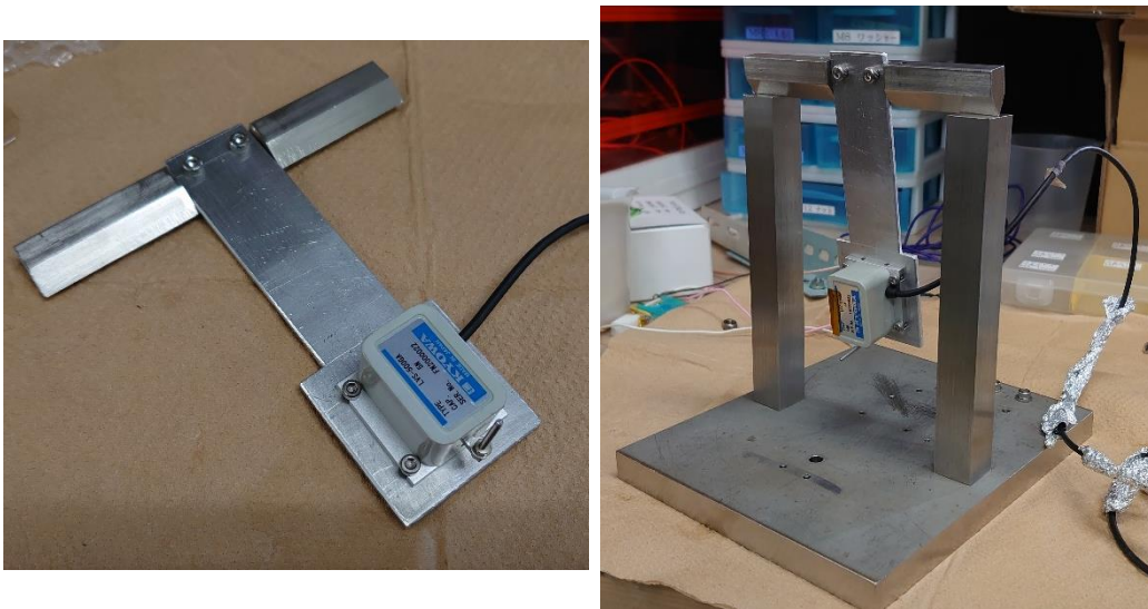
Figure 2.8. Pendulum type Calibration hammer
