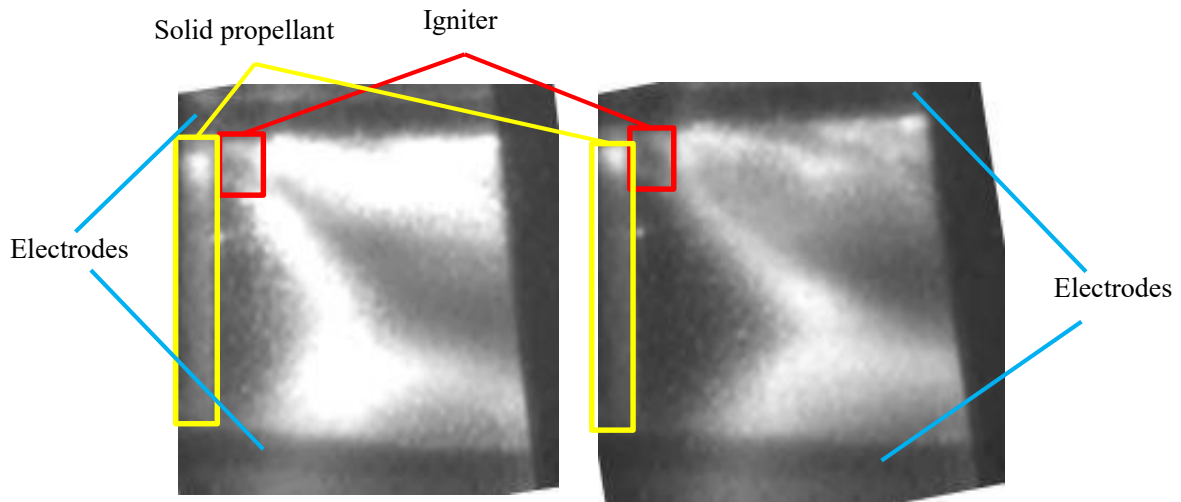
Figure 3.12. Plasma movement for 2 \mu\text{s} taken with a high-speed camera at 500 V in normal shape solid propellant
