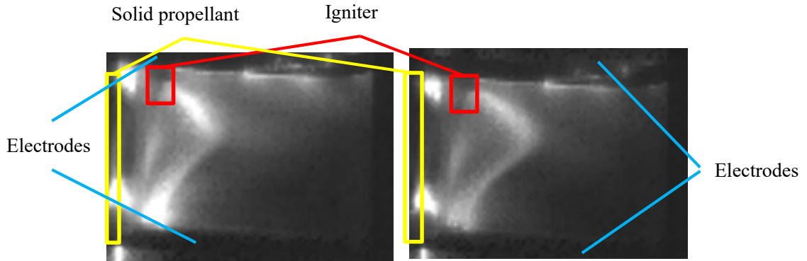
Figure 3.17. Plasma movement for 2 \mu\text{s} taken with a high-speed camera at 500 V in perforated solid propellant
