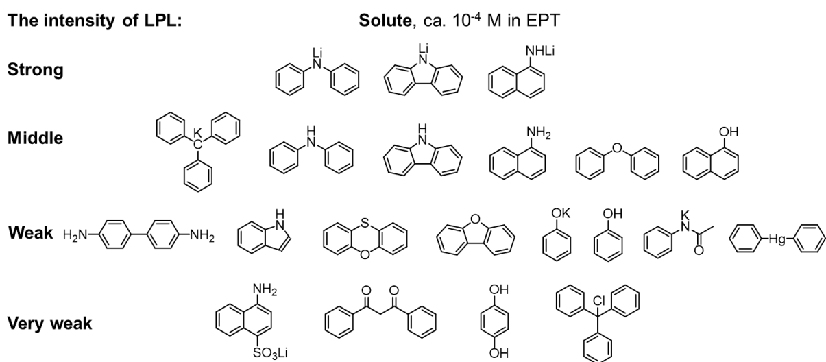
Figure 1-9. Structures of organic molecules as solute investigated by Linschitz and Berry as well as rough results of LPL performance. The solvent EPT is a mixture of ether, isopentane, triethylamine, 2:3:3 or 5:5:2. 82
