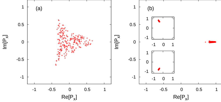
Figure 2.9: Scatter plot of P_x at (a) \kappa = 0 and (b) \kappa = 0.5 in one configuration. We set N_s = 6 . Two small windows in the right panel show the scatter plot in other configurations.
