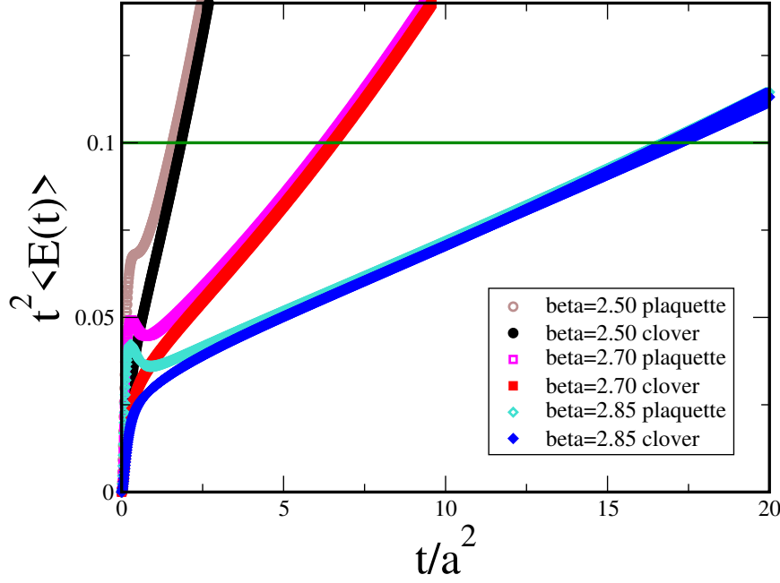
Figure 3.2: t/a^2 -dependence of t^2 \langle E(t) \rangle with both the plaquette and clover-leaf definitions at \beta = 2.500, 2.700 and 2.850 . The open symbols represents the results with the plaquette definition, and the filled ones denotes the results with the clover-leaf definition.
