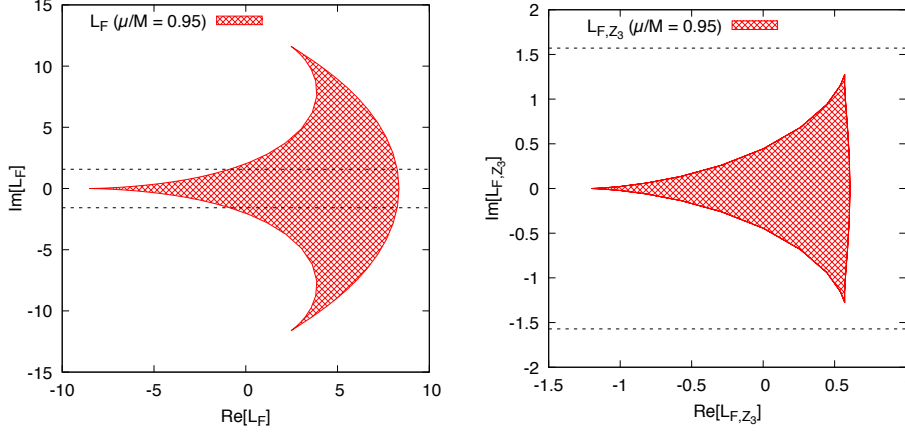
Figure 2.7: (left) \text{Re}[L_F] – \text{Im}[L_F] or (right) \text{Re}[L_{F,Z_3}] – \text{Im}[L_{F,Z_3}] relation in the case of N_f = 3 . We set M/T = 10 and \mu/M = 0.95 . The two dashed lines are drawn at \pm\pi/2 , respectively.
