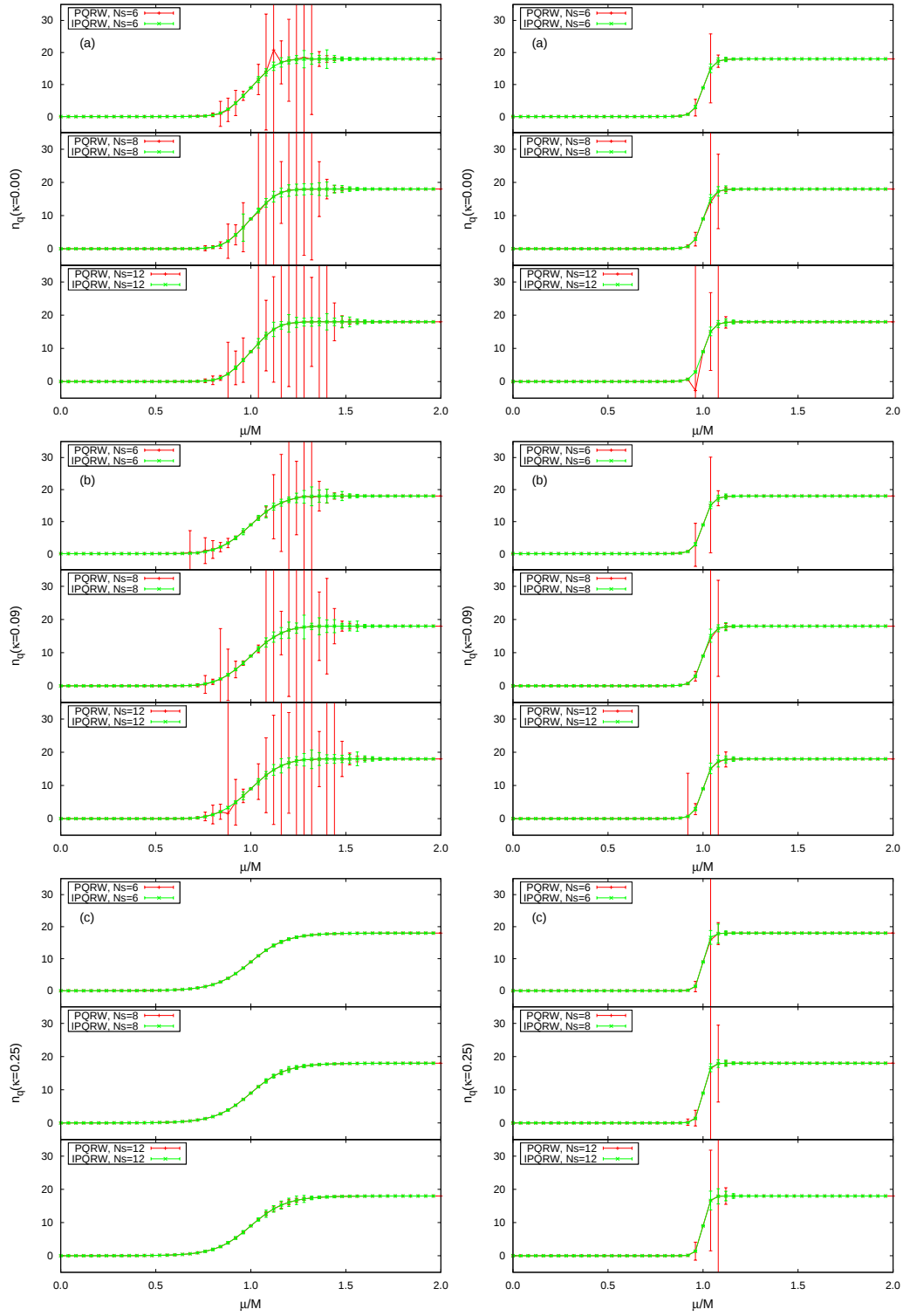
Figure 2.14: \mu - and N_s -dependence of n_q in (left) EPLMWO and (right) \mathbb{Z}_3 -EPLM with both PQRW and IPQRW. In all panels, red (green) symbols denote the results obtained with PQRW (IPQRW). (a) \kappa = 0.0 , (b) \kappa = 0.09 , and (c) \kappa = 0.25 .
