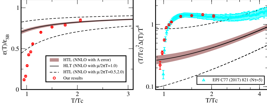
Figure 3.10: Comparison with the prediction of the HTL model. For the HTL model, we use the NNLO notation in the 2-color case shown in Ref. [34]. The left panel shows the result of the entropy density rescaled by that in the SB limit, while the right panel does the results of the rescaled trace anomaly. In both the panel, the solid line shows the result of HTL model with the renormalization scheme \mu_{\text{HTL}}/(2\pi T) = 1.0 , while the upper (lower) dashed line does that with \mu_{\text{HTL}}/(2\pi T) = 1.5 (0.5), respectively. The band also represents the systematic uncertainty from T_c/\Lambda_{\overline{\text{MS}}} = 1.23(11) . In the right panel, we also plot the result obtained in Ref. [68] as the triangle symbol.
