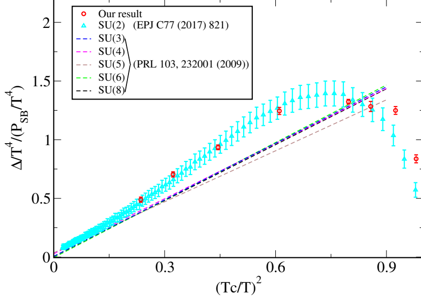
Figure 3.11: N_c -dependence of the rescaled trace anomaly (\Delta/T^4)/(P_{SB}/T^4) . The circle and triangle symbols denote our data and the results obtained in Ref. [68], respectively. The several dashed lines show the well-fitted linear functions for pure SU(3 \leq N_c \leq 8) gauge theories shown in Ref. [48].
