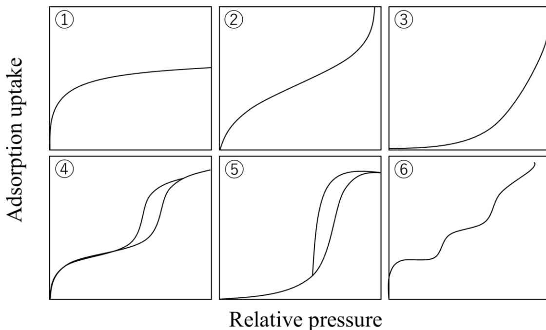
Fig. 2-1 The IUPAC classification of adsorption isotherm for solid/gas euqilibrium
