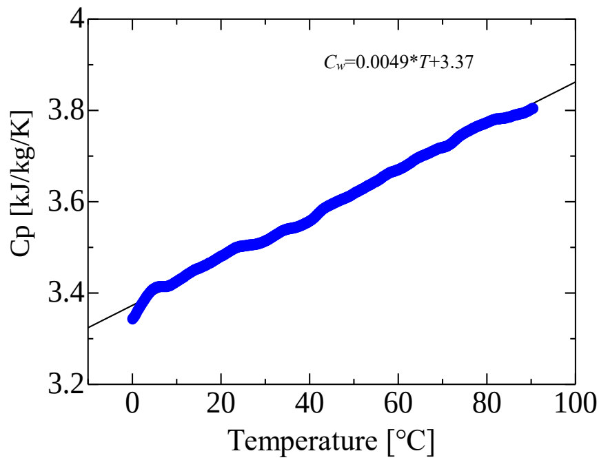
Fig. A-3 Specific heat of LLC
