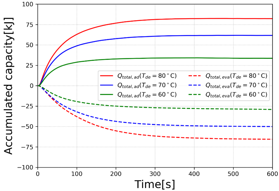
Fig. 3-9 Accumulated heat output profiles for various regeneration temperature where the adsorption and condensation temperature are set at 30°C, evaporation temperature is 15°C and flow rate of the heat transfer medium is set at 3LPM.
