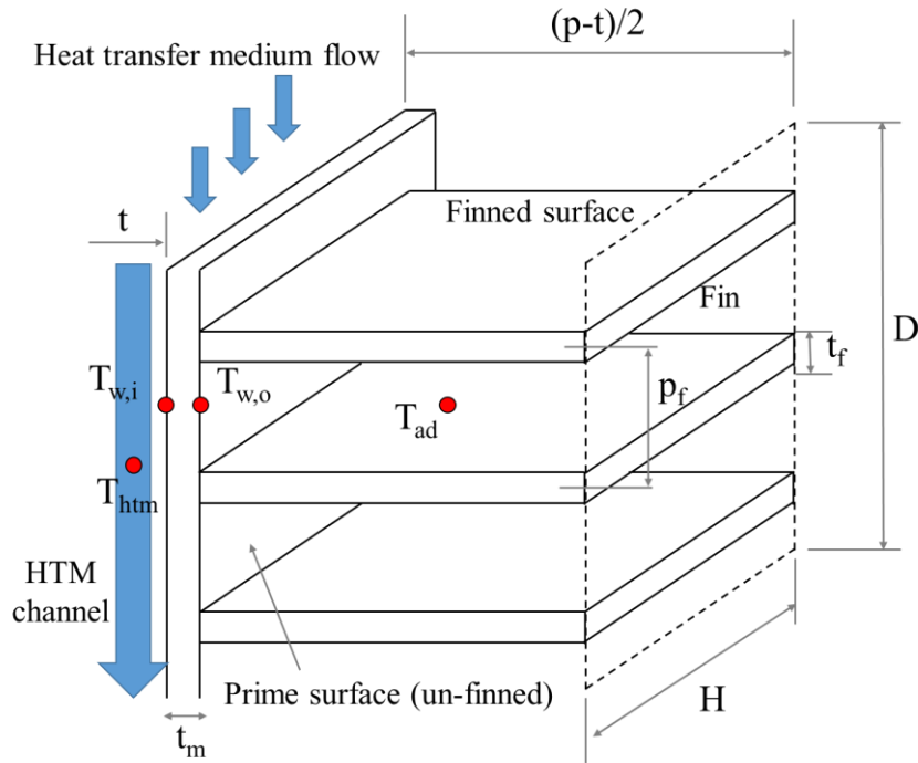
Fig. 4-2 Modelled adsorbent heat exchanger
