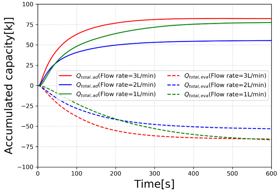
Fig. 3-15 Accumulated heat output profiles for various flow rate where the adsorption and condensation temperature are set at 30°C, desorption and evaporation temperature are set at 80°C and 15°C respectively.
