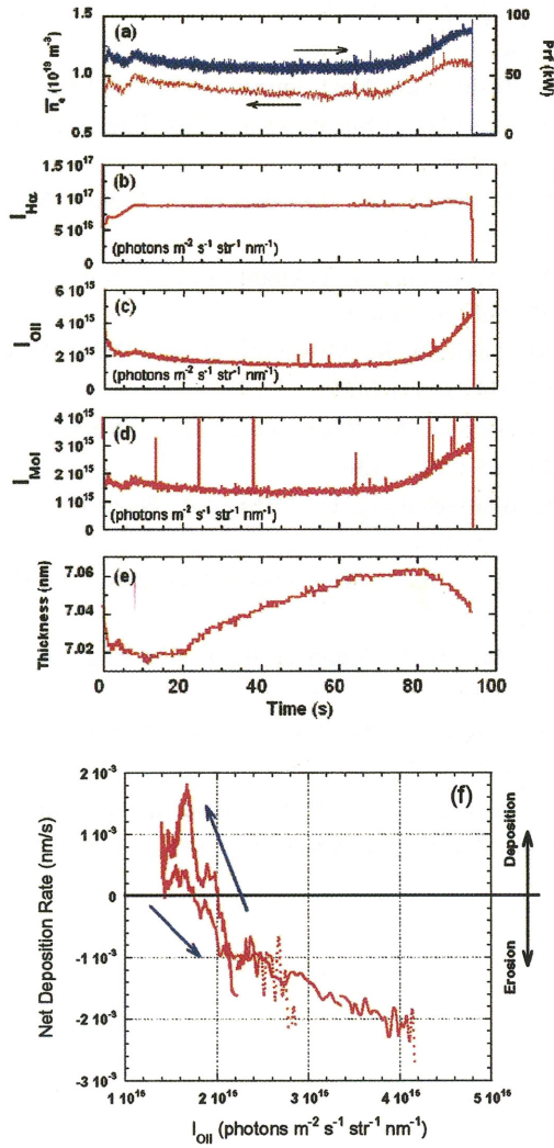
Fig.2 Time evolution of (a) the line average electron density, (b) H_\alpha line intensity, (c) OII line intensity, (d) MoI line intensity, (e) thickness of deposited layer, and (f) deposition rate as a function of OII line intensity.
