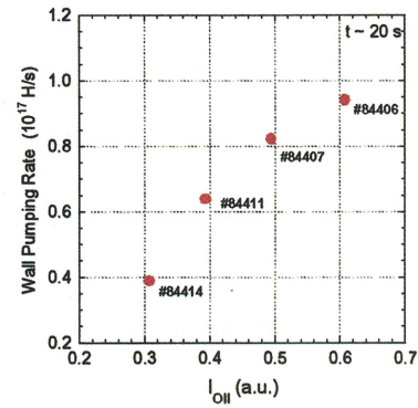
Fig.4 Wall pumping rate at t=20 \text{ s} as a function of OII line intensity.
