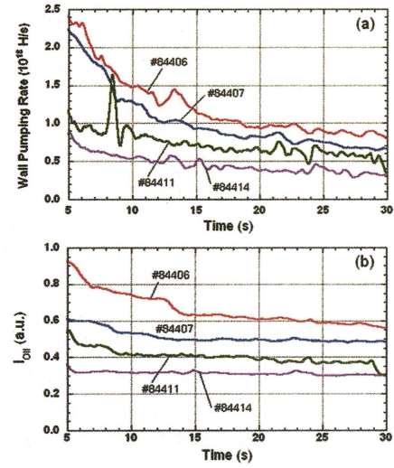
Fig.3 Time evolution of (a) wall pumping rate and (b) OII intensity in the initial discharge phase.
