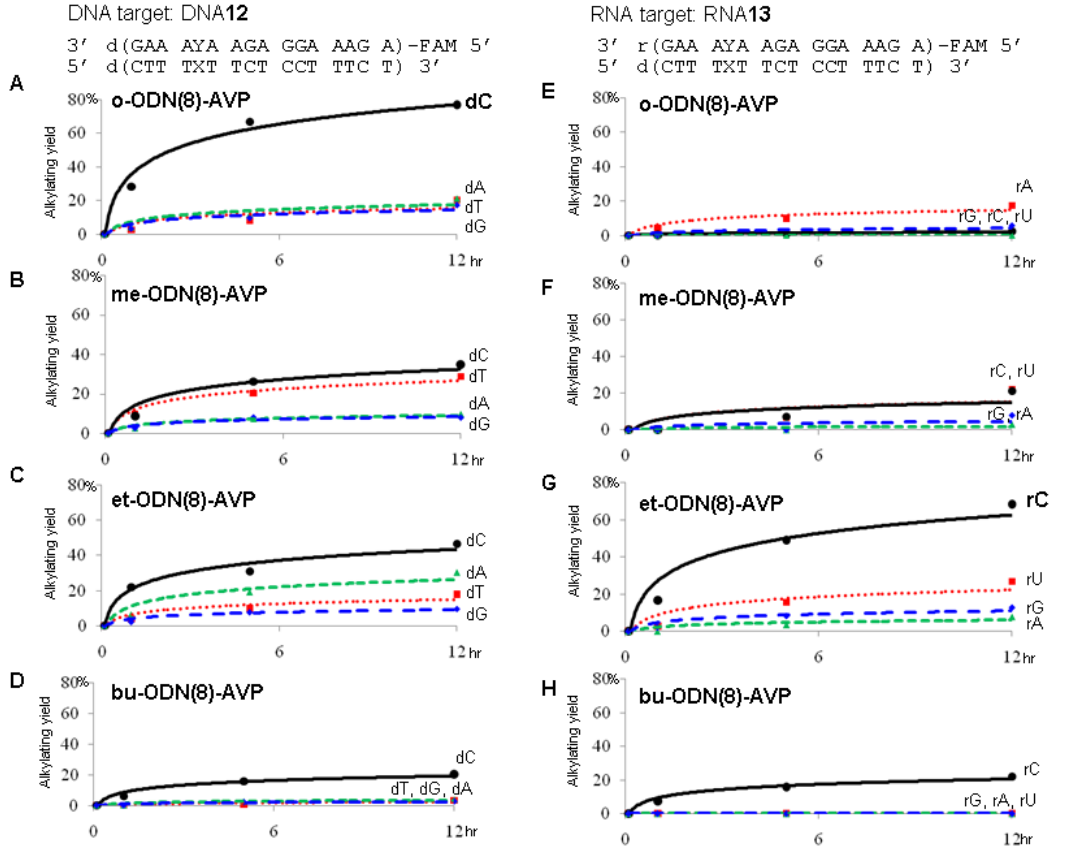
Figure 3. Results of alkylating ability of 10 \mu M 16 mer oligonucleotides (o-ODN(8), me-ODN(8), et-ODN(8), bu-ODN(8)) having AVP derivatives for 1 \mu M FAM labeled target DNA (A-D) and target RNA (E-H) (dC and rC black line, dT and rU red line, dA and rA green line, dG and rG blue line) in the reaction buffer containing 100 mM NaCl, 50 mM MES pH5.0.
