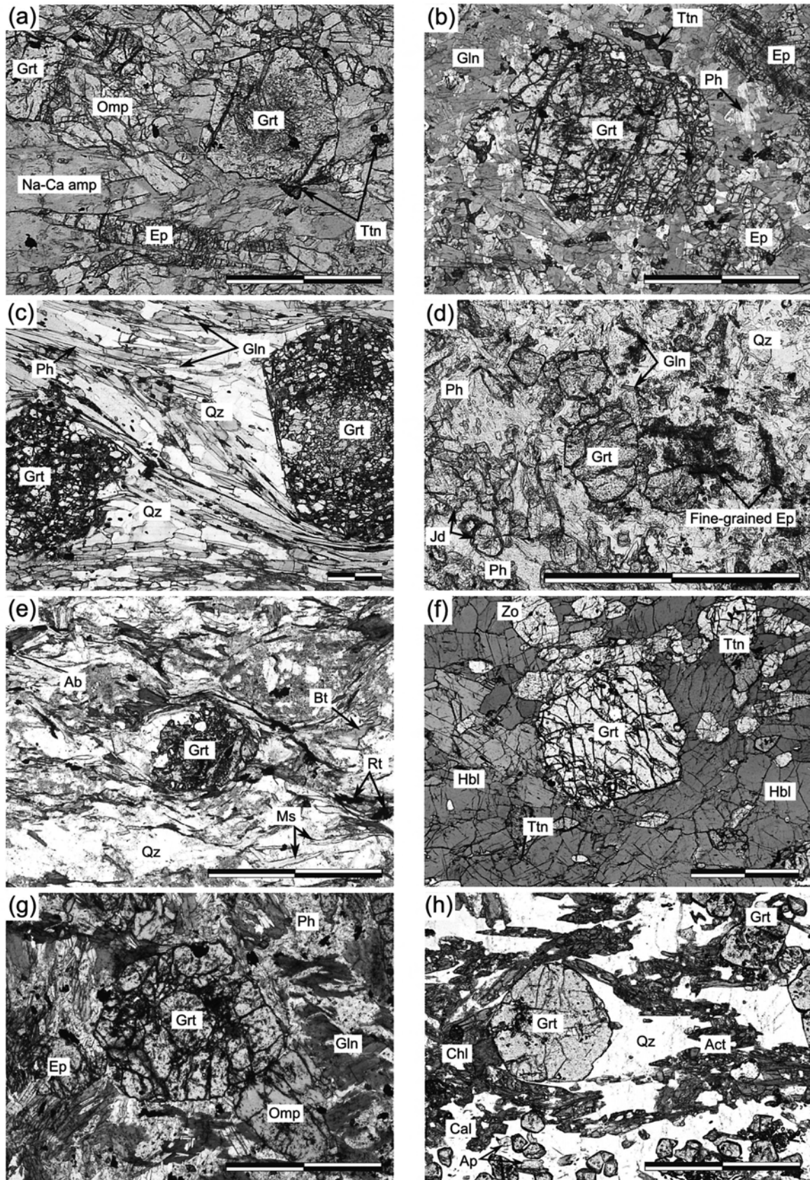
Figure 3. Photomicrographs of metamorphic rocks in central Indonesia. Scale-bars correspond to 1 mm. (a) Eclogite, (b) garnet-glaucophane rock, (c) garnet-glaucophane-phengite-quartz rock, and (d) garnet-jadeite-quartz rock from Bantimala Complex. (e) Garnet-biotite-muscovite-quartz rock from Barru Complex. (f) Garnet amphibolite, (g) eclogite, and (h) garnet-actinolite-quartz schist from Luk Ulo Complex.
