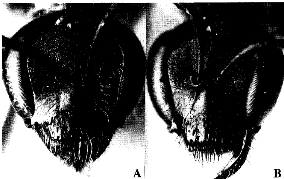
Fig. 18. Head of Lasioglossum (Sudila) alphenum (A) and L. (S.) bidentatum (B), female, seen frontally.
