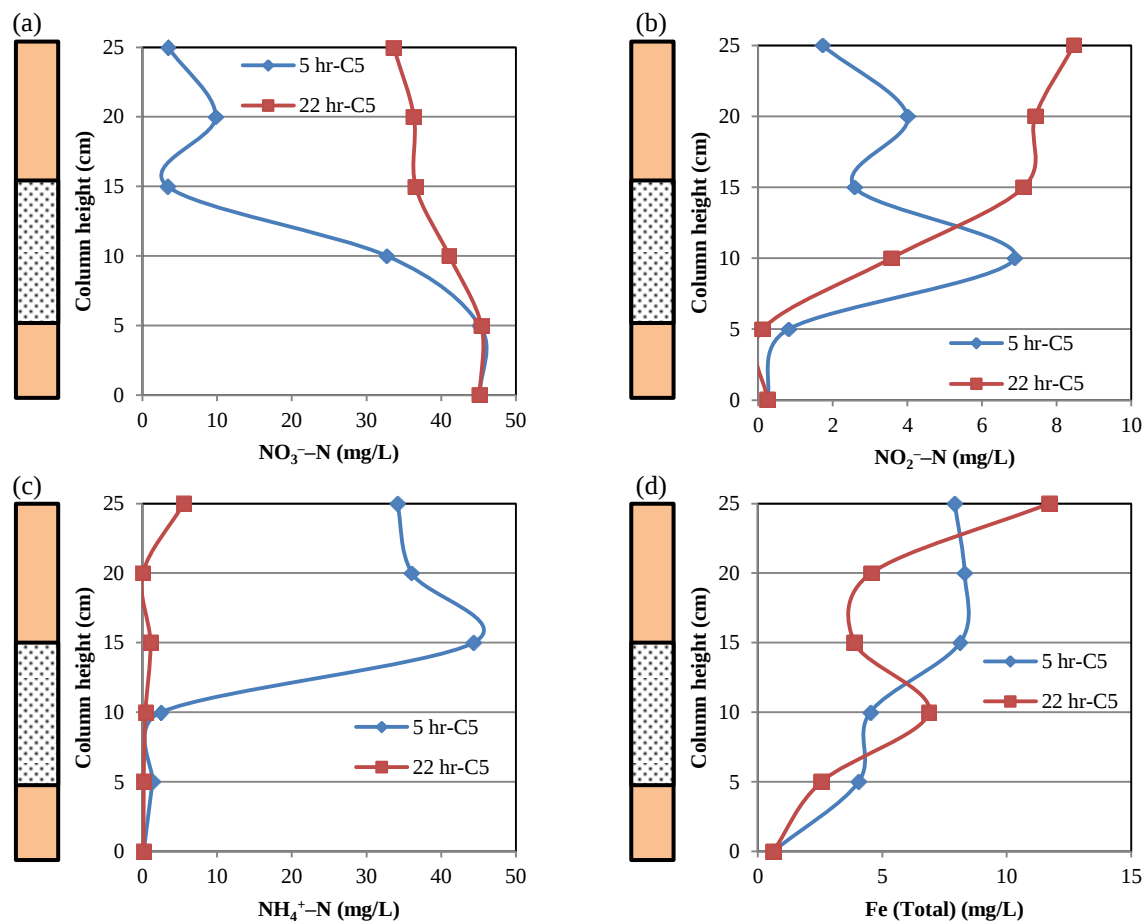
Fig. AI11. Sample profiles of \text{NO}_3^- -N, \text{NO}_2^- -N, \text{NH}_4^+ -N and total Fe concentrations along C5 after 5 and 22 hr feeding with 45 mg \text{NO}_3^- -N/L.
