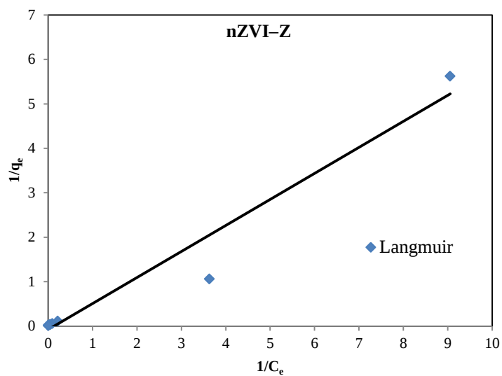
Fig. AIV19. Langmuir isotherm plots for Sr 2+ sorption onto nZVI-Z and nFe/Cu-Z.
