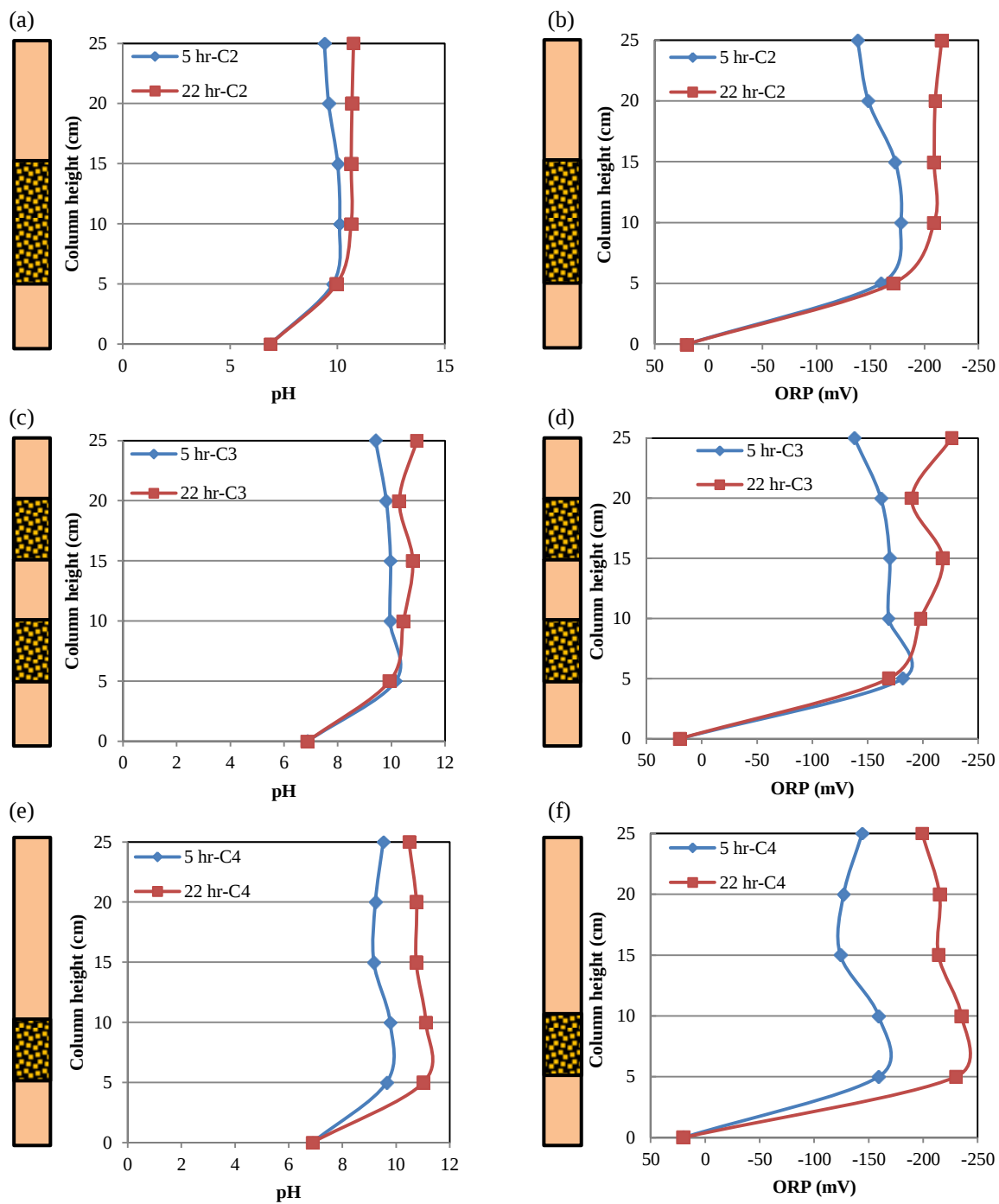
Fig. AI16. Sample profiles of pH and ORP along nZVI/sand columns (C2–C4) after 5 and 22 hr feeding with 45 mg \text{NO}_3^- -N /L.
