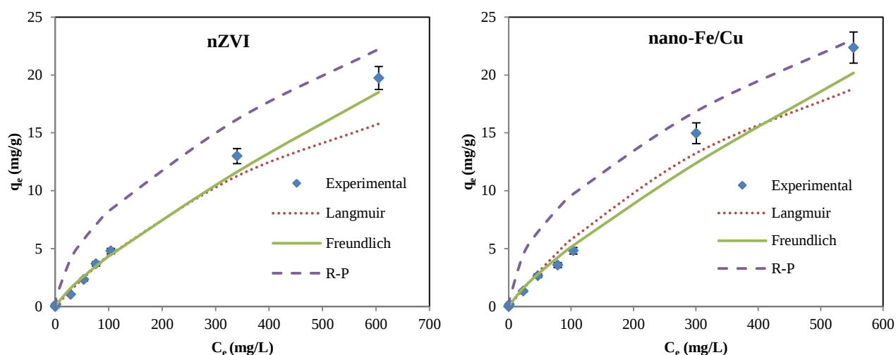
Fig. 4.9. Sorption isotherms of cesium onto nZVI and nano-Fe/Cu particles. (Initial conditions: pH = 6, dosage = 20 g/L, temperature = 298 K).
