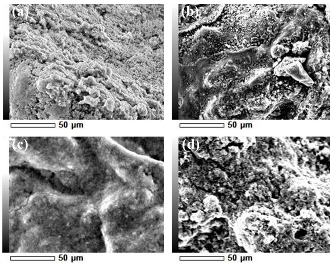
Fig. AII1. SEM images of synthesized (a) nZVI; (b) nano-Fe/Cu particles and the reacted nanoparticle solids acquired at the end of experiments (c) nZVI; (d) nano-Fe/Cu particles.
