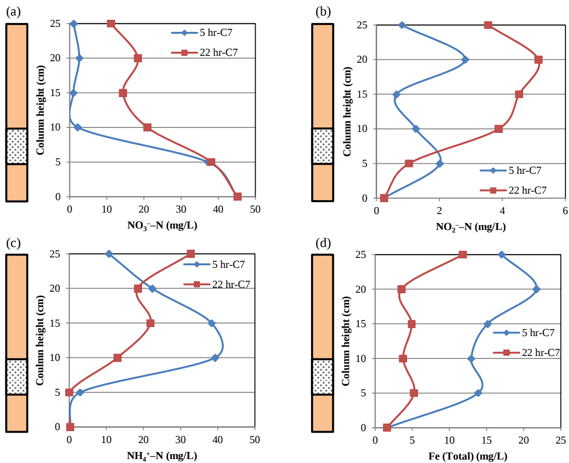
Fig. AI12. Sample profiles of \text{NO}_3^- -N, \text{NO}_2^- -N, \text{NH}_4^+ -N and total Fe concentrations along C7 after 5 and 22 hr feeding with 45 mg \text{NO}_3^- -N /L.
