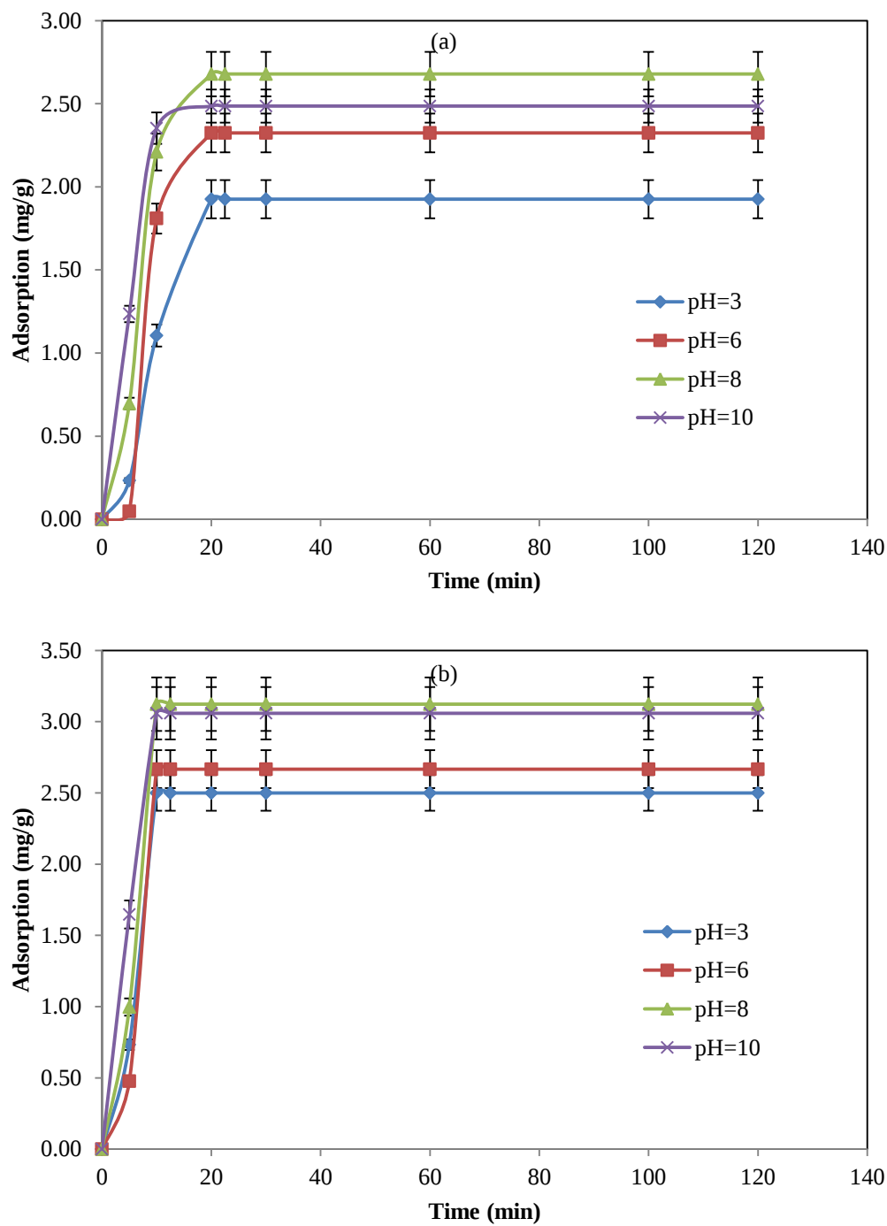
Fig. 4.6. Effect of contact time at different initial pH 3, 6, 8 and 10 on \text{Cs}^+ sorption by (a) nZVI and (b) nano-Fe/Cu particles. (Initial conditions: dosage = 20 g/L, initial \text{Cs}^+ concentration = 100 mg/L, temperature = 298 K).
