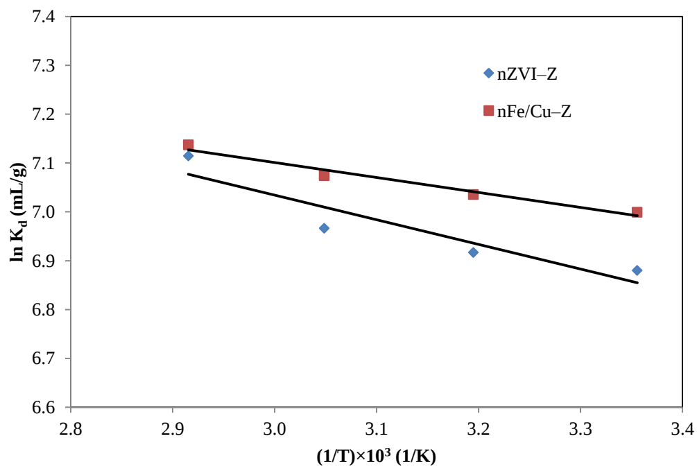
Fig. AIV21. Plot of \ln K_d vs. 1/T for \text{Sr}^{2+} sorption onto nZVI-Z and nFe/Cu-Z.
