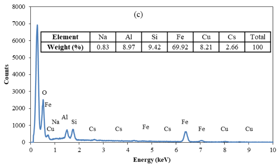
Fig. AIII16. EDS spectrums of (a) zeolite, (b) nZVI-Z composite and (c) nFe/Cu-Z composite acquired at the end of experiments after \text{Cs}^+ adsorption.
