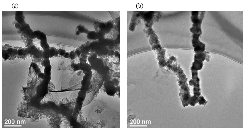
Fig. AI2. TEM images of synthesized (a) nZVI and (b) nano-Fe/Cu particles.
