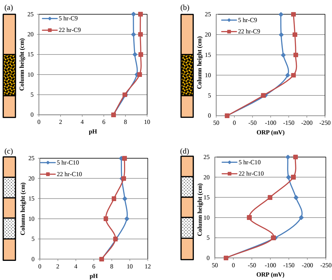
Fig. AI18. Sample profiles of pH and ORP along C9 and C10 after 5 and 22 hr feeding with simulated groundwater containing 45 mg \text{NO}_3^- -N /L.
