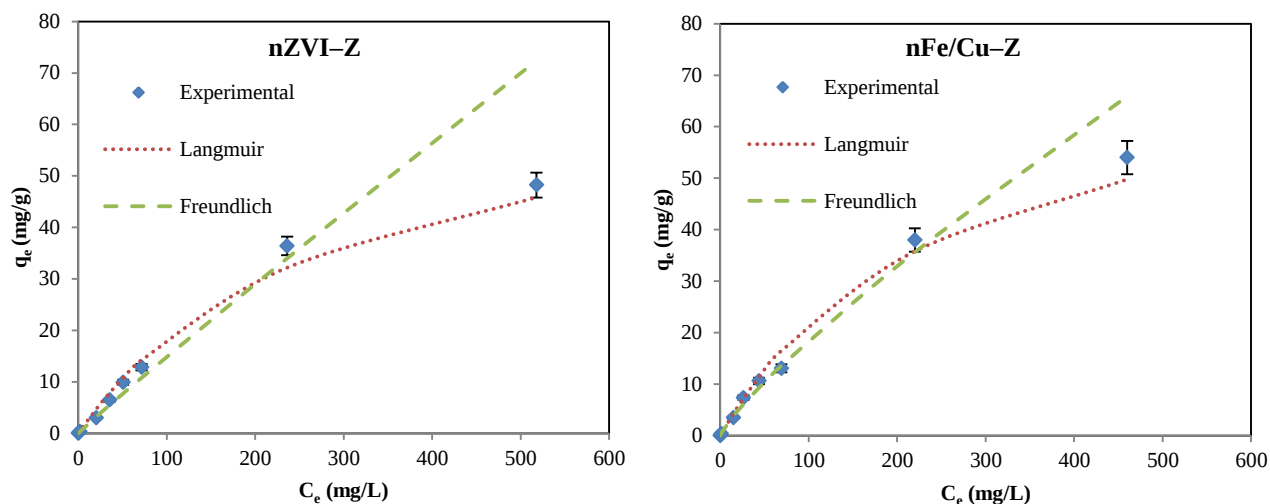
Fig. 5.7. Adsorption isotherms of cesium onto nZVI-Z and nFe/Cu-Z. (Initial conditions: pH = 6, dosage = 10 g/L, temperature = 298 K).
