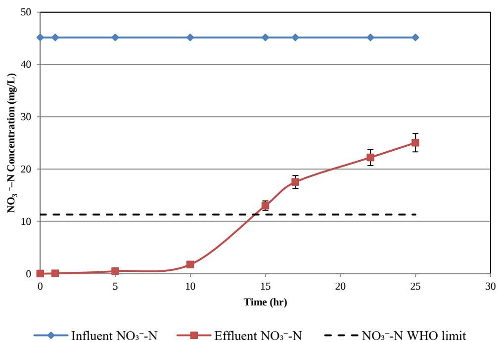
Fig. AI4. Changes in NO 3 - -N concentration over time in C8 with 3 layers of (nano-Fe/Cu)/sand.
