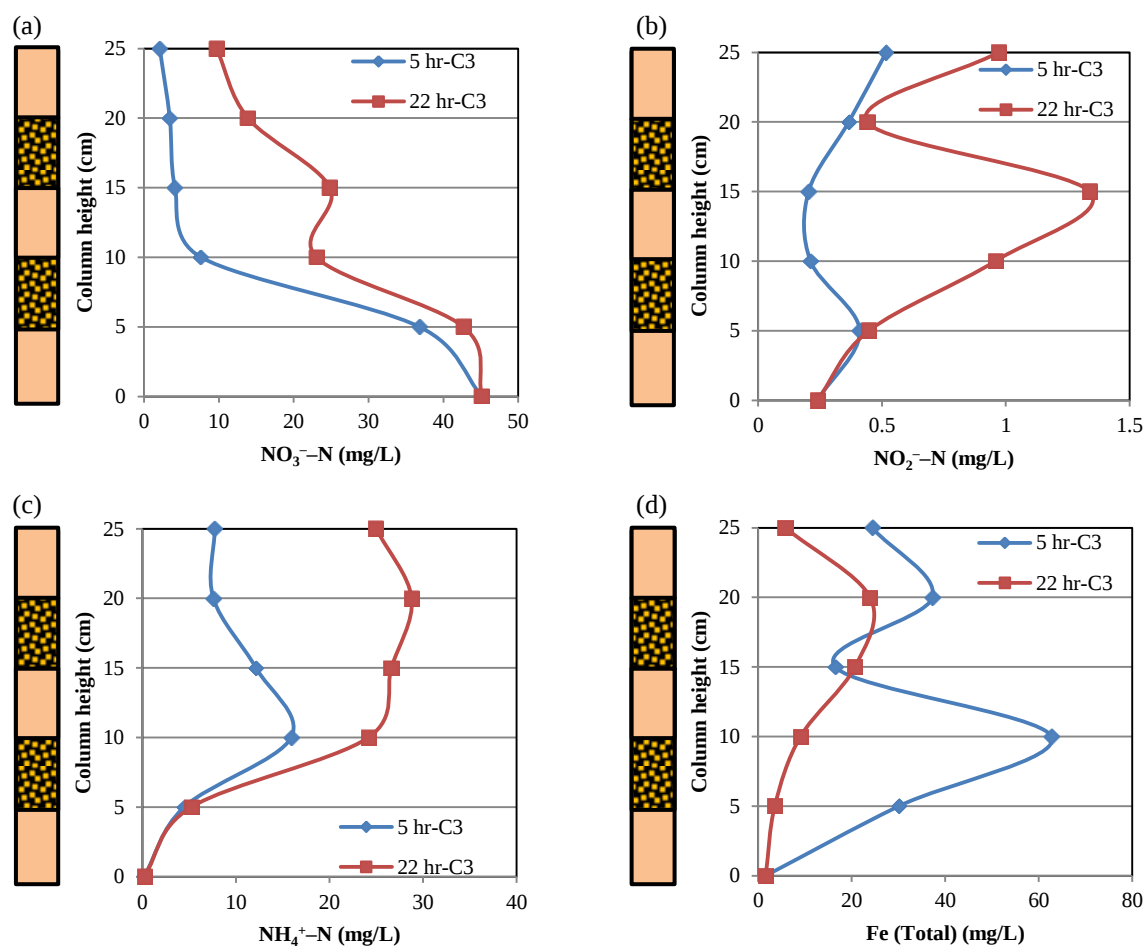
Fig. AI9. Sample profiles of \text{NO}_3^- -N, \text{NO}_2^- -N, \text{NH}_4^+ -N and total Fe concentrations along C3 after 5 and 22 hr feeding with 45 mg \text{NO}_3^- -N /L.
