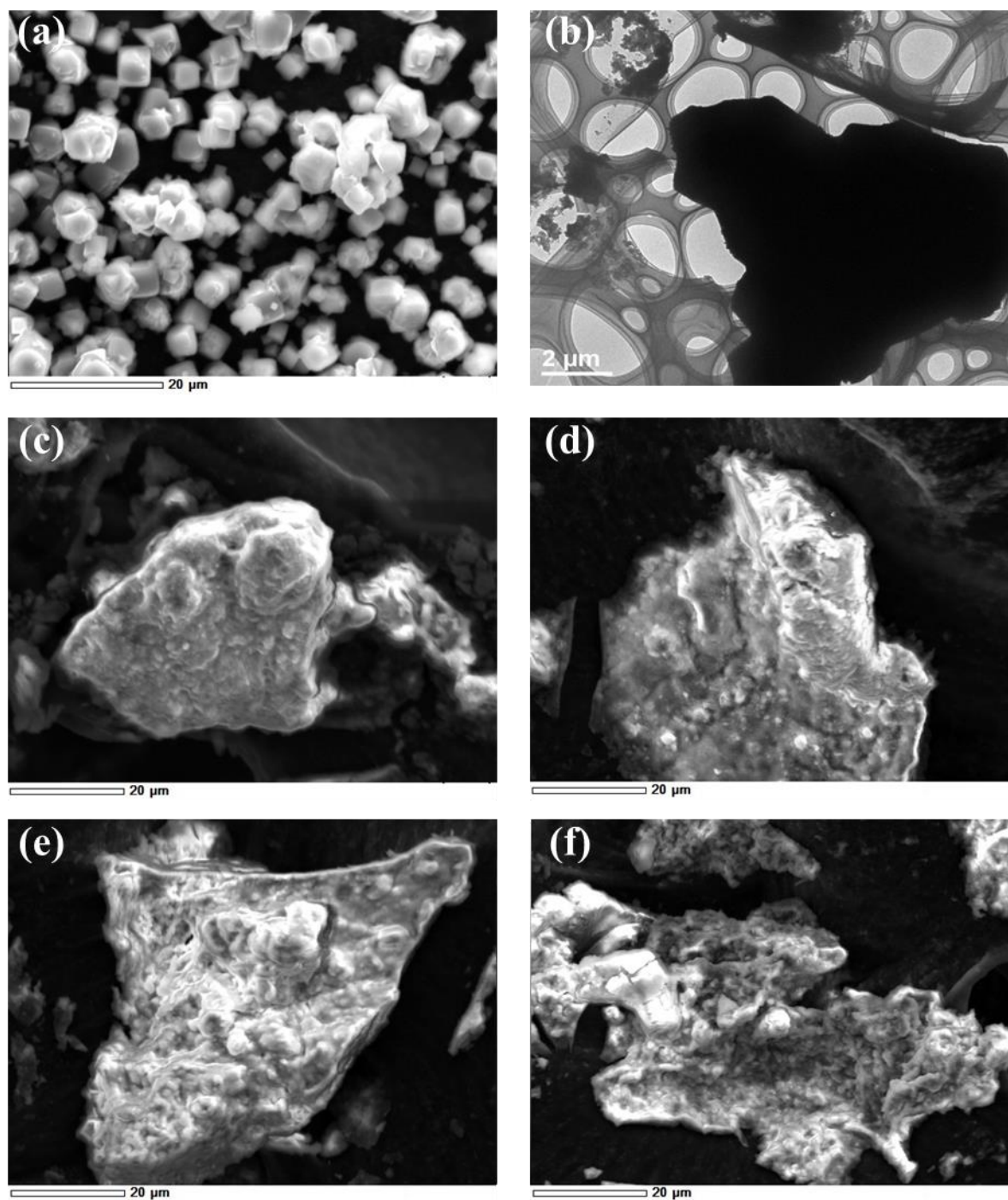
Fig. AIV17. SEM image of (a) zeolite; TEM image of (b) nZVI-Z; SEM images of (c, d) nZVI-Z and (e, f) nFe/Cu-Z.
