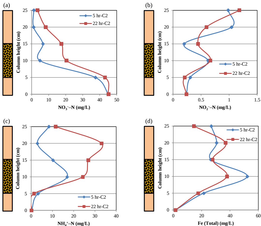
Fig. 3.13. Sample profiles of \text{NO}_3^- -N, \text{NO}_2^- -N, \text{NH}_4^+ -N and total Fe concentrations along C2 after 5 and 22 hr feeding with 45 mg \text{NO}_3^- -N /L.
