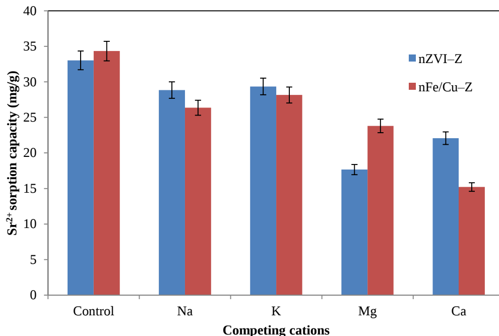
Fig. 6.9. Effect of different competing cation ions on \text{Sr}^{2+} sorption by nZVI-Z and nFe/Cu-Z. (Initial conditions: pH = 6, dosage = 2 g/L, initial \text{Sr}^{2+} concentration = 100 mg/L, temperature = 298 K).
