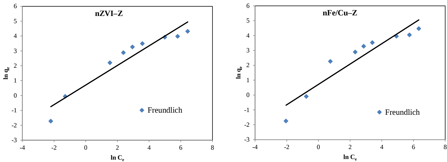
Fig. AIV20. Freundlich isotherm plots for \text{Sr}^{2+} sorption onto nZVI-Z and nFe/Cu-Z.
