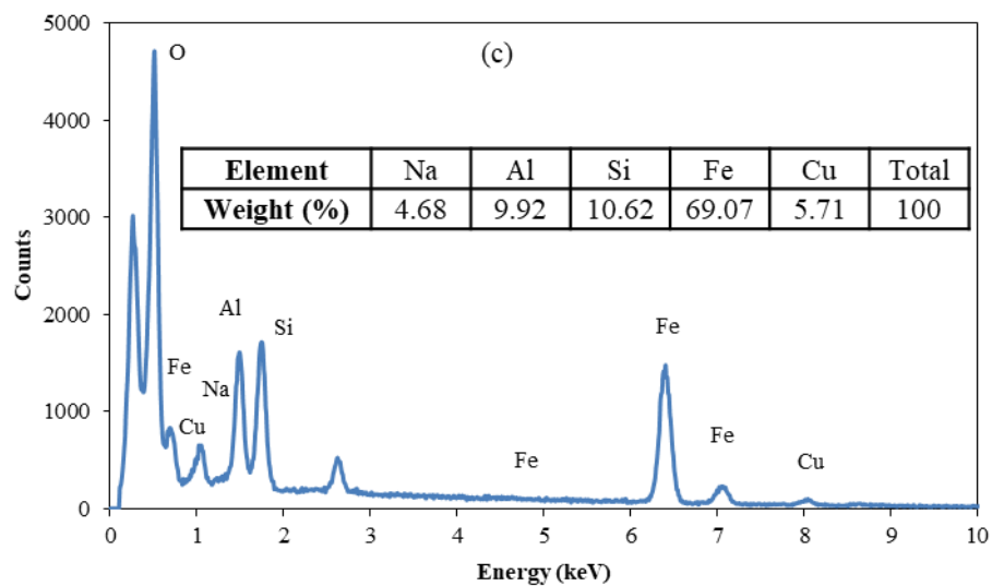
Fig. AIII10. EDS spectra of (a) zeolite, (b) nZVI-Z composite and (c) nFe/Cu-Z composite.
