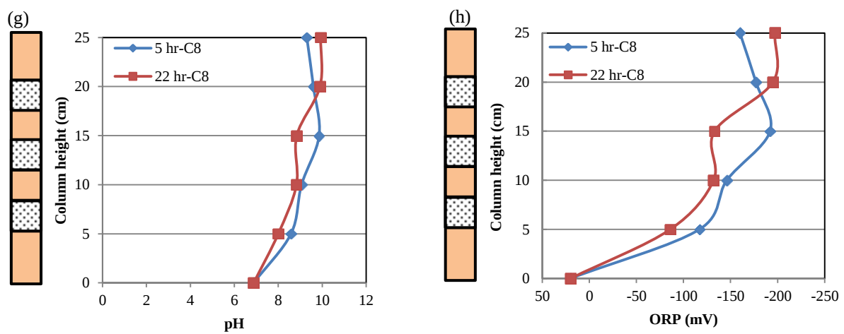
Fig. AI17. Sample profiles of pH and ORP along (nano-Fe/Cu)/sand columns (C5–C8) after 5 and 22 hr feeding with 45 mg \text{NO}_3^- -N /L.
