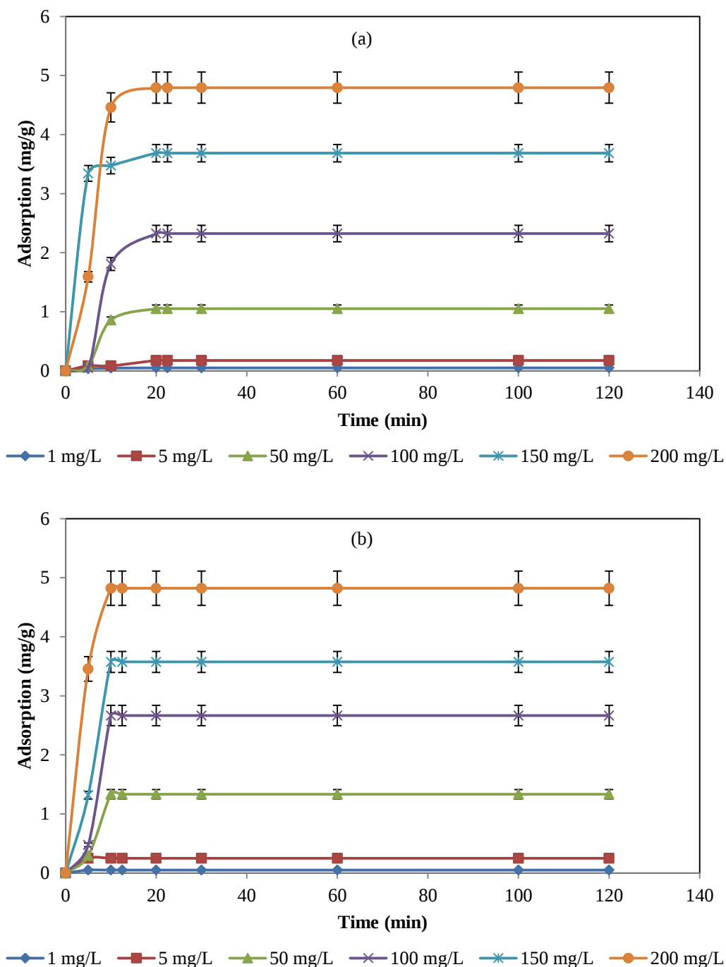
Fig. 4.5. Effect of initial \text{Cs}^+ concentration and contact time on cesium sorption by (a) nZVI and (b) nano-Fe/Cu particles. (Initial conditions: pH = 6, dosage = 20 g/L, temperature = 298 K).
