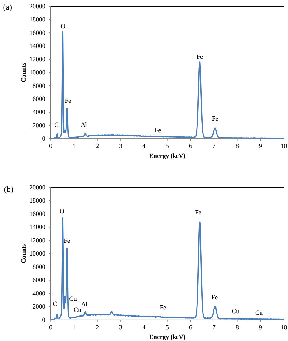
Fig. AII8. EDS spectra acquired from the reacted nanoparticle solids at the end of experiments; (a) nZVI and (b) nano-Fe/Cu particles.
