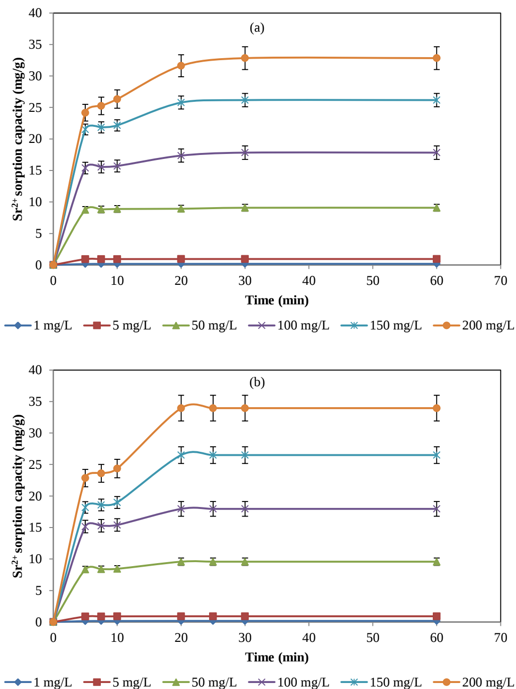
Fig. 6.5. Effect of initial concentration and contact time on \text{Sr}^{2+} sorption by (a) nZVI-Z and (b) nFe/Cu-Z. (Initial conditions: pH = 6, dosage = 5 g/L, temperature = 298 K).
