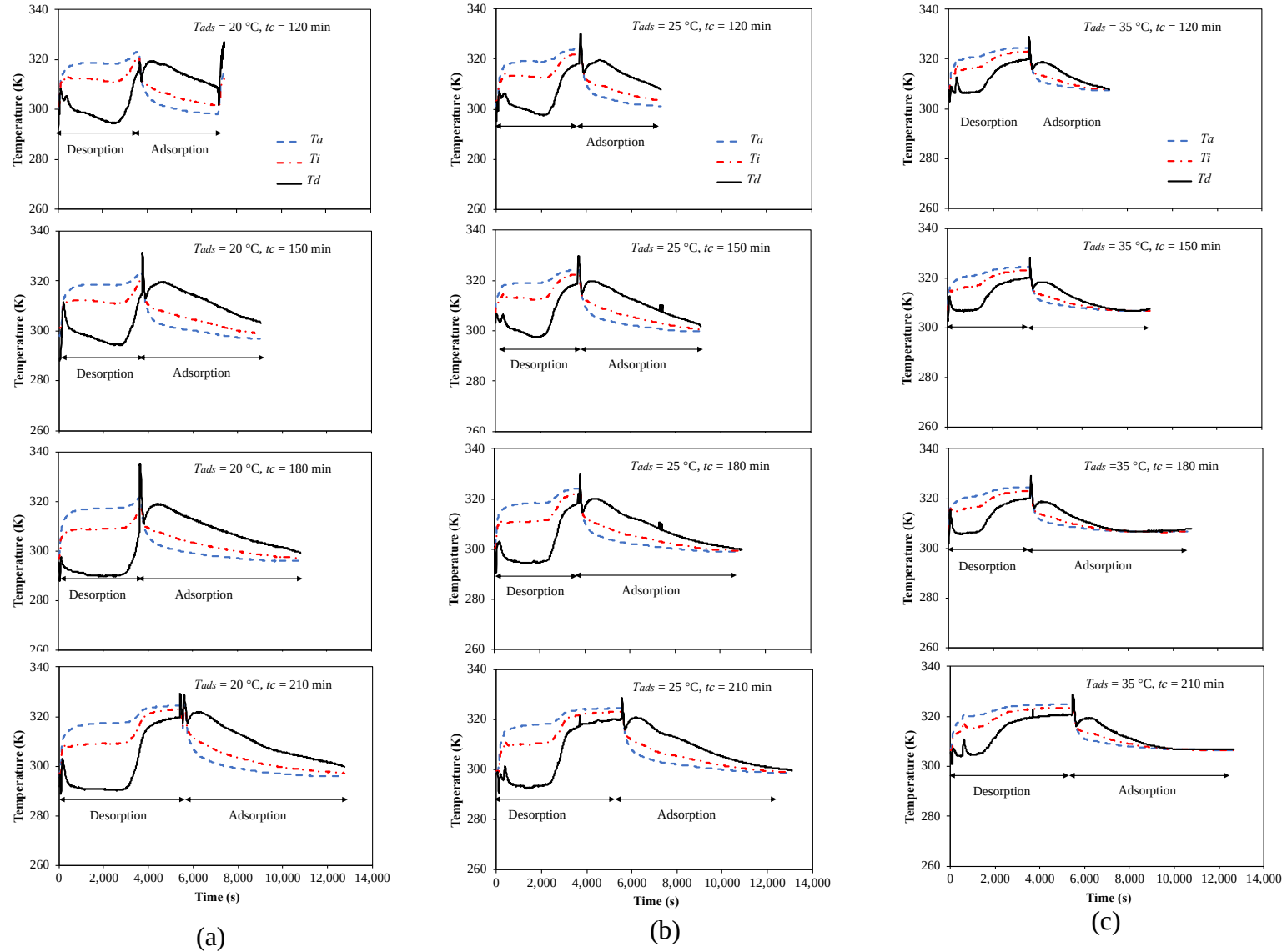
Figure 3.5. Temperature profiles during the experiments at various cycle times under similar adsorption temperature ( T_{ads} ) (a) 20^\circ\text{C} ; (b) 25^\circ\text{C} ; (c) 35^\circ\text{C} .
