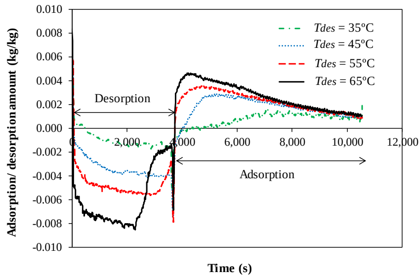
Figure 4.1. Adsorption/desorption amount for different desorption temperature.
