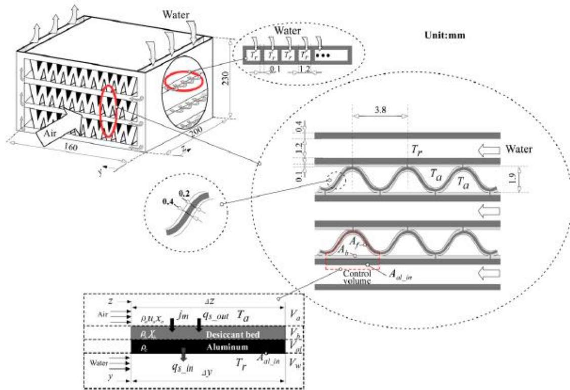
Figure 1.4. Schematic diagram of the batch-type dehumidification system with an internal heat exchanger (Jeong et al., 2011).
