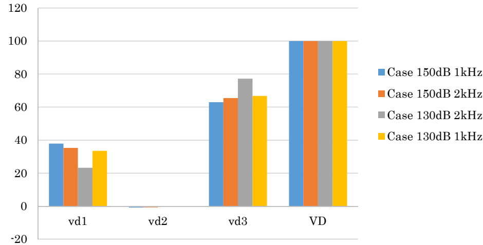
Figure V-26 Percentage of the absorption caused by each term of the viscous dissipation term, cases without bias flow
