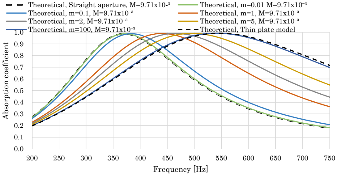
Figure VI-15 Absorption coefficient at different tapering slope
