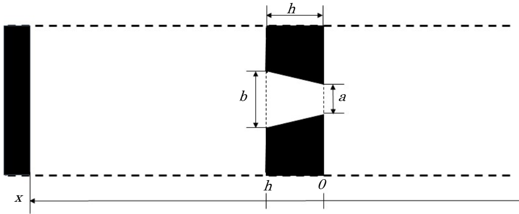
Figure VI-6 Perforated plate with tapered aperture
