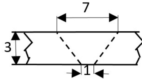
Figure V-3 Tapered aperture
