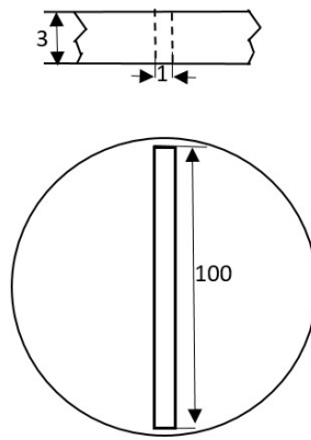
Figure IV-7 Straight aperture, unit: [mm]
