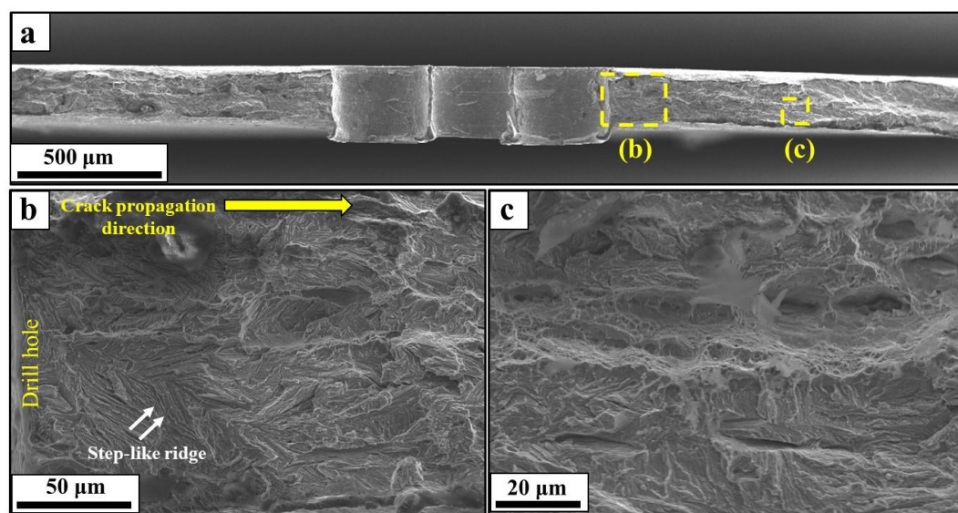
Fig. 3.13. (a) The entire fracture surface of the hydrogen-charged 3DH specimen. High magnification details of the areas highlighted in (a) are presented in (b) and (c).
