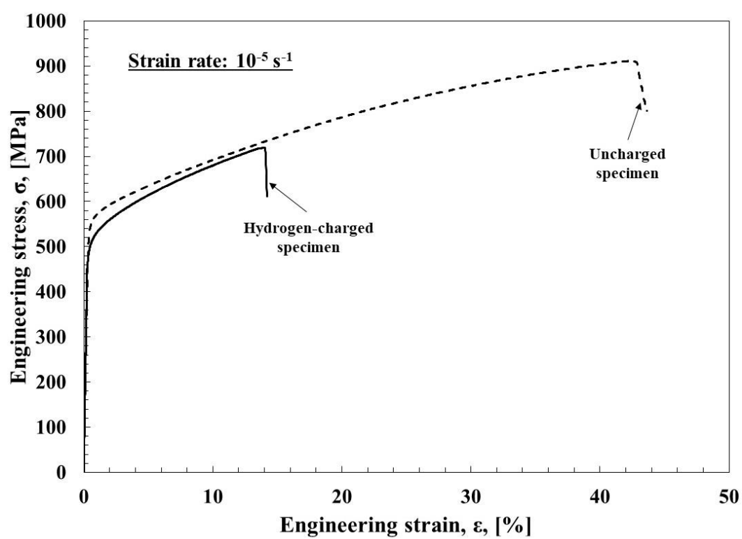
Fig. 2.6. Engineering stress–strain curves of hydrogen-charged and uncharged specimens.
