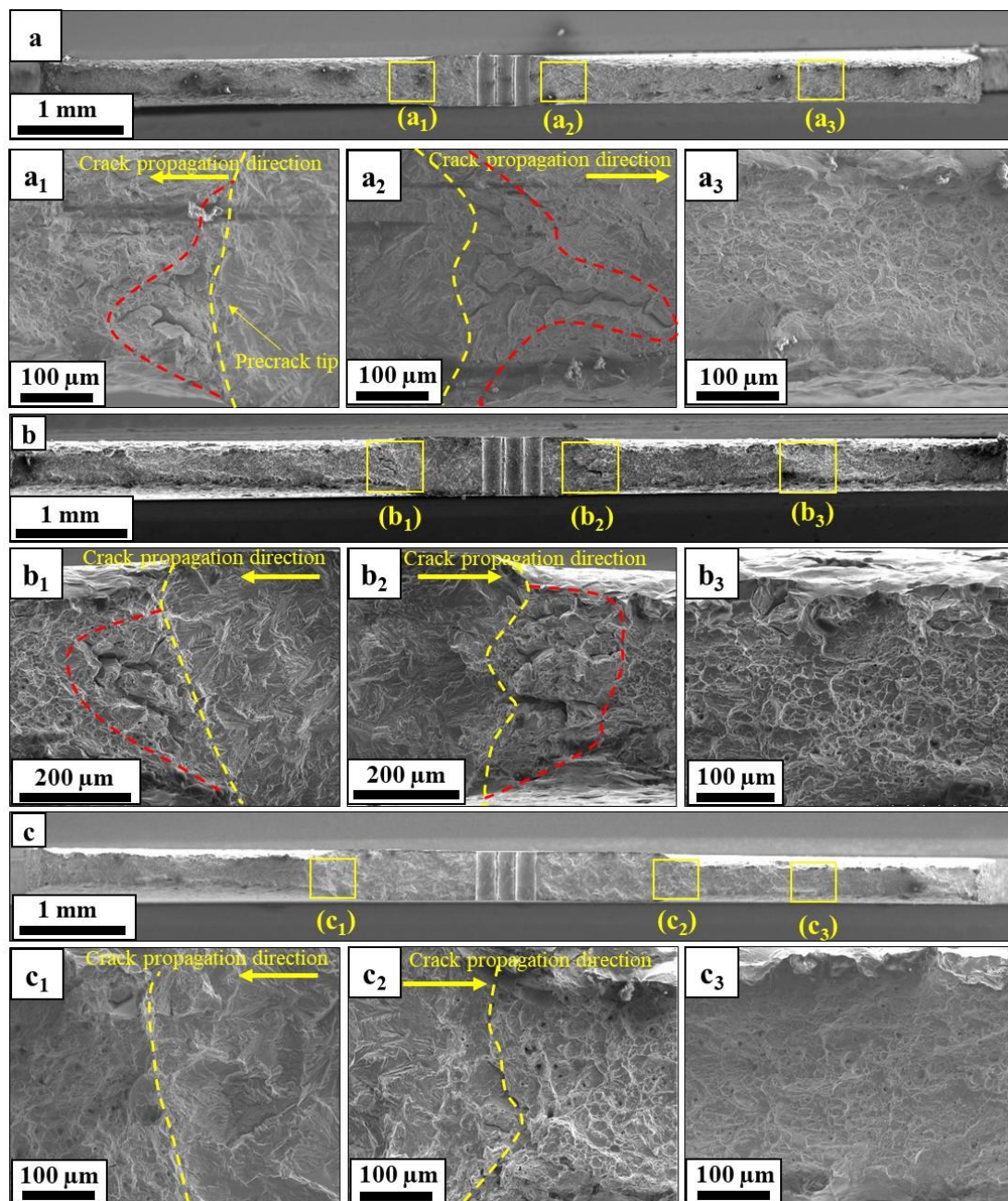
Fig. 4.11. (a), (b) and (c) overall images of fracture surfaces of hydrogen-charged specimen with 1, 1.8 and 3.2 mm precracks, respectively. X_1 and X_2 show the both sides of the fracture surfaces including precrack tips. For 1 and 1.8 mm precracks the fracture surfaces in front of the crack tip display the combination of intergranular and quasi-cleavage features, while, 3.2 mm precracked specimen show ductile feature as a void coalescence similar to the uncharged specimens. The remain parts of the fracture surface covered by dimples as shown in Figs. (a 3 ), (b 3 ) and (c 3 ). The yellow and red dashed-lines indicate the precrack tip and enclosed the brittle zone, respectively.
