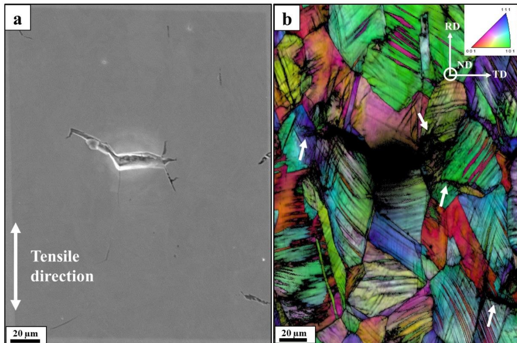
Fig. 5.6. (a) SEM image and (b) corresponding RD-IPF map of surface crack in the vicinity of the fracture surface of 1.8 mm precracked specimen at the strain rate of 10 -5 s -1 . The RD-IPF map is superimposed with the IQ contrast.
