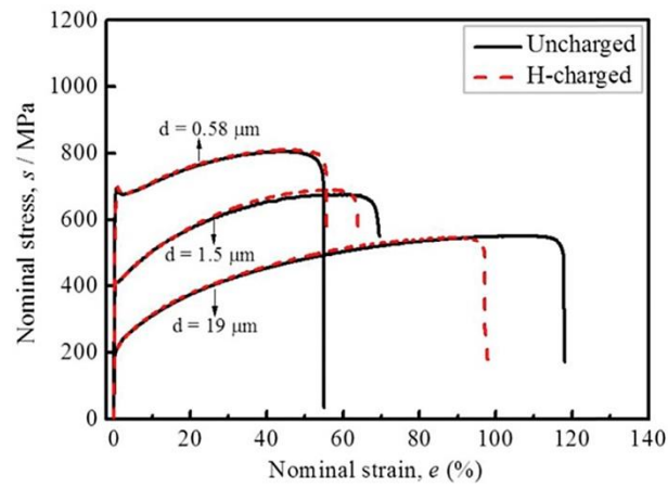
Fig. 1.6. Impact of grain refinement on hydrogen embrittlement in an Fe-31Mn-3Al-3Si TWIP steel hydrogen-pre-charged at 100 A/m 2 in a 3% NaCl aqueous solution containing 3 g/L of NH 4 SCN. The initial strain rate is 8.3 \times 10^{-6} \text{ s}^{-1} . Alloy composition is given in weight %[94].
