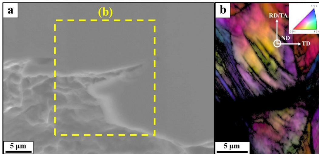
Fig. 3.8. (a) SEM image and (b) corresponding RD-IPF map of the surface crack at the vicinity of the fracture surface in 3DH specimen. The RD-IPF map is superimposed with the IQ contrast.
