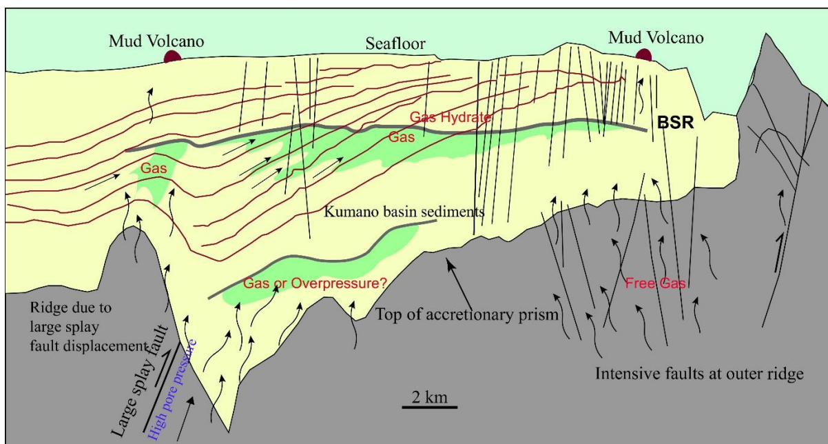
Figure 2.12 Schematic model of hydrocarbon gas migration processes and formation in the Kumano forearc basin on profile of IL 2460
