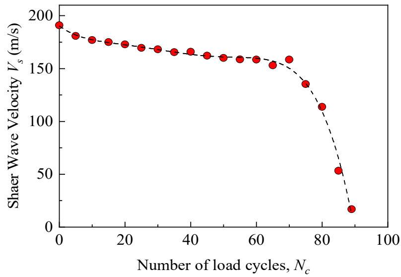
Figure 6.8 Variation of shear wave velocity during cyclic loading (Toyoura sand with D_r = 60\% ).
