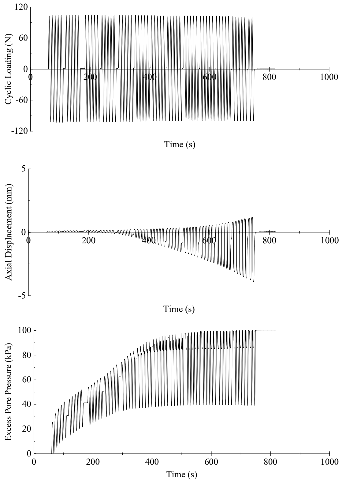
Figure 4.6 The time history of axial force, axial displacement and excess pore in first cyclic test for Toyoura sand with Dr = 70\% ( CSR = 0.257 )
