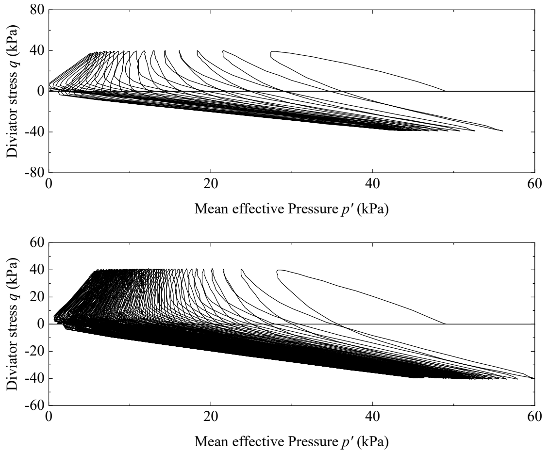
Figure 5.5 Stress path of first and second cyclic tests for Kuroboku moved out fines with initial relative density D_r = 60\%
