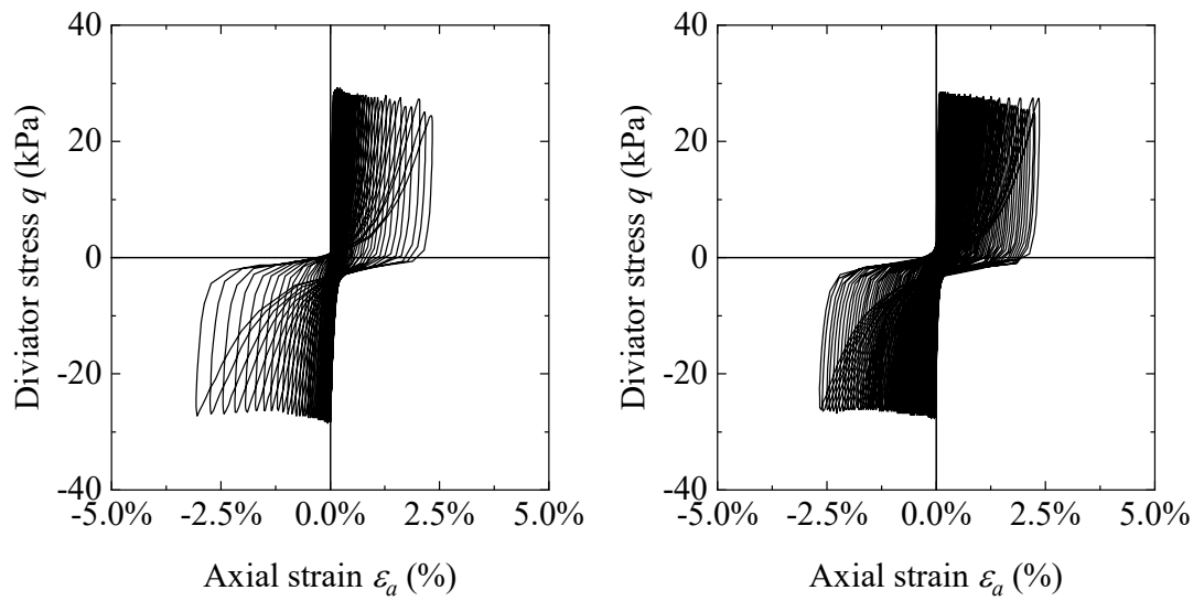
Figure 5.12 Shear stress-strain relation between first and second cyclic tests for boiled sand with initial relative density D_r = 80\%
