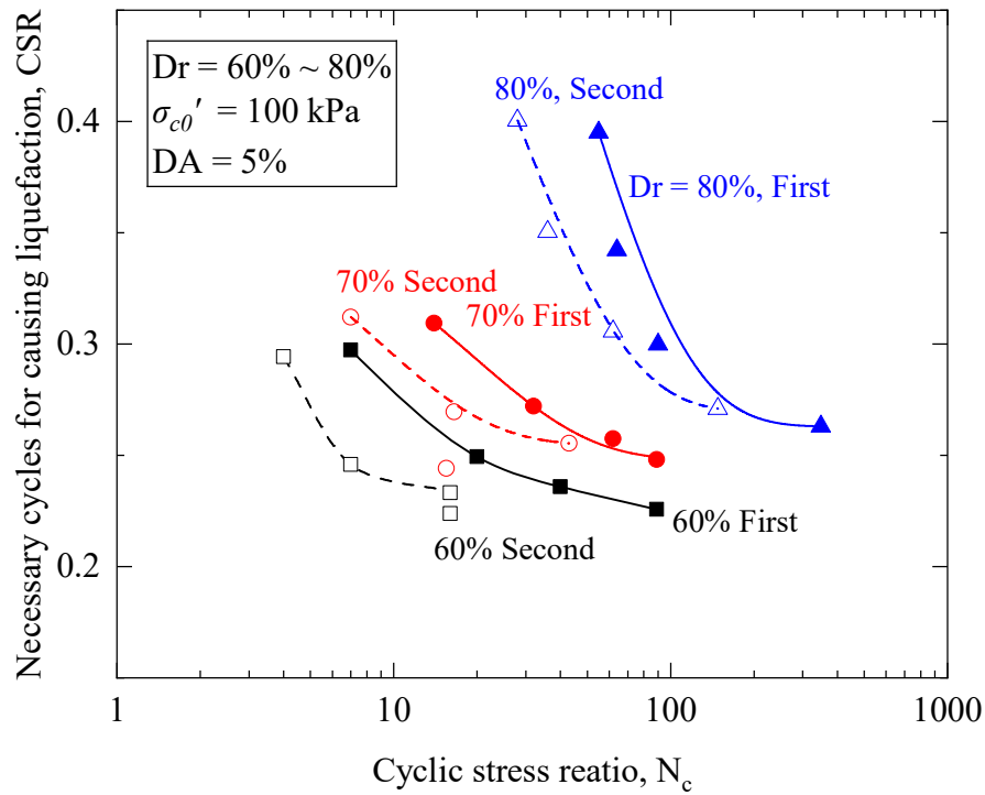
Figure 4.23 Comparison of liquefaction resistances between first and second cyclic tests for Toyoura sand with the relative density: 60\% \sim 80\% .
