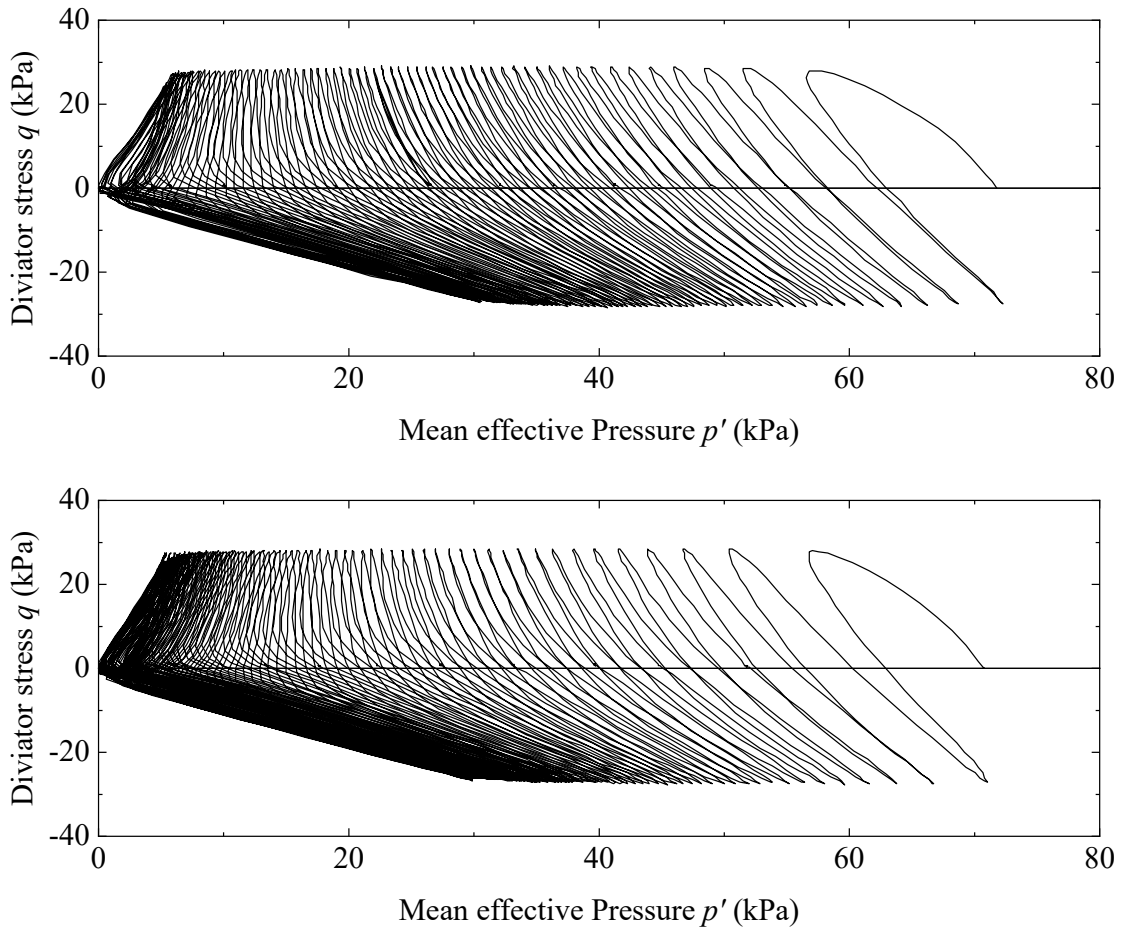
Figure 5.11 Stress path of first and second cyclic tests for boiled sand with initial relative density D_r = 80\%
