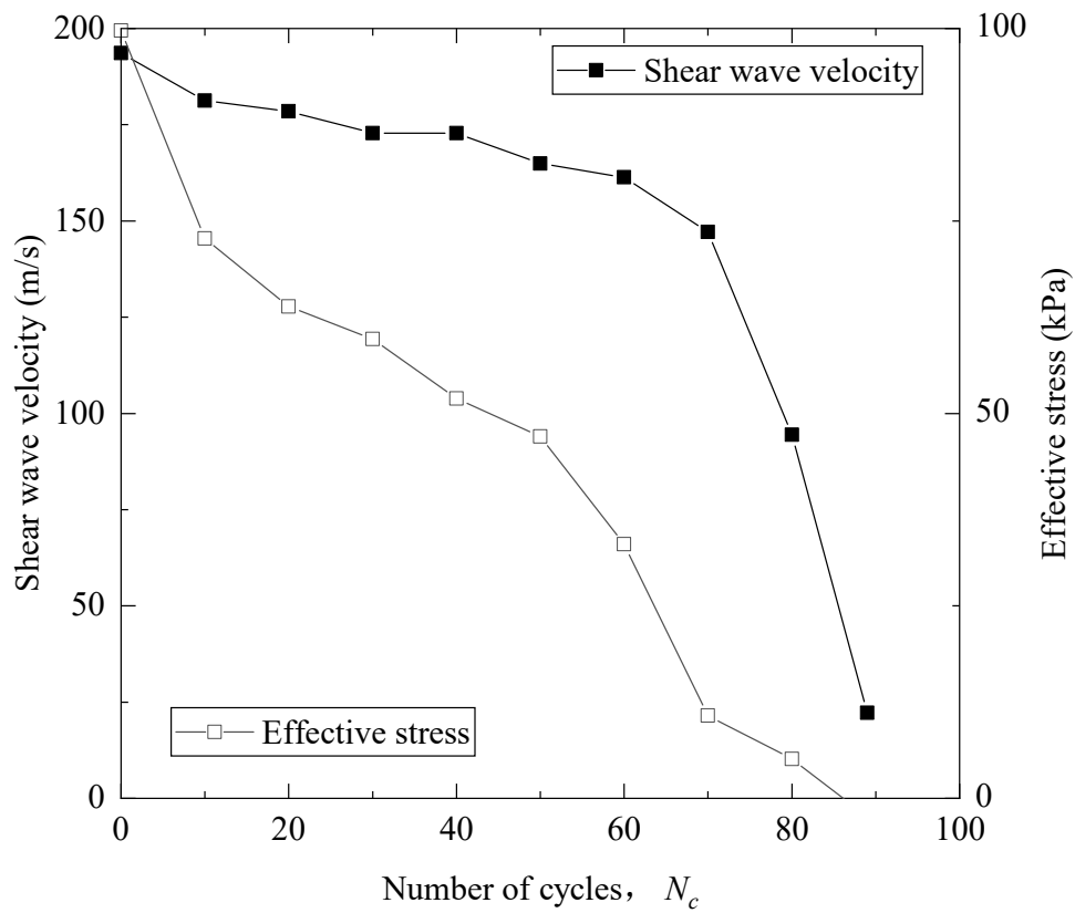
Figure 6.9 Variation of effective stress together with shear wave velocity during cyclic loading (Toyoura sand with D_r = 70\% )
