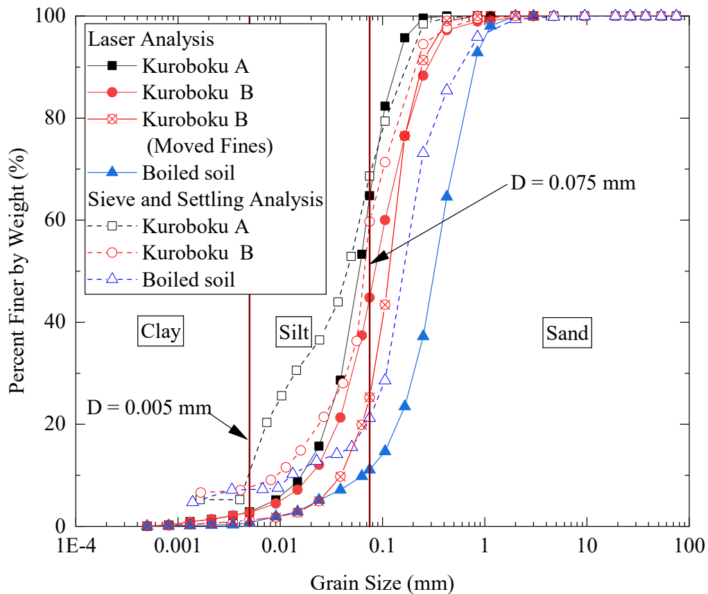
Figure 5.1 Cumulative grain size distribution of Kuroboku and boiled sand
