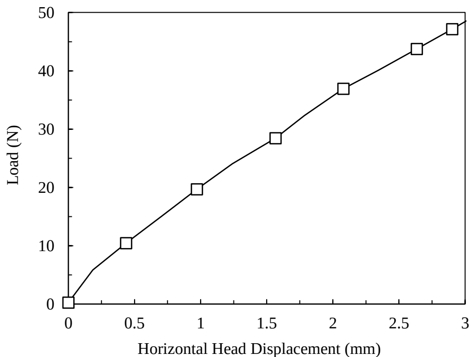
Figure 3-9 Typical result of a monotonic test for single pile
