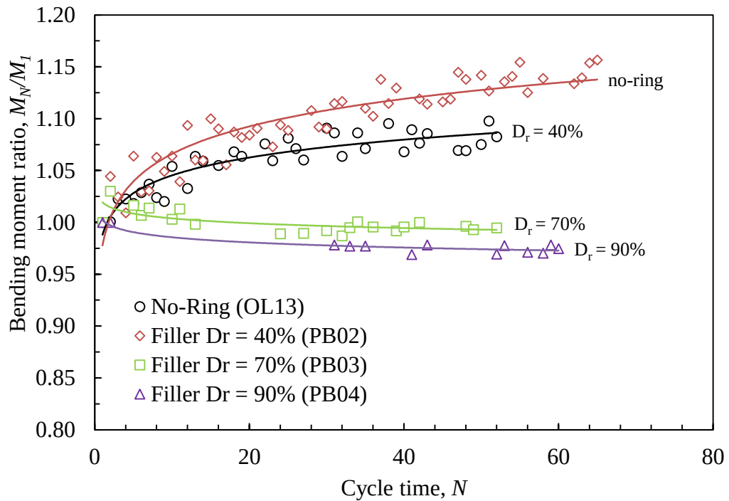
Figure 4-24 Effect of density on bending moment of pre-bored pile system under cyclic lateral loading
