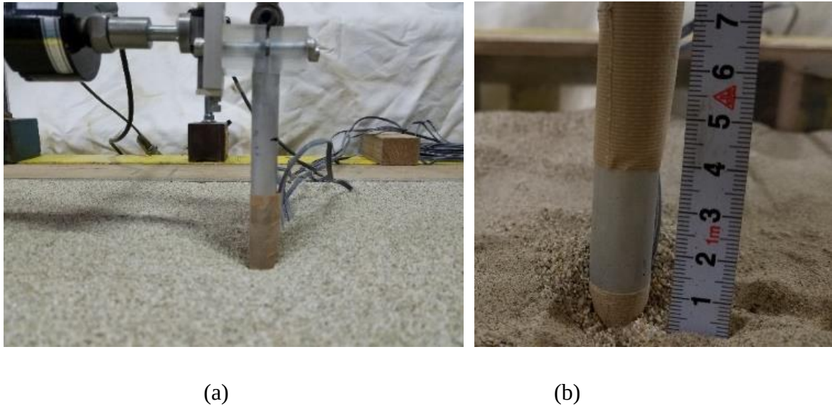
Figure 4-14 Soil condition after 50-time of cyclic loading for the layer depth ratio ( x/D ) of 3, (a) condition on surface layer (b) condition on the border layer
