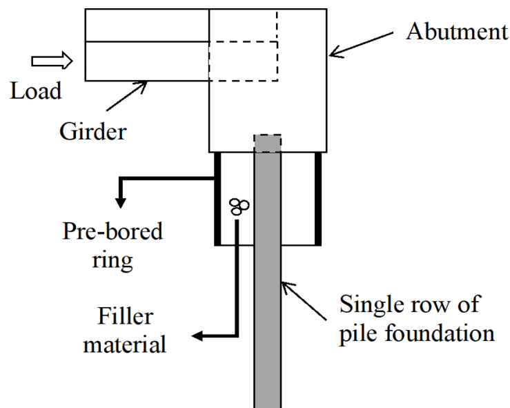
Figure 1-4 Typical design of integral abutment bridge with a pre-bored hole system.
