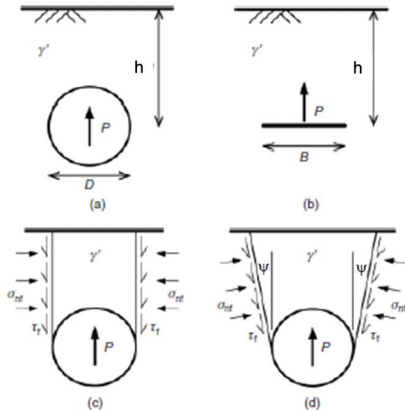
Figure 6-3 Failure mechanism of uplift pipe (a) pipe geometry; (b) strip geometry; (c) vertical slip mechanism; (d) inclined slip mechanism (White et al., 2008)
