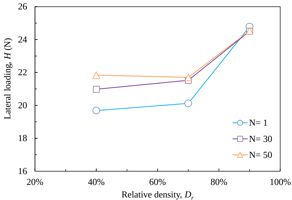
Figure 4-22 Lateral capacity of pre-bored pile foundation with different filler material density
