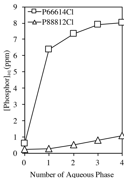
Figure 2.11. Ionic liquid cation release to the aqueous phase after repeated contact with an aqueous phase.; [M]_{aq} = 0 \text{ mg L}^{-1} , V_{aq}/V_{IL} = 2 , time = 3 hours, Aq phase= 0.5 \text{ mol L}^{-1} HCl
