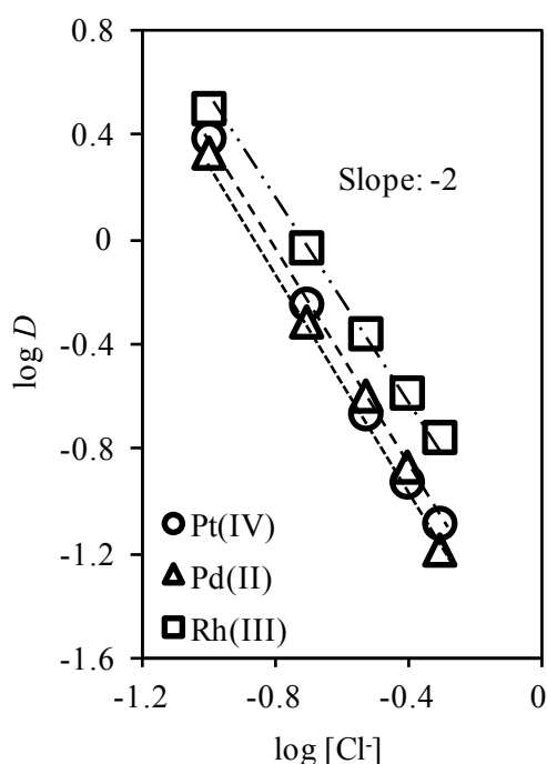
Figure 2.6. Effect of chloride ion concentration on the distribution ratio of Pt(IV), Pd(II), and Rh(III); Aqueous phase: [M]_{aq} = 100 \text{ mg L}^{-1} , [H^+]_{aq} = 0.5 \text{ mol L}^{-1} , [Cl^-] = 0.1\text{-}0.5 \text{ mol L}^{-1} (adjusted with 0.5 \text{ mol L}^{-1} HCl and HClO_4 ); Organic phase: [P_{8,8,8,12}Cl] = 0.07 \text{ mol L}^{-1} (Pt(IV) and Pd(II)) and 0.12 \text{ mol L}^{-1} (Rh(III)), toluene, V_{aq}/V_{IL} = 2 , time = 3 hours.
