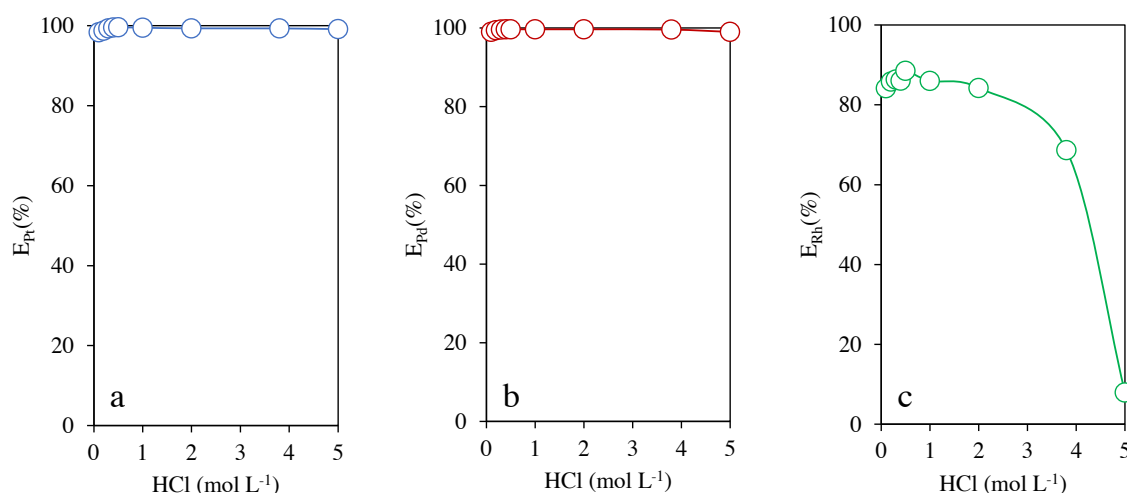
Figure 2.3. Effects of HCl concentration on the (a) Pt(IV), (b) Pd(II), and (c) Rh(III) extraction by \text{P}_{8,8,8,12}\text{Cl} ; [\text{M}]_{\text{aq}} = 100 \text{ mg L}^{-1} , V_{\text{aq}}/V_{\text{IL}} = 2 , time = 3 hours.
