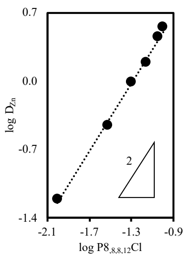
Figure 4.5. Effect of P 8,8,8,12 Cl concentration on (A) Zn(II) extraction ([M] aq = 50 mg L −1 , V aq /V IL = 2, [P 8,8,8,12 Cl] = 0.01–0.1 mol L −1 , solvent = toluene).
