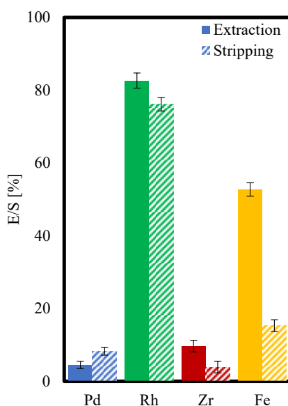
Figure 3.7. Extraction of \text{Rh(III)} from the raffinate ( 1 \text{ mol L}^{-1} \text{ HCl} ) and stripping of \text{Rh(III)} using 5 \text{ mol L}^{-1} \text{ HCl} . Conditions: V_{\text{aq}}/V_{\text{IL}} = 2 , T = 298 \text{ K} , time = 5 h.
