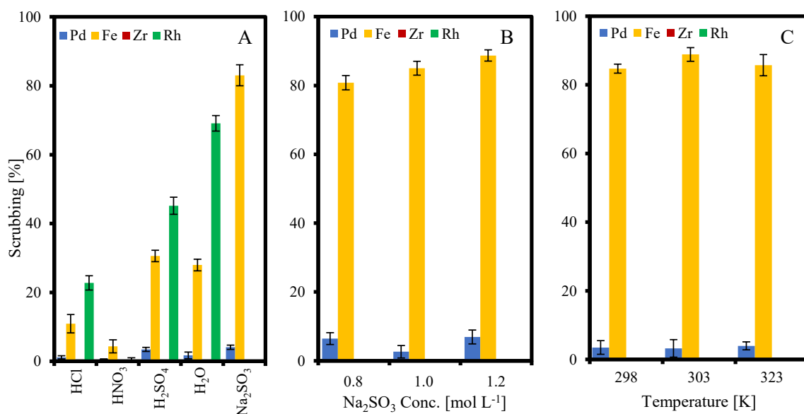
Figure 3.4. Fe scrubbing from loaded P 8,8,12 Cl. (A) The results obtained using 0.1 mol L -1 HCl, 0.5 mol L -1 HNO 3 and H 2 SO 4 , water and 1.0 mol L -1 Na 2 SO 3 at 323 K. (B) The effect of Na 2 SO 3 concentration at 323 K and 30 min. (C) The effect of temperature using 1 mol L -1 Na 2 SO 3 at 30 min and V aq /V IL = 2.
