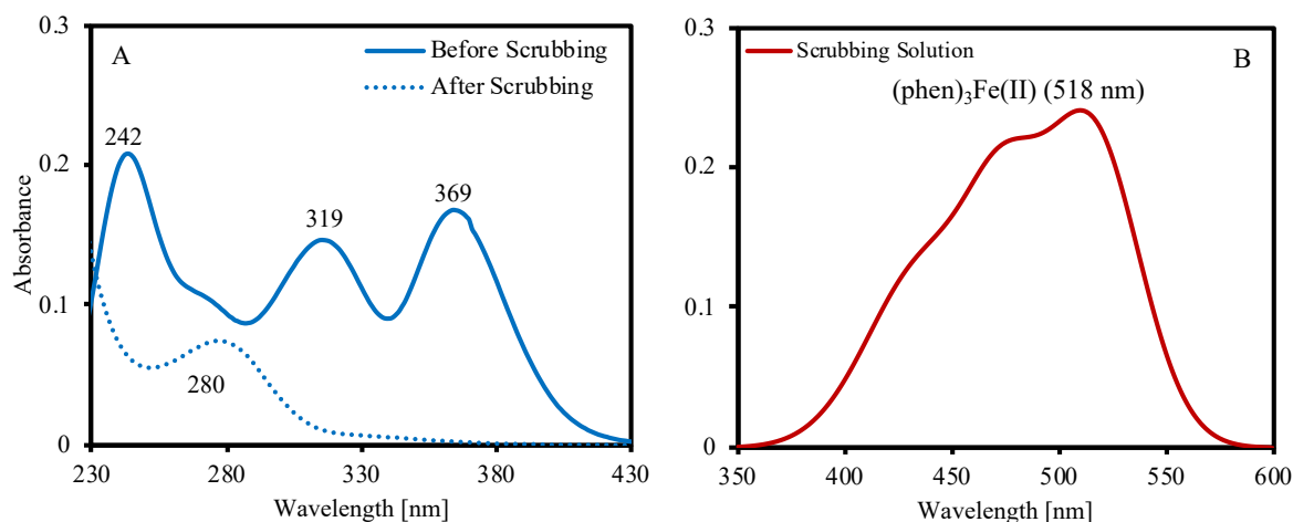
Figure 3.5. UV-visible spectra of (A) iron(III)-chlorocomplexes in P 8,8,8,12 Cl before and after scrubbing with Na 2 SO 3 . Conditions: [HCl] aq = 5 mol L -1 , V aq /V IL = 2. Spectra were acquired in ethanol. (B) iron(II)-phenanthroline complexes from scrubbing solution. Conditions: 1,10-phenanthroline = 0.01 mol L -1
