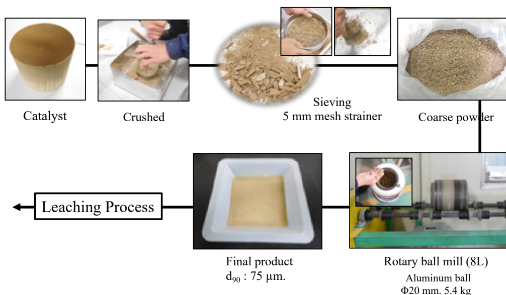
Scheme 4.1. Spent automotive catalyst pre-leaching treatment.
