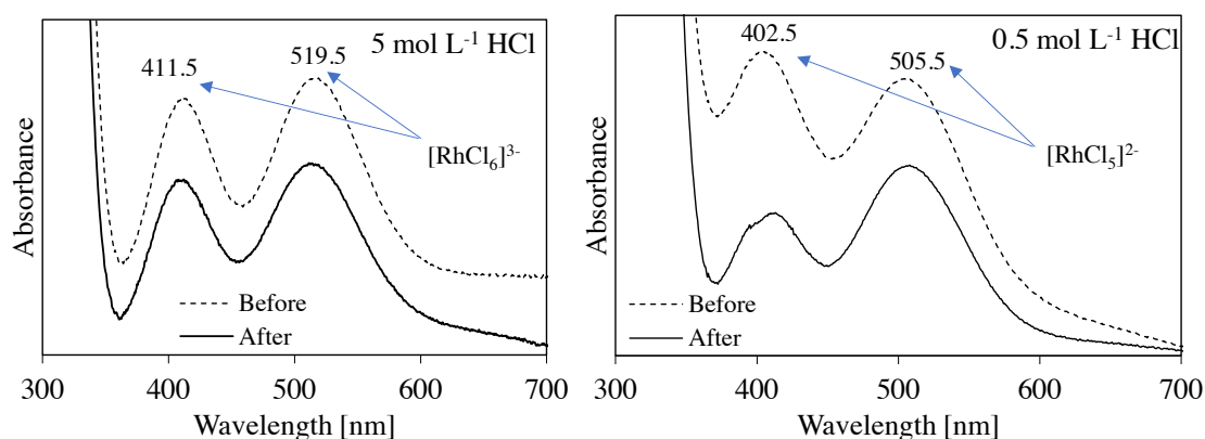
Figure 2.7. UV-vis spectral changes of the chlorocomplexes of Rh(III) in the aqueous phase before and after extraction with P_{8,8,8,12}Cl ; [Rh]_{aq} = 100 \text{ mg L}^{-1} , V_{aq}/V_{IL} = 2 , time = 3 hours.
