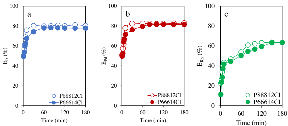
Figure 2.2. Effects of contact time on the Pt(IV), Pd(II), and Rh(III) extraction; [M]_{\text{aq}} = 200 \text{ mg L}^{-1} , V_{\text{aq}}/V_{\text{IL}} = 2 , [\text{HCl}]_{\text{aq}} = 0.5 \text{ mol L}^{-1}
