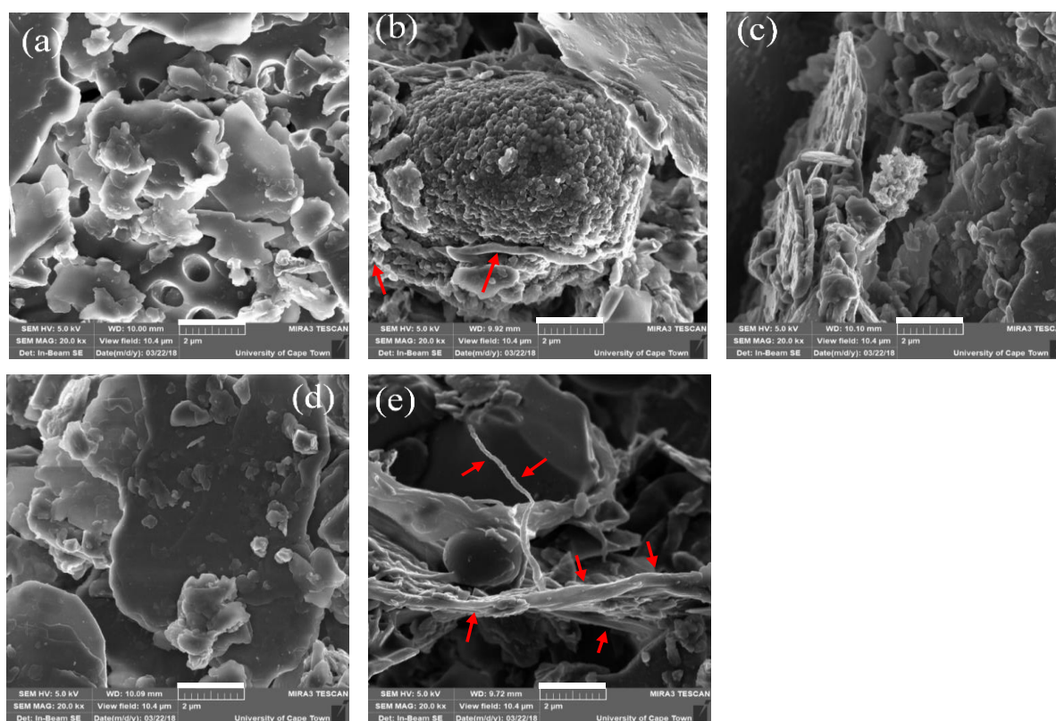
Figure 4. 12 Scanning electron micrographs of the surface of the (a) as-received ore, and the solid residues after treated by (b) CFSM (DC), (c) A. brierleyi (DA), (d) CFSM followed by A. brierleyi (DCA), and (e) A. brierleyi followed by CFSM (DAC). A scale 2µm was used for the analysis. Red arrows in the images clearly highlight the presence of the long thin strands of fungal biomass.
