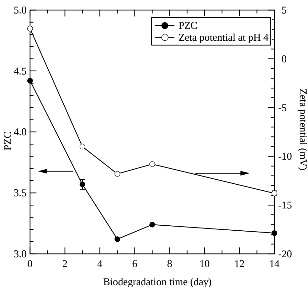
Figure 3. 6 The pH of zero charge (PZC) and zeta potential at pH 4 of pristine PAC and PAC 5 after 3~14 days treatment with CFSM depending on degradation time. The vertical bars represent the standard error of three measurements.
