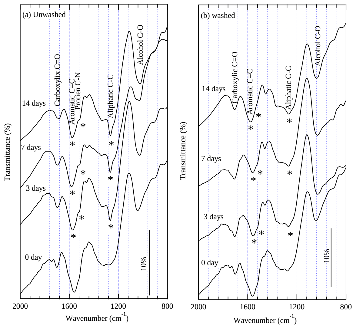
Figure 3. 8 FTIR spectra of pristine PAC and PAC 5 after 3~14 days treatment with CFSM. (a) before and (b) after washing with 2-propanol.
