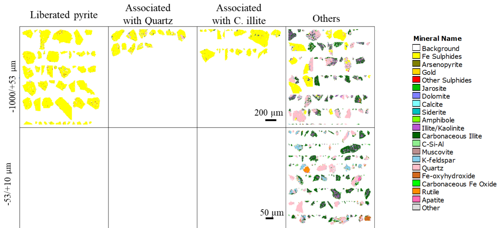
Figure 4.7 QEMSCAN maps of liberated pyrite, pyrite associated with quartz and carbonaceous illite, and others in the solid residues of DRGO after 14 days-treated by A. brierleyi (DA) depending on size fractions ( \mu\text{m} ). Scales of 200 \mu\text{m} and 50 \mu\text{m} was used for the -1000 \mu\text{m} /+53 \mu\text{m} and -53 \mu\text{m} /+10 \mu\text{m} respectively.
