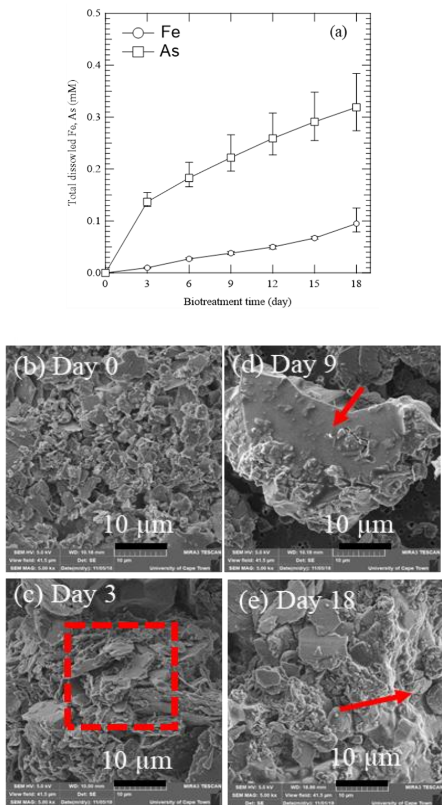
Figure 6. 1 (a) Effect of treatment time on total Fe and As released during CFSM bio-treatment; (b)-(e) Effect of CFSM treatment time on morphology of the as-received sample and DRGO_CFSM as observed by SEM. Scale of 10 \mu m, was used for SEM observation. The
