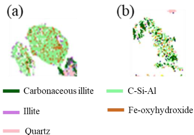
Figure 6. 3 Two types of aggregates produced CFMS only treated DRGO prepared for QEMSCAN analysis using (a) vibrating screening to produce +53 µm and – 53 µm products, followed by ultrasonic-assisted filtering of the – 53 µm products through a 10 µm sieve and (b) only ultrasonic-assisted filtering of the whole sample through a 10 µm sieve.
