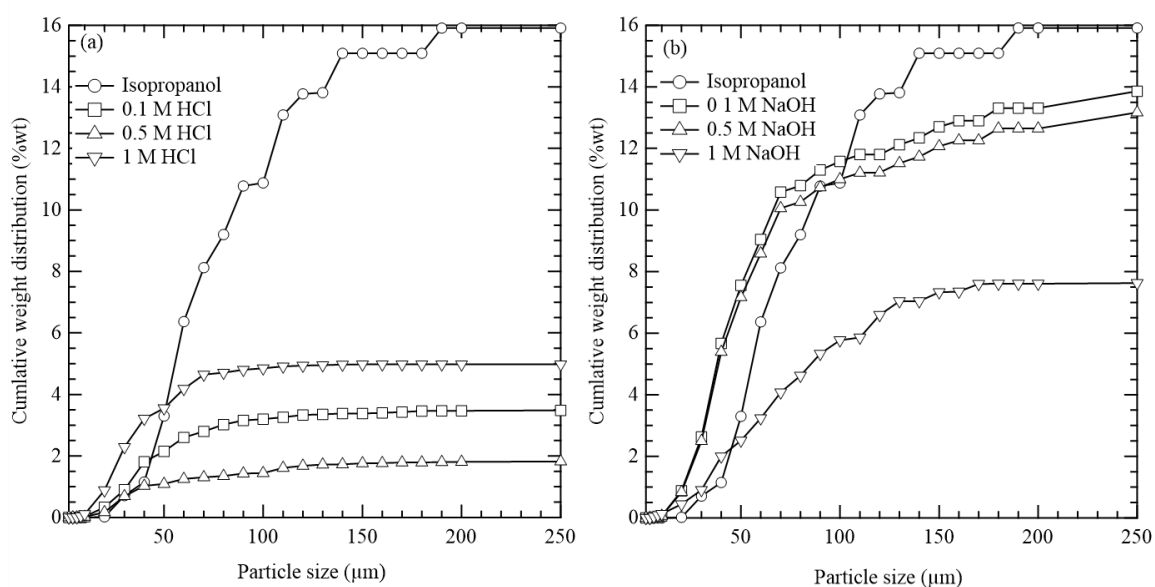
Figure 6. 4 QEMSCAN analysis of the cumulative particle size distribution of larger agglomerates in (a) isopropanol and HCl washed DRGO_CFMS and (b) isopropanol and NaOH washed DRGO_CFMS.
