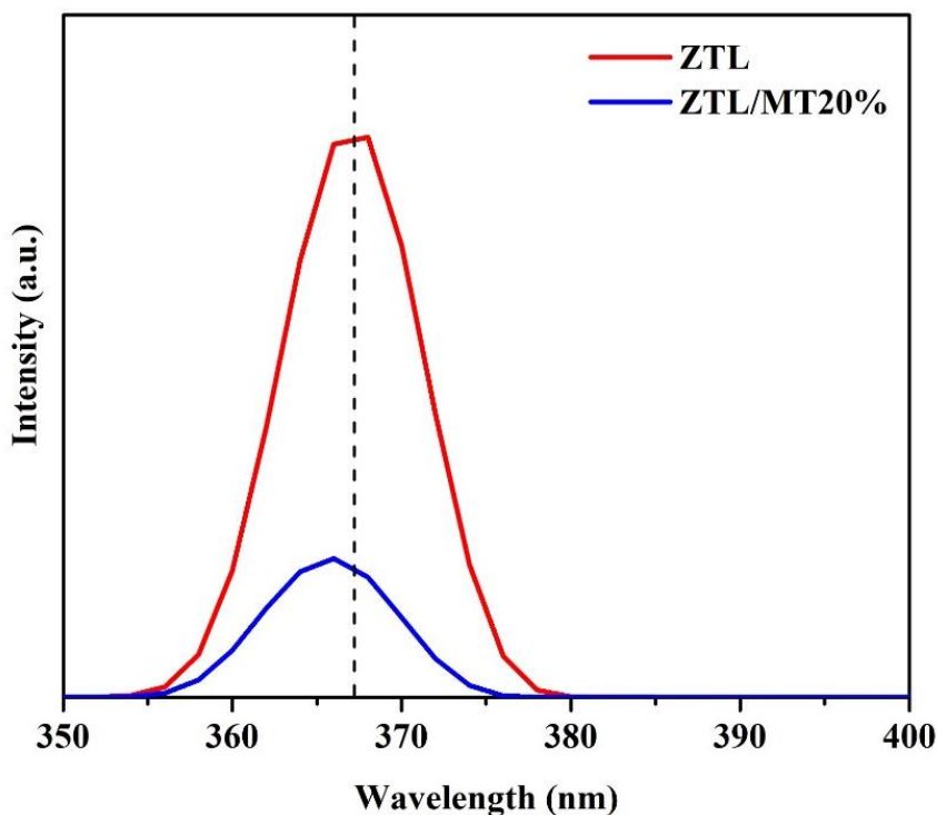
Fig. 3.5 Photoluminescence spectra of ZTL and ZTL/MT20%.
