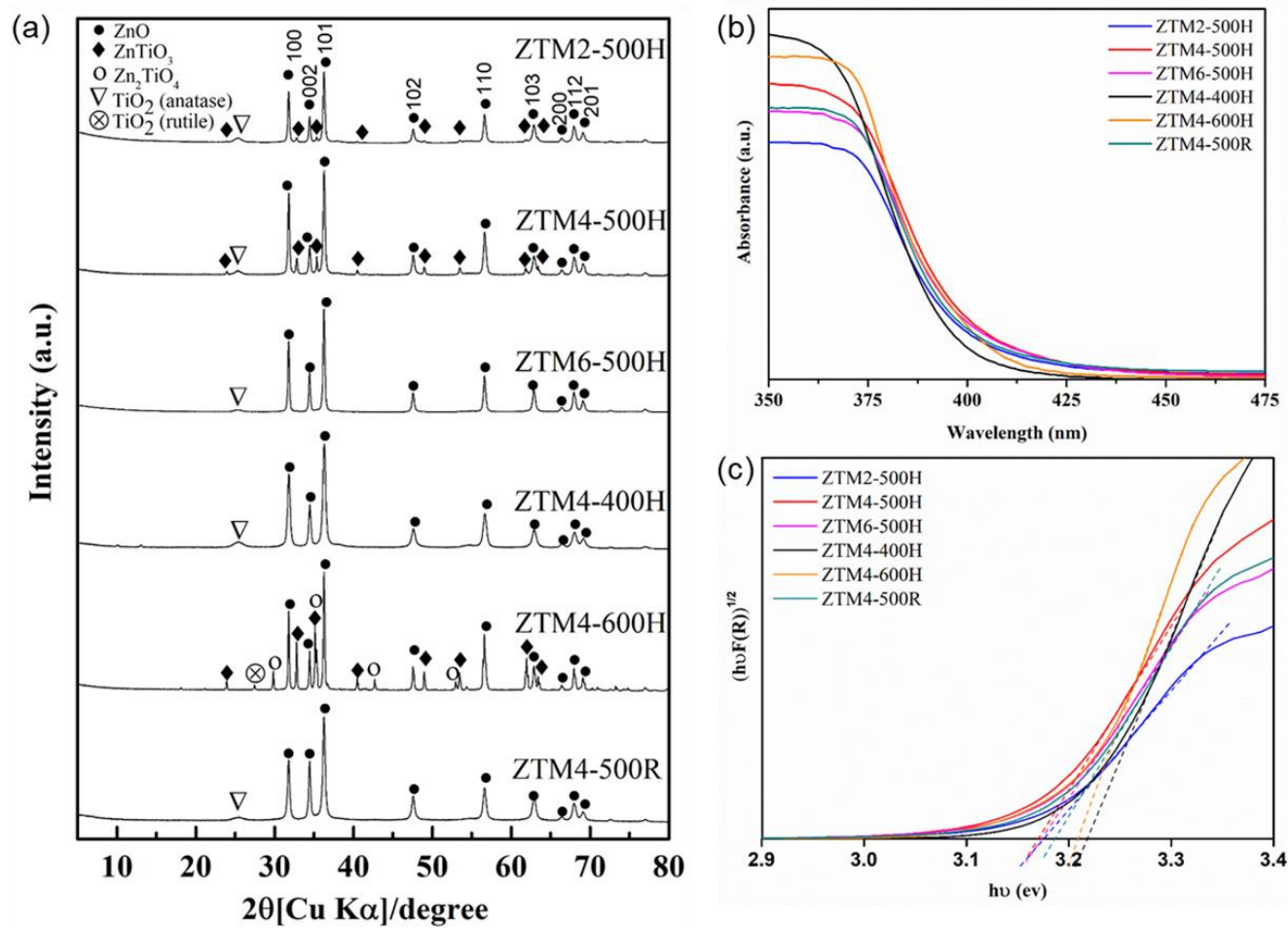
Fig. 4.1 a) PXRD patterns of ZTM samples, b) diffuse reflectance UV-visible spectra of ZTM samples, and c) plots between (\text{hf}(\text{R}))^{1/2} vs. \text{hf} (eV) for ZTM samples.
