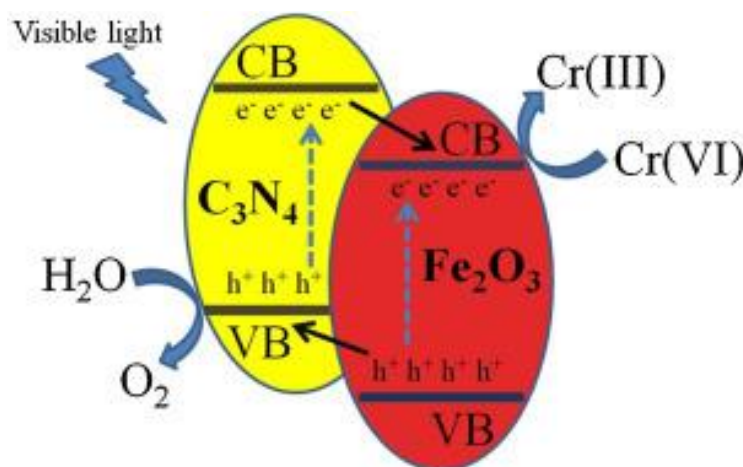
Fig. 1.18 Mechanism for photocatalytic reduction of Cr(VI) [68].
