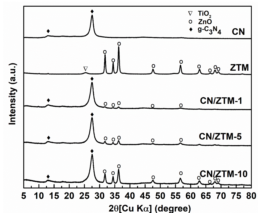
Fig. 6.1 PXRD pattern for CN, ZTM, and CN/ZTM composites.
