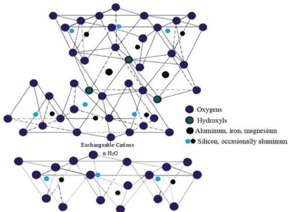
Fig. 1.12 Montmorillonite structure [94].
