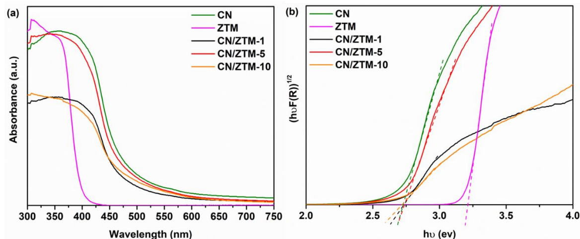
Fig. 6.3 (a) Diffuse reflectance UV-visible spectra and (b) Plots between (\hbar\nu F(R))^{1/2} vs. \hbar\nu (eV) for synthetic samples.
