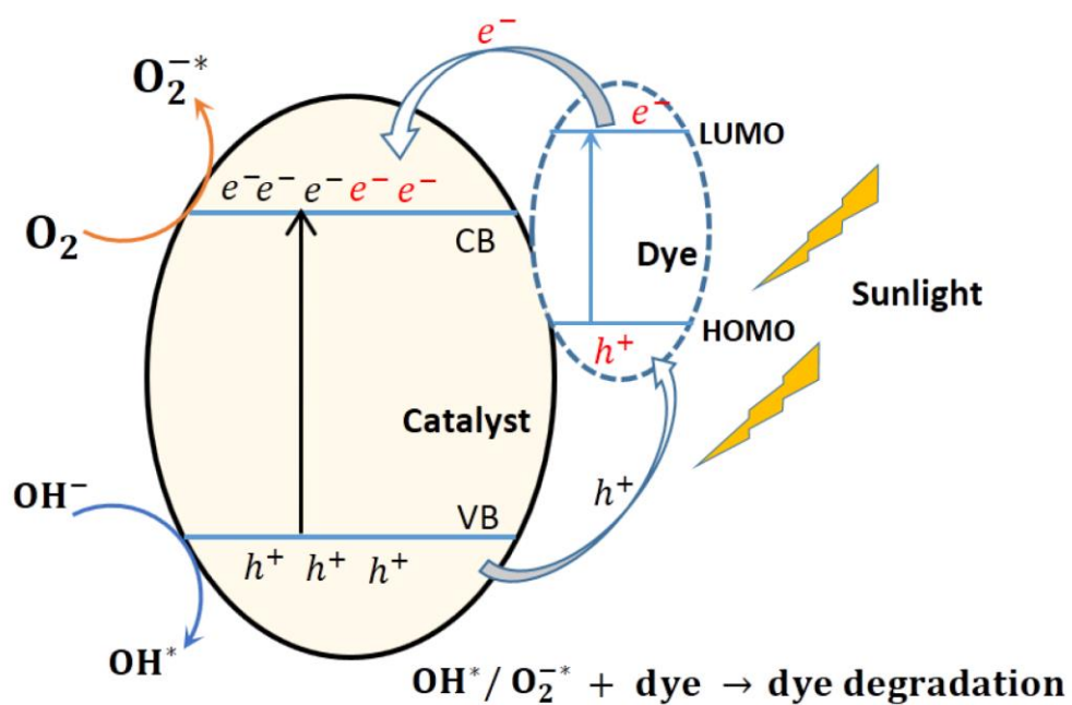
Fig. 1.15 Dye-sensitized visible light photocatalytic mechanism [117].
