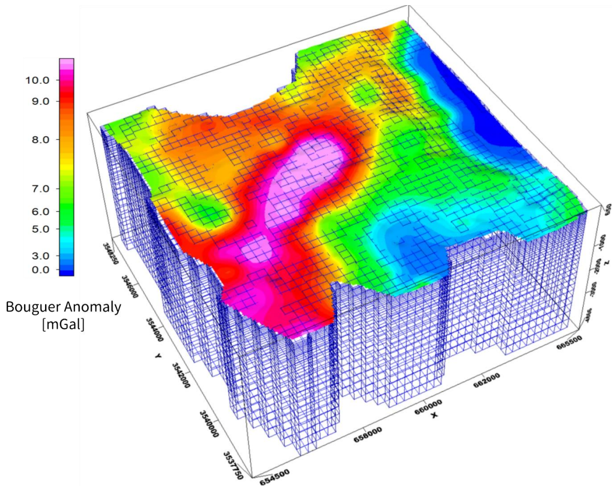
Figure 4-20. A 3-D Gravity inversion grid. The cell size is 250 m \times 250 m \times 50 m (number of cells x , y , z are 42, 41, 38 respectively). The colored map represents Bouguer anomaly (CBA) with values ranging from -2.9 mGal to 11.7 mGal.
