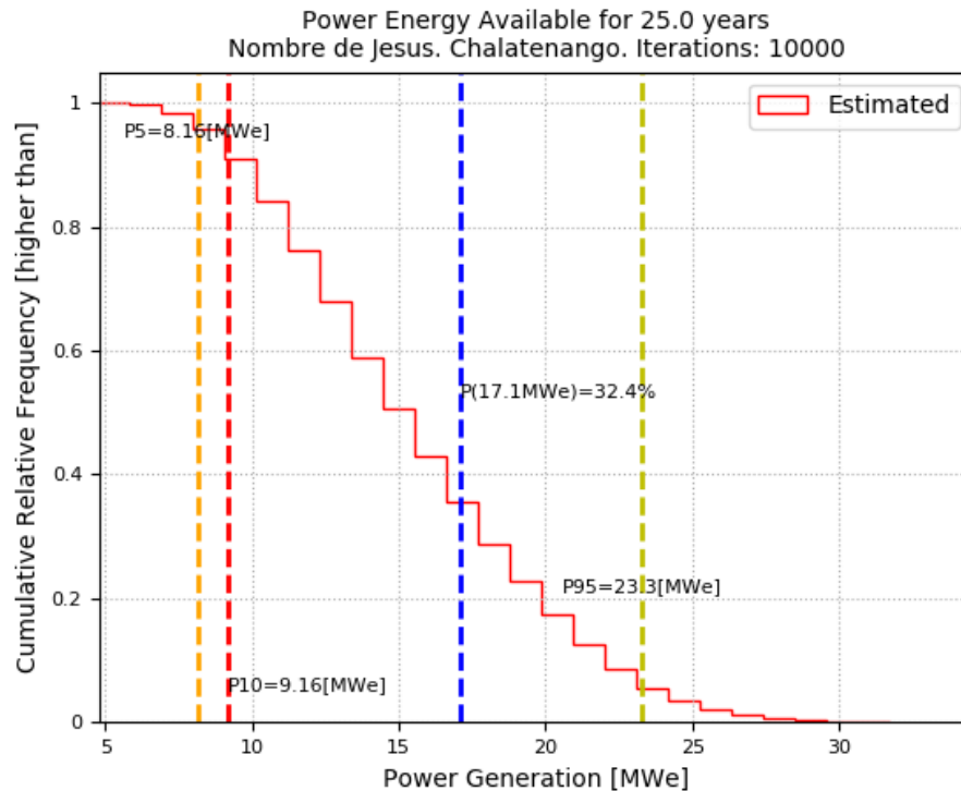
Figure 2-15. Cumulative frequency distribution (CFD) of Nombre de Jesús, El Salvador. This simulation was run for 25 years.
