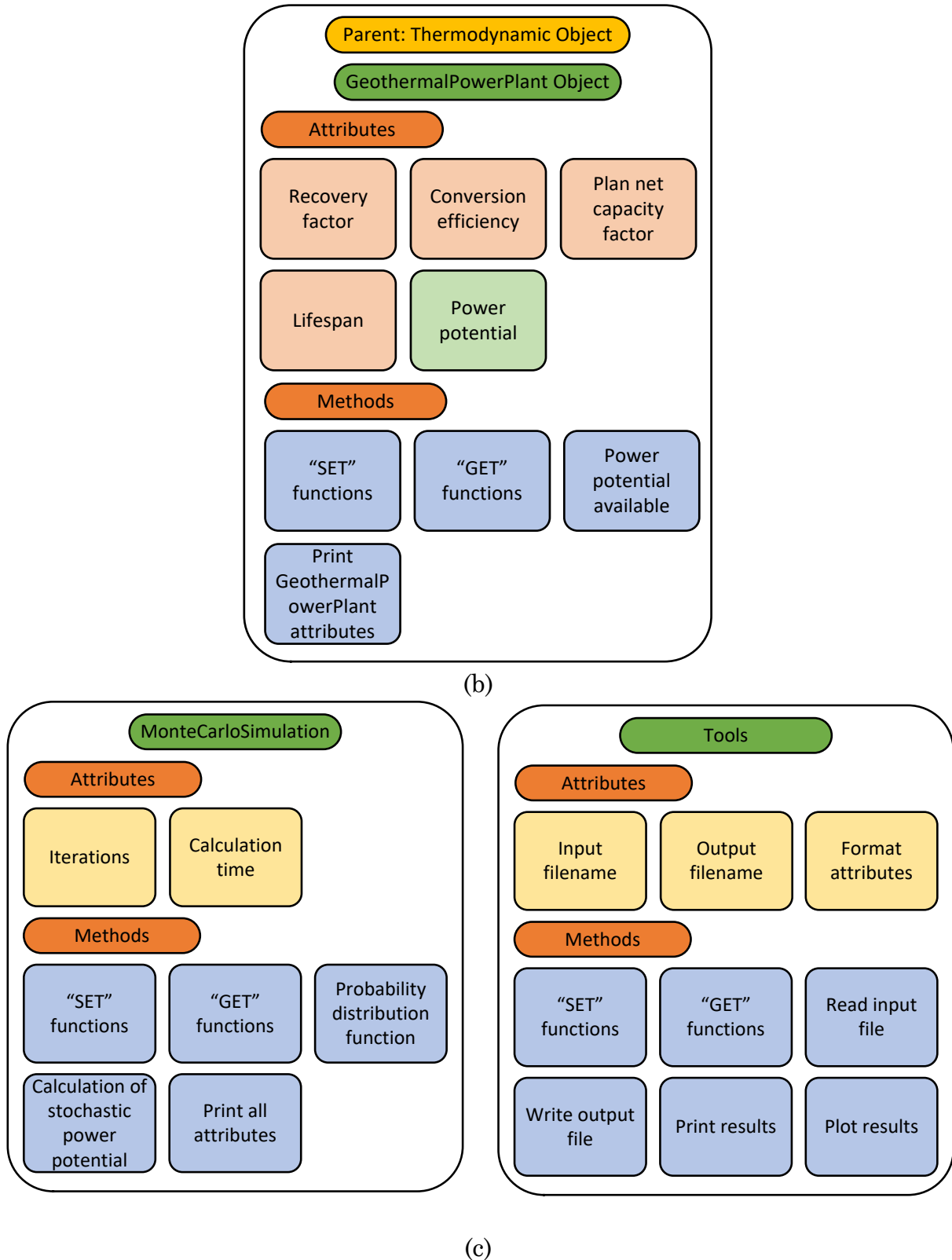
Figure 2-6. Overview of the objects used in the Python-based stochastic library. (a) & (b) Geothermal power plant module, which inherits properties and methods from parent objects (i.e., thermodynamic and reservoir objects). (c) Monte Carlo and tools modules.
