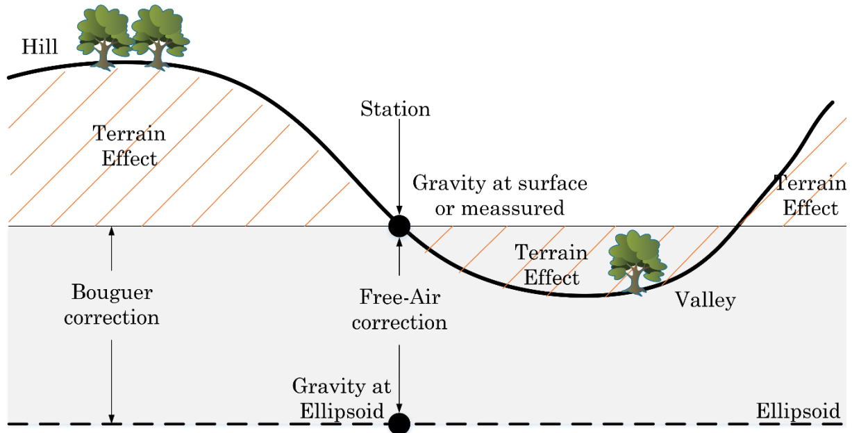
Figure 4-2. Bouguer anomaly calculated at gravity ellipsoid adding Free-Air correction, Bouguer effect, and Terrain correction (Saibi et al., 2007).
