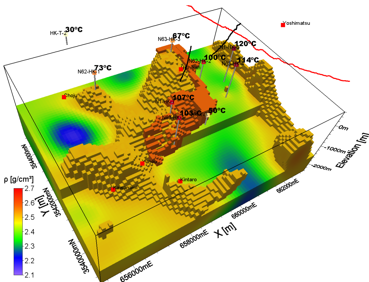
Figure 4-21. 3-D inversion model grid. The brown structure located aside of the high dense body in the center might be the hydrothermal reservoir with the volume of about 0.93 \text{ km}^3 , and an average block density value of 2.45 \text{ g/cm}^3 . The grid is plotted using Voxler 3-D program (Golden Software LCC, 2018).
