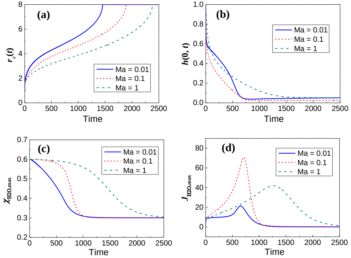
Figure 7.12 Evolution of (a) contact line position, (b) droplet height, (c) maximum water concentration, and (d) maximum mass flux for different Marangoni numbers of 0.01, 0.1, and 1. ( \chi_{H_2O} = 60\% , RH = 30\% .)
