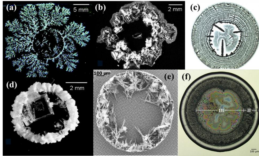
Figure 2.2 Examples of the crystalline patterns formed from drying aqueous saline solution droplet. (a) Saturated \text{NaSO}_4 droplets on a hydrophilic glass substrate. [104] (b) Saturated \text{NaCl} droplets on a hydrophilic glass substrate. [104] (c) Aqueous solution droplet of 0.5 g/l \text{NaPSS} and 0.1M salt on a hydrophilic glass substrate. [107] (d) Saturated \text{NaCl} droplets on a hydrophobic substrate. [104] (e) Droplet of saturated \text{CaSO}_4 solution on a superhydrophobic surface. [106] (f) Droplet of 1.0 wt.% lysozyme + 0.1 wt.% \text{NaCl} solution on a hydrophilic silicon wafer. [108]
