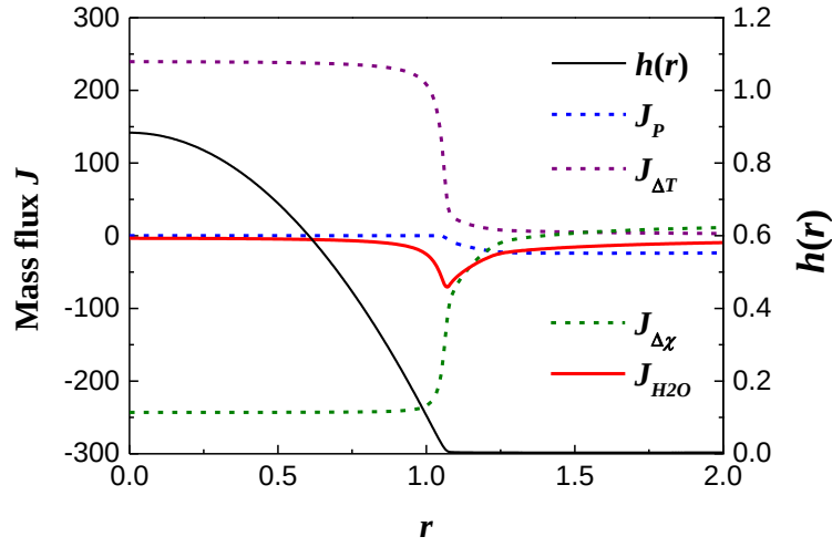
Figure 7.9 Distribution of decomposed mass fluxes along with droplet profile, at the moment of t = 65 s. ( \chi_{\text{H}_2\text{O}} = 60\% , RH = 90%.)
