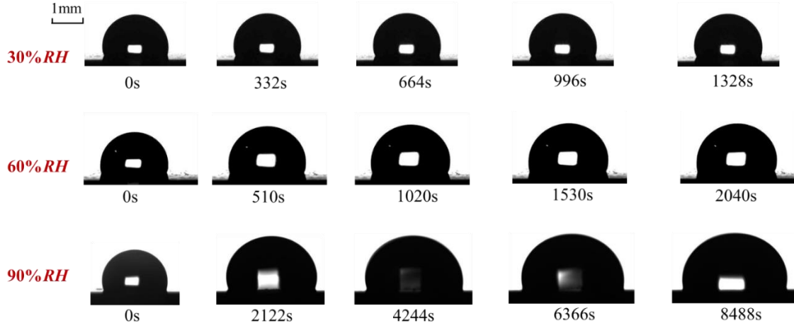
Figure 5.1 Profile evolution of LiBr-H 2 O droplets during vapor absorption for ambient condition of 45°C and 30% RH, 60% RH, 90% RH, for \tau = 0, 0.25, 0.5, 0.75 and 1.
