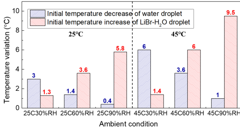
Figure 5.7 Initial temperature increase of LiBr-H 2 O droplet caused by absorption heating (red columns), and temperature decrease of pure water droplet caused by evaporation cooling (blue columns) for the six experimental conditions.
