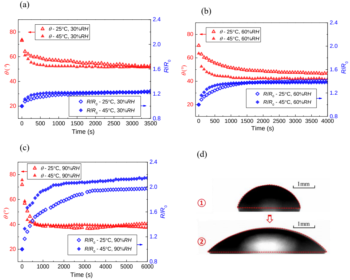
Figure 4.1 Evolution of (up-triangles) contact angle, \theta (°), and (diamonds) normalized contact radius, R/R_0 , of LiBr-H 2 O droplets, versus time (s) for (a) 30% RH , (b) 60% RH , and (c) 90% RH , at (open symbols) T_{amb} = 25^\circ C and (close symbols) T_{amb} = 45^\circ C on hydrophilic glass substrates. (d) Initial ( t = 0 s) and final ( t = 6000 s) snapshots of a LiBr-H 2 O droplet on a hydrophilic glass substrate at 45^\circ C and 90% RH .
