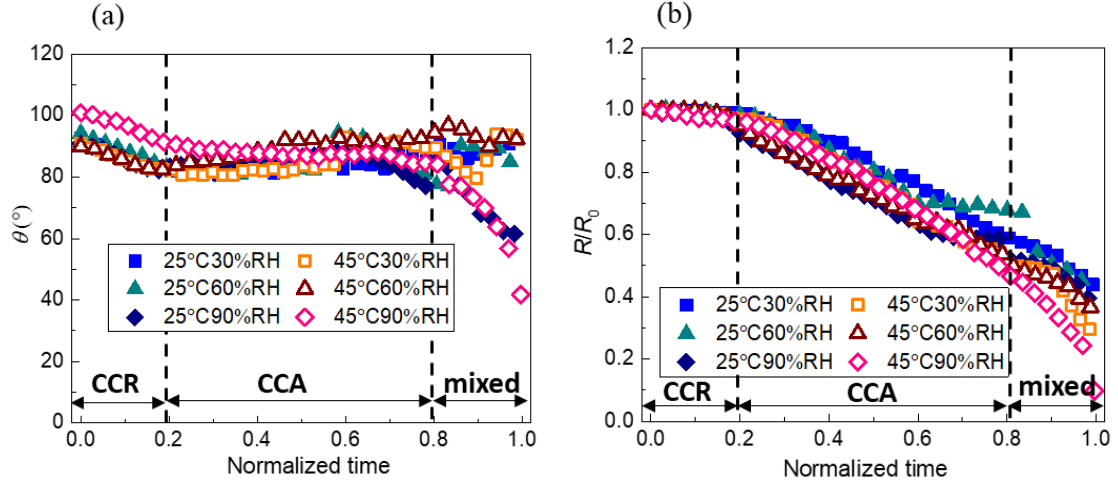
Figure 5.4 Evolution of (a) contact angle \theta , and (b) non-dimensional contact radius R/R_0 of pure water droplets, versus non-dimensional time, \tau (s) for (closed symbols) T_{\text{amb}} = 25^\circ\text{C} and (open symbols) T_{\text{amb}} = 45^\circ\text{C} at (square) 30% RH, (up-triangles) 60% RH, and (diamonds) 90% RH on smooth PTFE.
