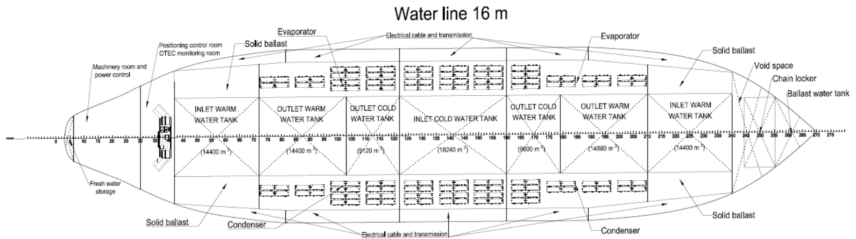
Figure II.22 Top view at waterline of 16 m for case two Top view
