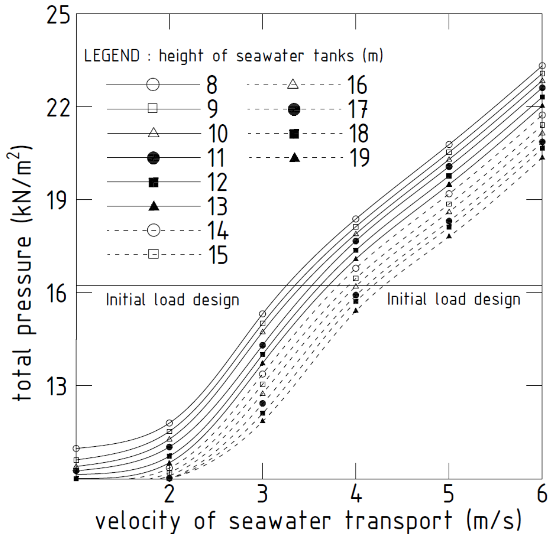
Figure II.14 Total pressure acting on the top part of seawater tank
