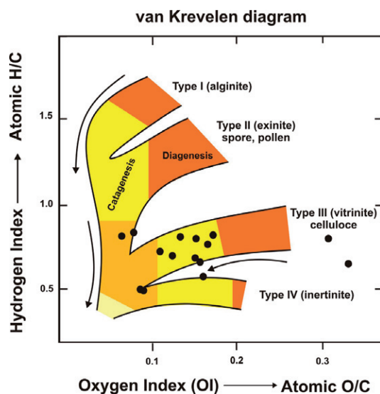
Fig. 4 van Krevelan diagram Oxygen Index (OI) against Hydrogen Index (HI), showing the hydrogen generative type, and most samples plot in the Type III (gas prone).
