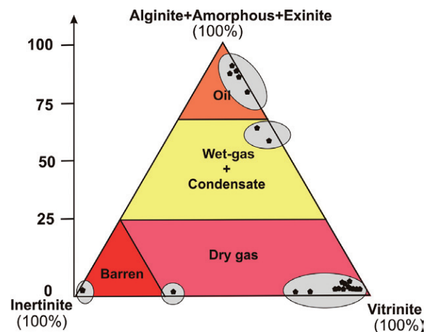
Fig. 5 Samples distribution of visual kerogen analyses and most samples fall in dry-gas, almost up 70% 10 .
