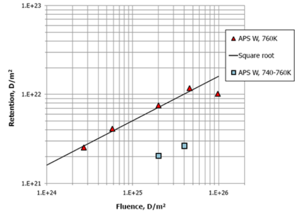
Fig.5 Fluence dependence of D retention in APS W exposed to D plasma at 760 K (triangles). The repetitive points are shown by squares, the square root behavior is shown by the line
