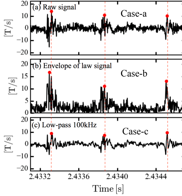
FIG. 3.14: Different three proceeded signals, (a) Raw signal, (b) envelope of the raw signal, and (c) low-pass 100 kHz signal are prepared for the verification study. For threshold method, thresholds are defined as 10, 10 and 7 T/s, respectively. The red points indicate the local peaks, where the timing are defined as clocks.
