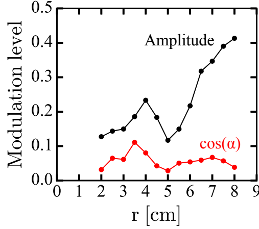
FIG. 4.18: Modulation level of amplitude and phase of particle flux. The modulation level is defined as root-mean-squared of fluctuation part of amplitude and phase, where the amplitude is normalized by its mean values.
