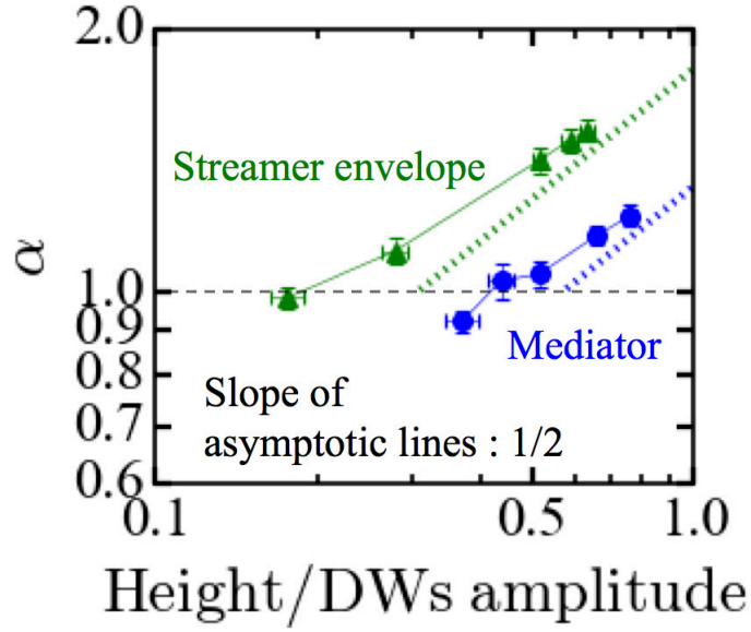
FIG. 4.11: Dependence of anharmonicity \alpha on the normalized height is shown as a double logarithmic plot. The slope of asymptotic lines is 0.5, which indicates that height converges proportionally to \alpha^2 .
