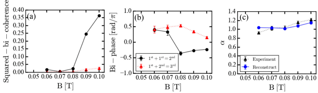
FIG. 4.12: Magnetic field dependence of the (a) squared-bi-coherence and (b) bi-phase of the components of mediator. The ensemble number is 150. Reconstruction of the mediator is performed by bi-phase analysis. The anharmonicities \alpha of the mediator for the observed (black) and reconstructed (blue), which is performed by bi-phase analysis, are shown in (c). A good agreement with experimental observation can be seen.
