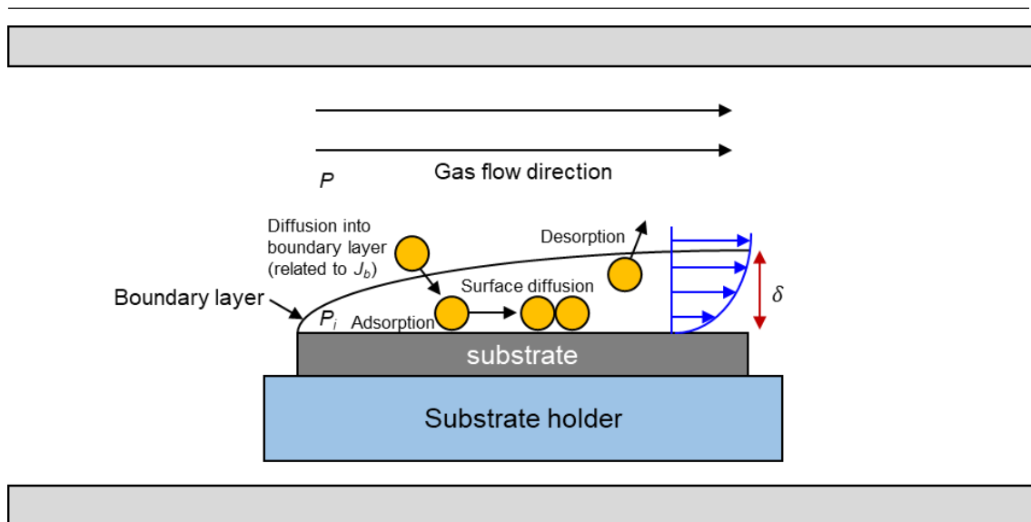
Figure 3-22 Behavior of gaseous molecules in the tubular CVD reactor.
