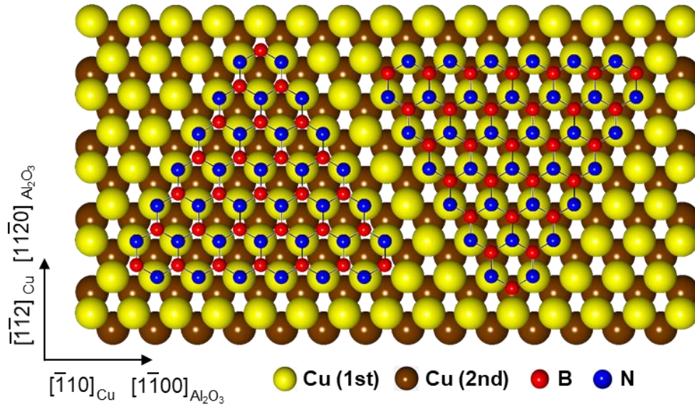
Figure 4-4 Atomic model of triangular grains of h-BN on Cu(111). Left and right configurations correspond to (N_{\text{top}}, B_{\text{fcc}}) and (N_{\text{top}}, B_{\text{hcp}}) , respectively. The orientations of c-plane sapphire and Cu are indicated by arrows.
