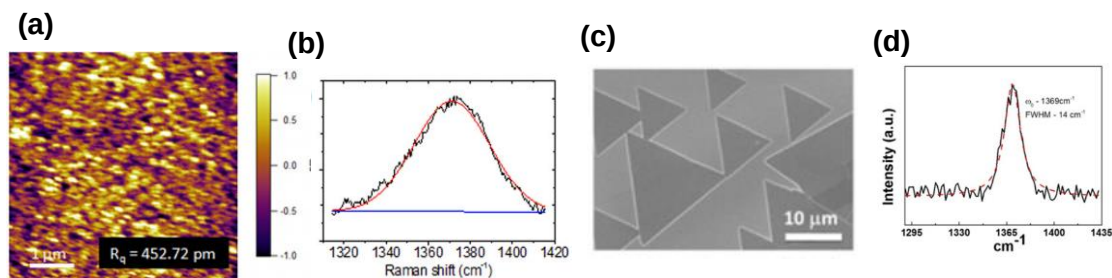
Figure 3-18 AFM image (a) and Raman spectrum (b) of h-BN nanocrystals grown on SiO 2 . 42 SEM image (c) and Raman spectrum (d) of h-BN grown on Cu foil. 43
