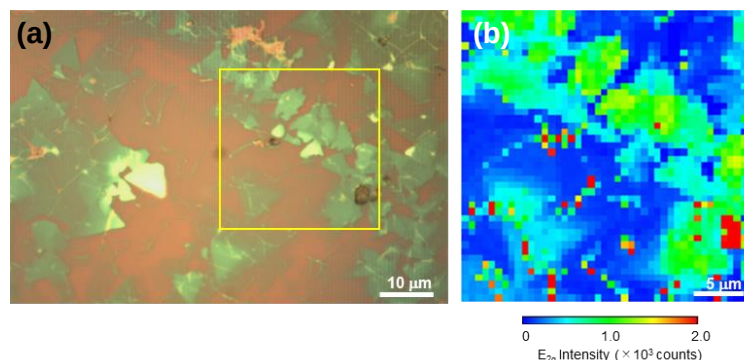
Figure 5-3. h-BN grown on the Fe foil. Optical microscope (a) and Raman E_{2g} intensity mapping (b) images of the transferred h-BN. The Raman mapping was measured at the marked area shown in (a). Total 1600 spectra were collected from the 30\ \mu\text{m} \times 30\ \mu\text{m} square area (no pixel smoothing process was applied).
