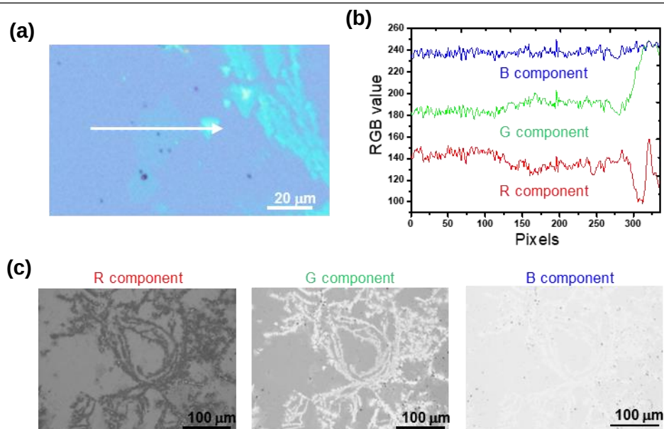
Figure 5-10. (a) Optical microscope image of h-BN grown on the Fe foil after the transfer on a \text{SiO}_2/\text{Si} substrate. (b) Intensity of RGB components measured along the white arrow in (a). The G component reflects the optical contrast of the h-BN. (c) Optical microscope image made only from the R, G, and B components. The original optical image is shown in Figure 5-7d.
