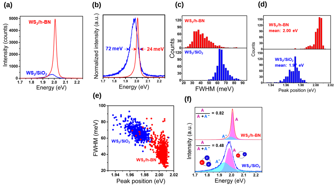
Figure 5-12. (a) Representative PL spectra of the WS 2 grown on h-BN (red) and SiO 2 /Si (blue) substrates. (b) Normalized PL spectra. (c,d) Distributions of the PL linewidth and PL peak position (total number of collected spectra is >600 for each sample). (e) Relationship between the PL linewidth and peak position. (f) Curve-fitted PL spectra of WS 2 on h-BN (upper) and SiO 2 /Si substrate (lower). Pink and light blue peaks represent exciton (A) and charged exciton (A - ), respectively. The A/(A+A^-) ratio is calculated from the peak areas.
