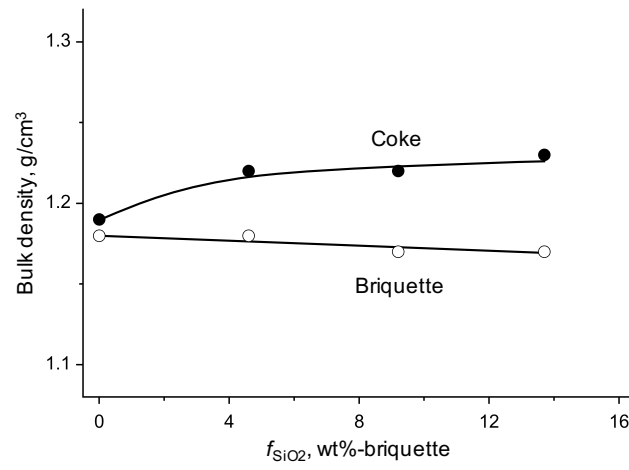
Fig. 3. Effects of f_{\text{SiO}_2} on bulk densities of briquette and coke.
