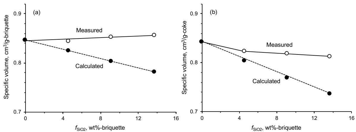
Fig. 4. Effect of f_{\text{SiO}_2} on specific volume of (a) briquette and (b) coke.
