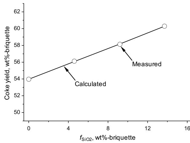
Fig. 1. Effect of f_{\text{SiO}_2} on coke yield. Plot; measured yield, solid and straight line; calculated yield.
