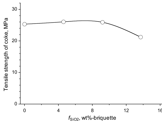
Fig. 2. Effect of f_{\text{SiO}_2} on tensile strength of coke.
