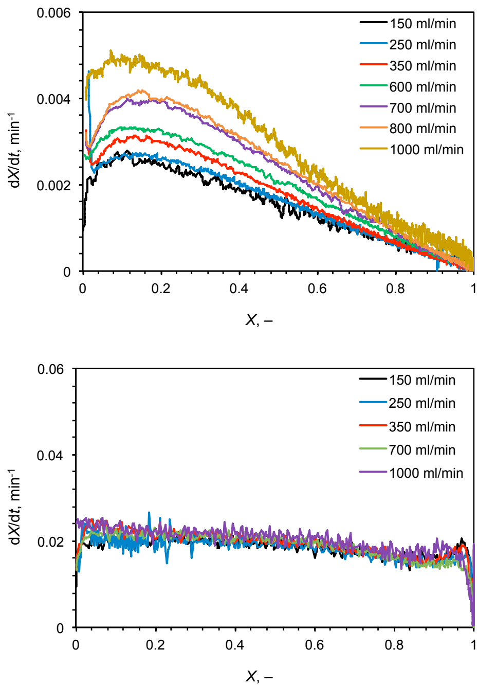
Fig. 8. Profiles dX/dt vs X of ALY (top) and LY (bottom) char gasification at different flow rates. The particle size is 106 \mu\text{m} or smaller, and the initial mass is 1.3 mg.
