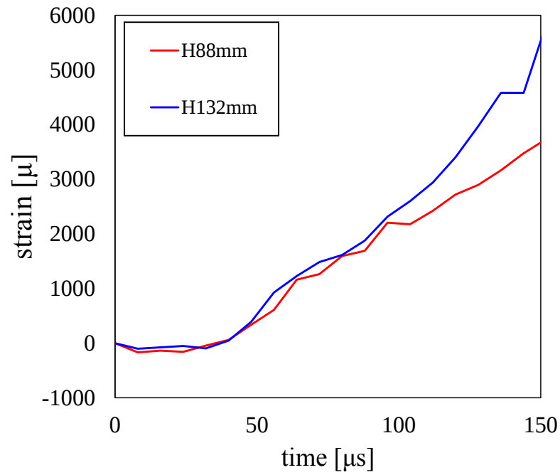
Fig. 2.22 The strain profiles of \epsilon_{xx} on the cracks at Point A3
