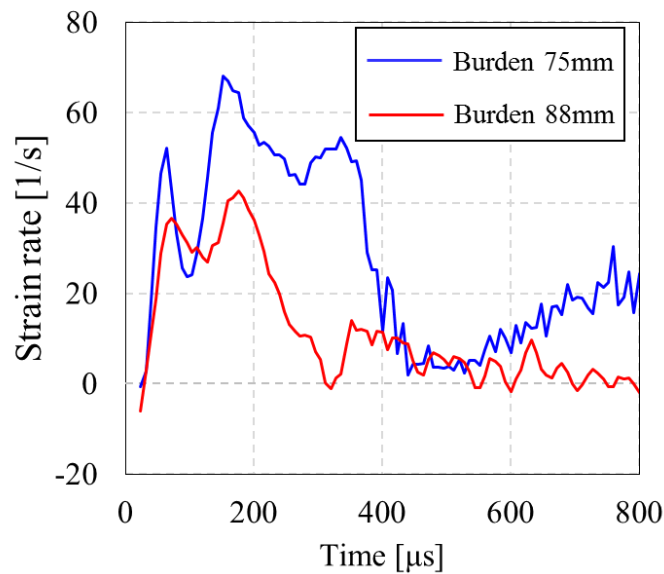
Fig. 2.19 The strain rate profiles of \epsilon_{xx} on the cracks at Point A2
