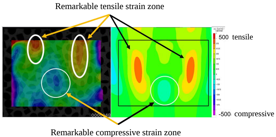
Fig. 3.2 Comparison of horizontal strain distribution at 50 [ \mu s] (a) Small-scale blasting experiment (b) Numerical simulation (same contour scale)
