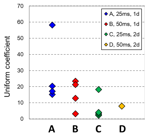
Fig. 5.18 Uniformity coefficient in each firing pattern
