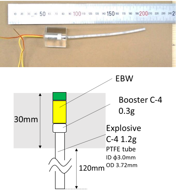
Fig. 2.9 Outline of mortar block and blasting designs
