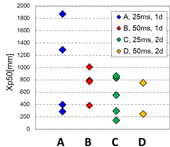
Fig. 5.19 The relationship between firing pattern and Xp50
