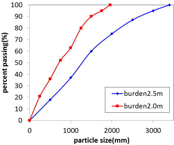
Fig. 5.8 Particle size distribution curve of fragmentation at burden of 2.5 m and 2.0 m
