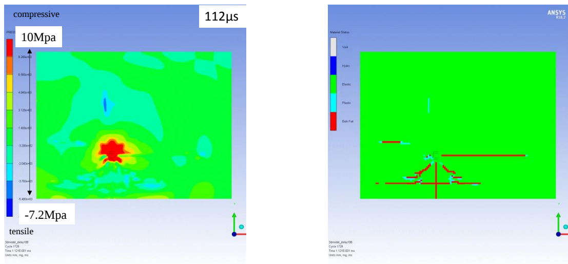
Fig. 3.8 Stress wave and crack propagation behavior inside rock mass in the case of 72 \mu s of delay time (a) pressure contour and (b) crack conditions
