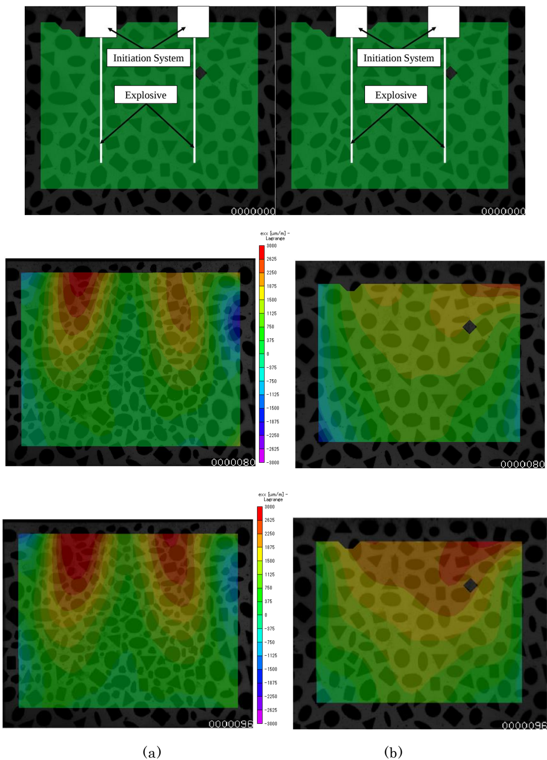
Fig. 2.17 The time history of stain distribution of \epsilon_{xx} at 0 \mu s , 80 \mu s , and 96 \mu s (a) Burden: 75 mm and (b) Burden: 88 mm
