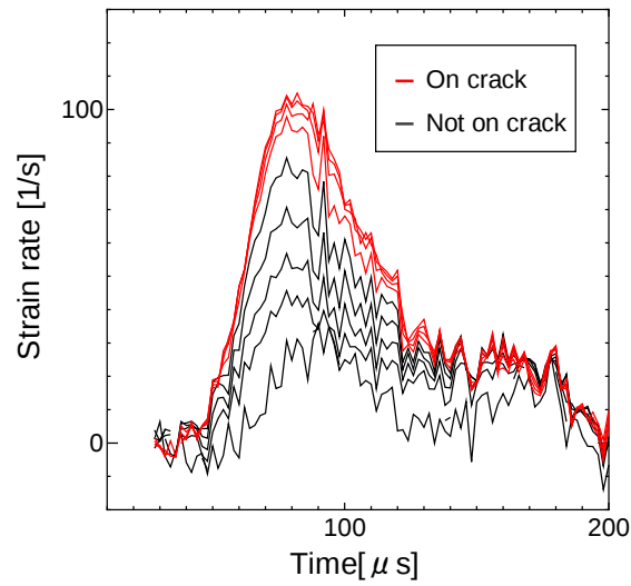
Fig. 2.8 Strain rate history of \epsilon_{yy} at 10 points on line AB (15 moving average)
