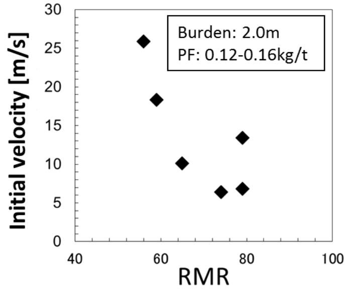
Fig. 4.6 The relationship between RMR and maximum initial velocity of blast-induced fragmented rocks under similar blasting designs
