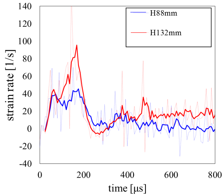
Fig. 2.23 The strain rate profiles of \epsilon_{xx} on the cracks at Point A3
