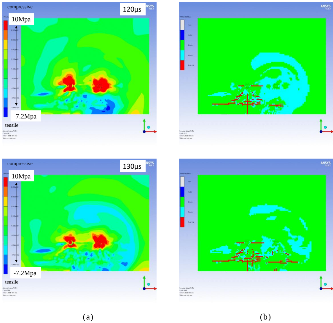
Fig. 3.8 Stress wave and crack propagation behavior inside rock mass in the case of 72 \mu s of delay time (a) pressure contour and (b) crack conditions
