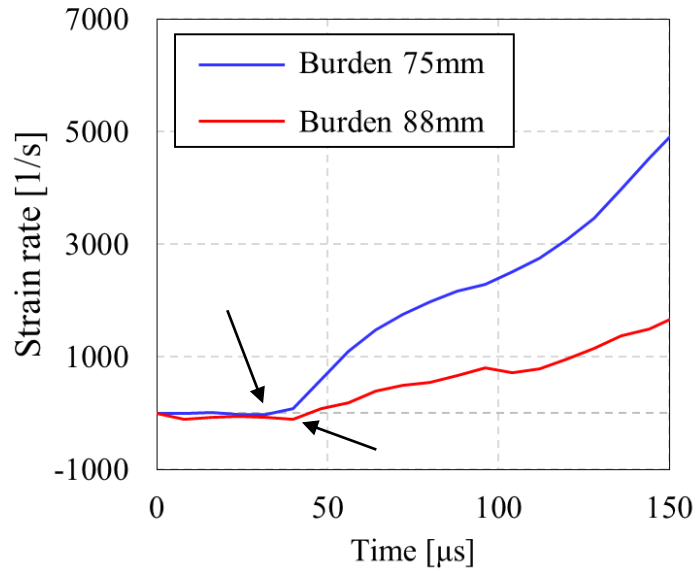
Fig. 2.18 The strain profiles of \epsilon_{xx} on the cracks at Point A2
