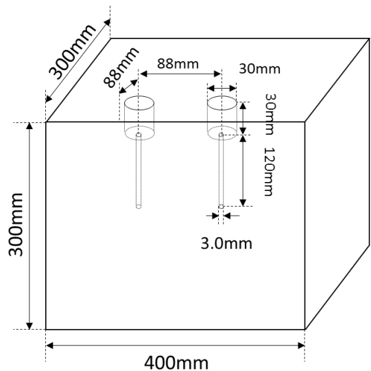
Fig. 2.9 Outline of mortar block and blasting designs
