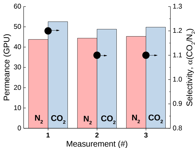
Figure 2-7. Gas permeance property of the PVA/ \text{TiO}_2 multilayer nanomembrane.
