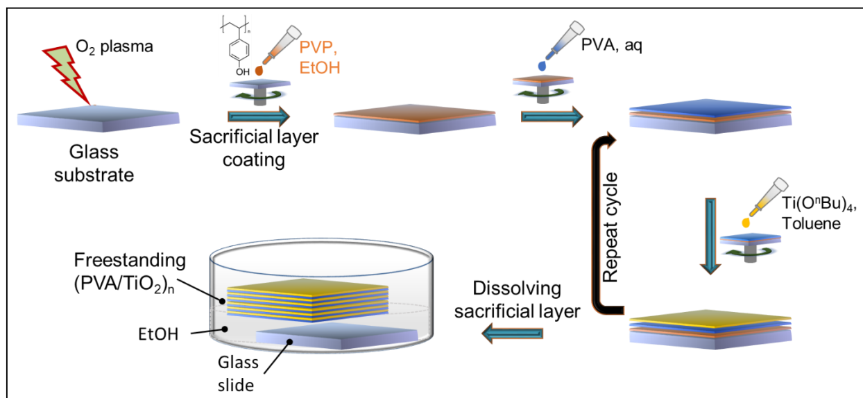
Figure 2-2. Schematic representation of nanomembrane fabrication process by spin-assisted LBL assembly.
