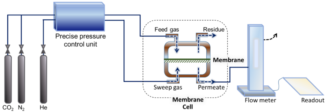
Figure 3-4. Single gas permeation measurement apparatus. The flow rate of \text{CO}_2 and \text{N}_2 was measured separately and transformed into permeance. Helium was used as a sweep gas in both cases. The feed gas volume and pressure conditions were set at 100 sccm and 0.2 MPa, respectively.
