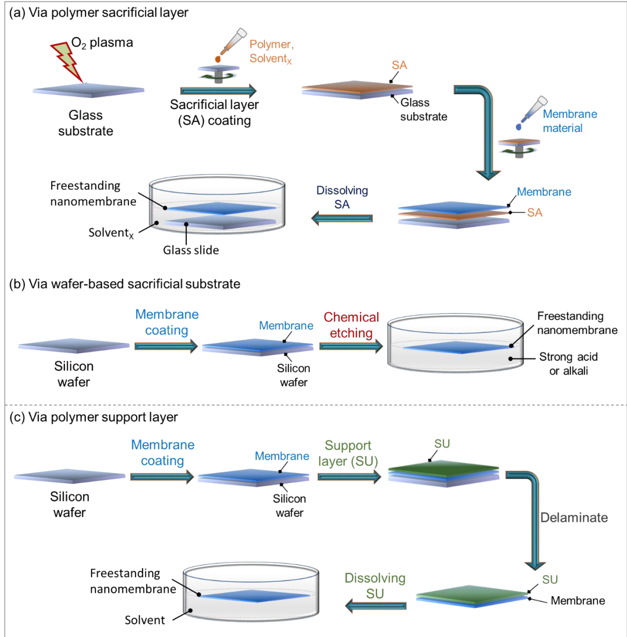
Figure 1-1. Schematic illustration of FS-NM preparation procedures. (a) Via polymer sacrificial layer: it is a commonly used approach, and applicable to the majority of nanomembrane deposition techniques. (b) Via wafer-based sacrificial substrate: it is generally used for the preparation of polymeric FS-NMs which are stable in strong acid/alkaline solution. (c) Via polymer support layer: it is often utilized in the fabrication of metallic and metal oxide FS-NMs. In the current study, polymer sacrificial layer approach using poly(4-vinyl phenol) was employed.
