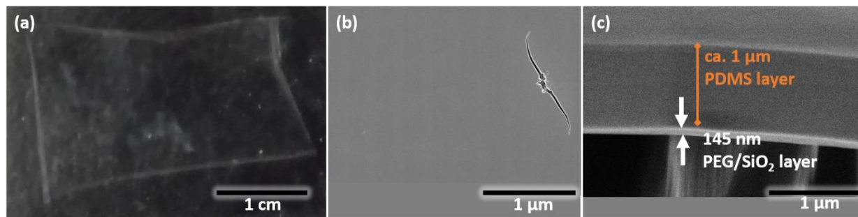
Figure 1-5. (a) Digital image of the nanomembrane in the detachment solvent. (b,c) SEM image of bare PEG/SiO 2 nanomembrane transferred onto a porous support; (c) after caulking layer coating to prevent leakage during gas separation experiment. Scale bar
