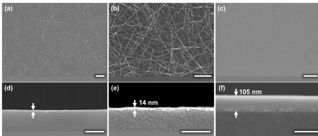
Figure 4-8. SEM observation of morphological changes during the nanomembrane preparation process, Scale bar: 200 nm. (a) Bare ASNTs. (b) Crosslinked ASNTs network structure after 10 cycles of alternate ASNT and \text{TiO}_2 coating steps, i.e., (\text{A-T})_{10} . (c) Film surface became smooth following PDMS coating on (b), i.e., (\text{A-T})_{10}/\text{PDMS} . (d-f) Cross-sectional view of (a), (b) and (c) respectively. All images were recorded on PVP sacrificial layer before membrane detachment.
