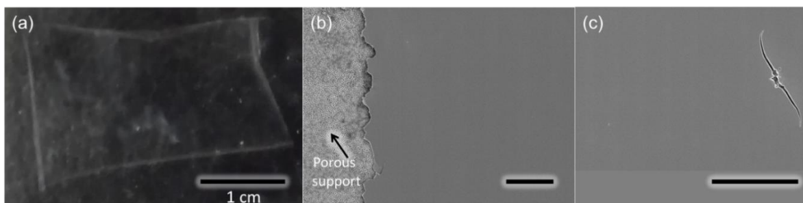
Figure 3-7. (a) Digital image of the PEG-OH/SiO 2 nanomembrane while it was in the detachment solvent. (b,c) SEM image of the nanomembrane transferred onto a porous support. Scale bar: 10 μm.
