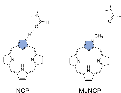
Figure 2-7. The interaction between NCP and DMF molecule through hydrogen bonding (left), and no interaction between MeNCP and DMF molecule (right).
