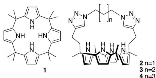
Figure 1-20. Structures of the calix[4]pyrroles 1-4 used in the selective fluoride binding. 31a
