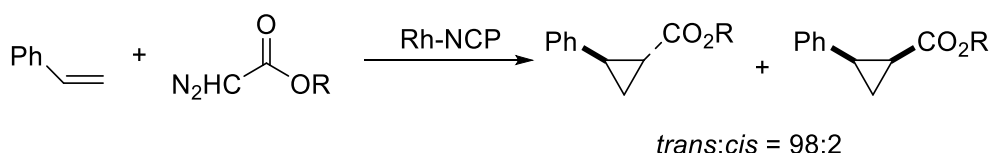
Scheme 1-4. The catalytic reaction using NCP-Rh complex as the catalyst. 47
