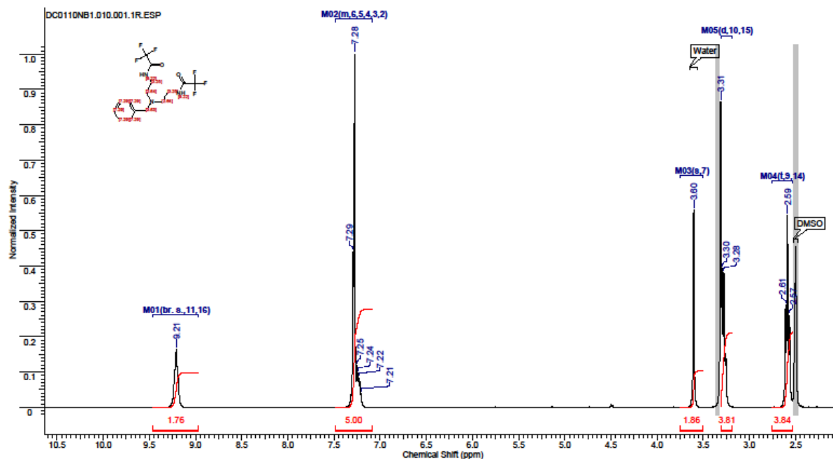
Figure 4-10. 1 H NMR (300 MHz) spectrum of 4 in DMSO- d 6 .
