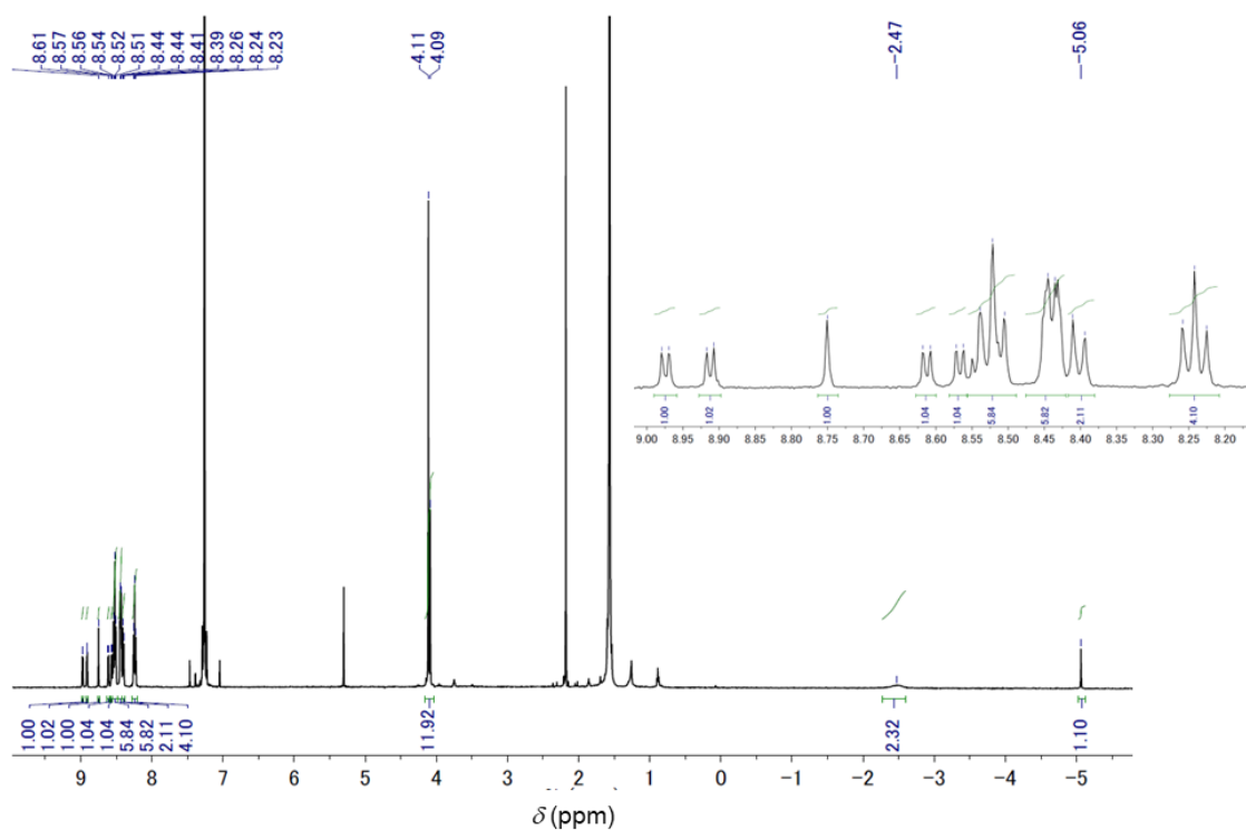
Figure 2-13. 1 H NMR spectrum (500 MHz) of NCTPP ( 1 ) in CDCl 3
