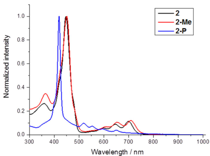
Figure 2-18. UV/vis spectra of NCP ( 2 , black), MeNCP ( 2-Me , red), and TPP ( 2-P , blue) in DMF.
