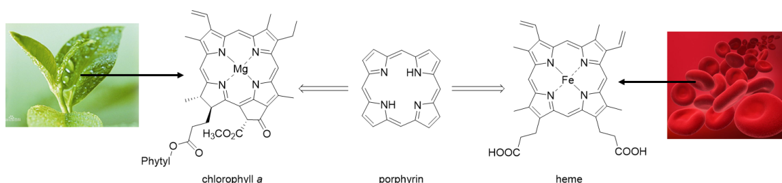
Figure 1-13. The structure of porphyrin (middle), heme (right) and chlorophyll a (left).
