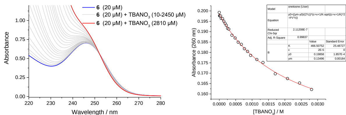
Figure 4-29. UV-vis titration of 6 (20 \mu\text{M} ) with \text{TBANO}_3 (0–2810 \mu\text{M} ) in \text{CH}_3\text{CN} at 298 K.
