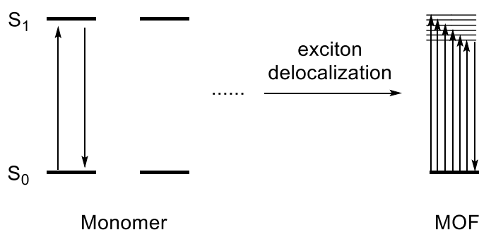
Figure 2-12. In MOFs, delocalization of exciton leads to the merge of ligand energy bands, which then causes the broadening and bathochromic shift of absorption and emission spectra.
