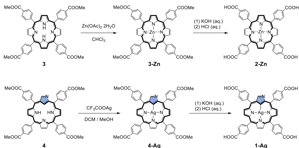
Scheme 3-2. Organic ligands synthesized in this Chapter.
