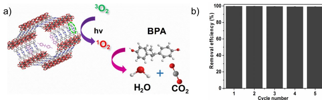
Figure 1-22. a) The proposed mechanism of photodegradation of BPA by ^1\text{O}_2 with PCN-222; b) Removal efficiency of BPA after five-time photocatalysis. 38
