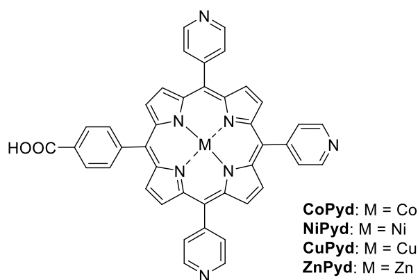
Figure 1-17. Structures of MPyds . 24
