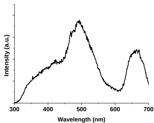
Figure 2-19. The excitation spectrum of the aqueous suspension of MeNCP MOF under probing at 850 nm. Below the wavelength at 700 nm, the spectrum is not corrected.
