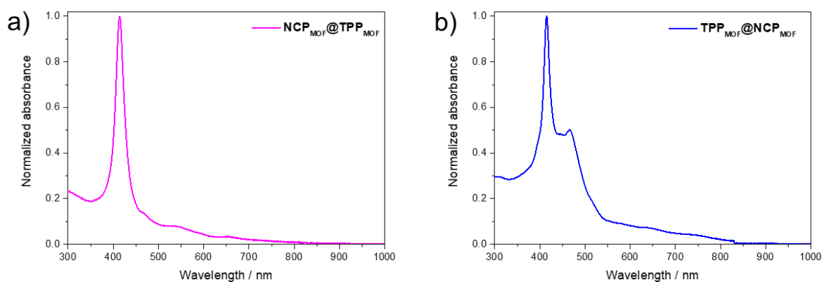
Figure 3-5. Absorption spectra of \text{NCP}_{\text{MOF}}@TPP_{\text{MOF}} (a) and \text{TPP}_{\text{MOF}}@NCP_{\text{MOF}} (b) dissolved in 0.1 M NaOH aqueous solution.
