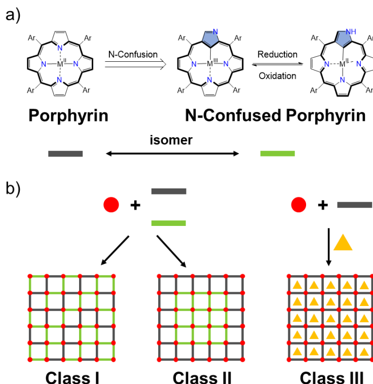
Figure 3-1. (a) Chemical structures of a regular porphyrin and an N-confused porphyrin used in this work: Ar = aryl groups, M = freebase or metals. (b) Schematic description of the classified structures of hybrid MOFs; Class I-III. The red circle, gray bar, green bar, and orange triangle indicate the metal ion, porphyrin linker, isomeric linker and guest molecule, respectively. 11
