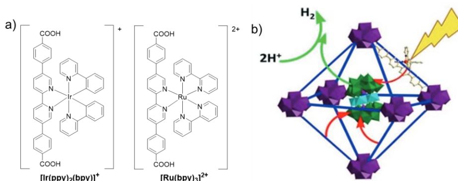
Figure 1-4. a) The structures of the organic ligands ( [\text{Ir}(\text{ppy})_2(\text{bpy})]^+ and [\text{Ru}(\text{bpy})_3]^{2+} ) used in the MOF synthesis. B) Water splitting reaction under light irradiation in the presence of MOF. 10a
