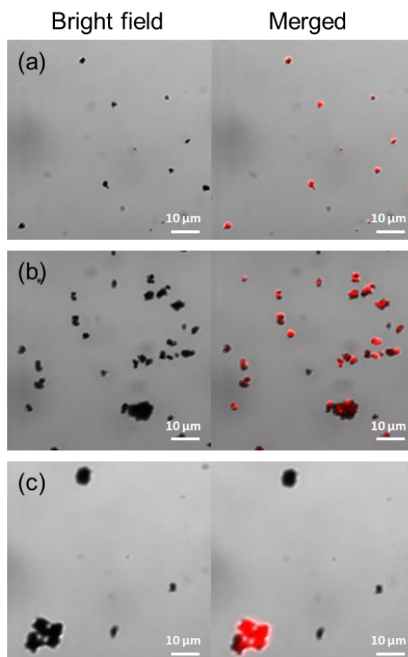
Figure 3-16. Fluorescent microscope images of (a) \text{NCP}_{\text{MOF}}@\text{TPP}_{\text{MOF}} , (b) \text{TPP}_{\text{MOF}}@\text{NCP}_{\text{MOF}} and (c) the mixture of \text{NCP}_{\text{MOF}} and \text{TPP}_{\text{MOF}} (5:2 ratio). The bright field images (left) and the merged fluorescent images (right, detect at 650 nm) are given with the scale bars of 10\ \mu\text{m} .
