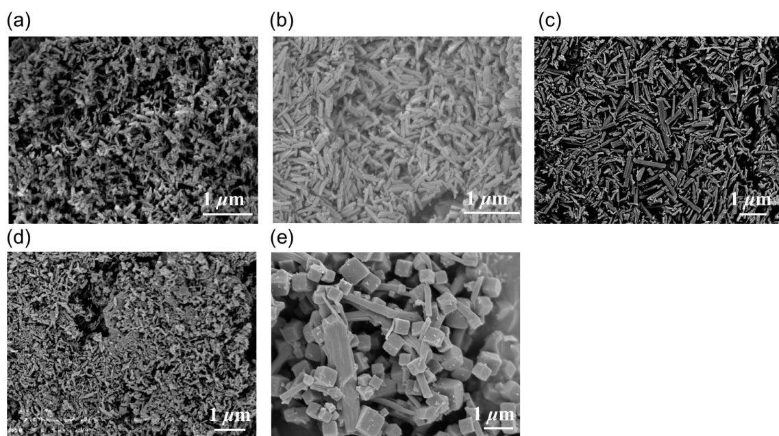
Figure 2-17. Selected SEM images of \text{NCP}_{\text{MOF}} fabricated under various conditions: (a) entry 1, (b) entry 2, (c) entry 3, (d) entry 5, and (e) entry 8.
