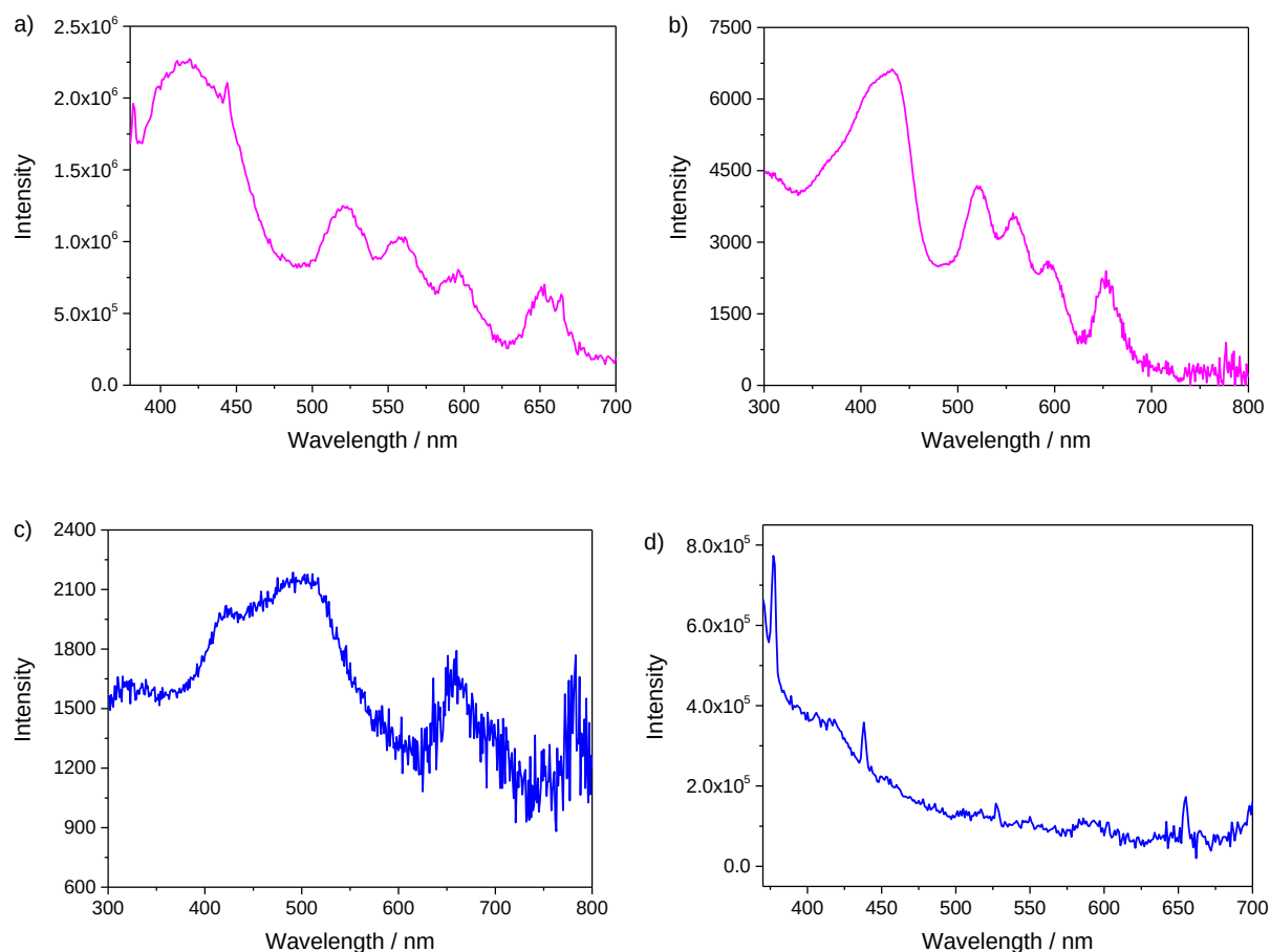
Figure 3-11. Photo-excitation spectra of \text{NCP}_{\text{MOF}}@\text{TPP}_{\text{MOF}} monitored at a) 730 nm and b) 910 nm. Photo-excitation spectra of \text{TPP}_{\text{MOF}}@\text{NCP}_{\text{MOF}} monitored at c) 900 nm and d) 720 nm.
