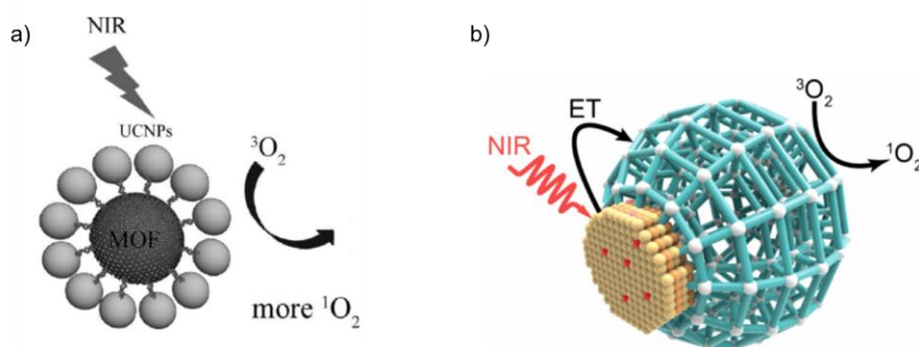
Figure 2-2. a) Self-assembled MOF–UCNP core–satellite in singlet oxygen generation, b) MOF growing on an upconversion nanoparticle. 13
