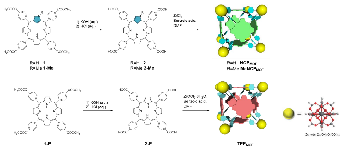
Scheme 2-1. Synthesis of NCP MOF , MeNCP MOF , and TPP MOF . The structures of MOFs shown here are the theoretical structures based on Rietveld refinement. The structure of Zr_6 cluster present in MOF-525 is drawn
