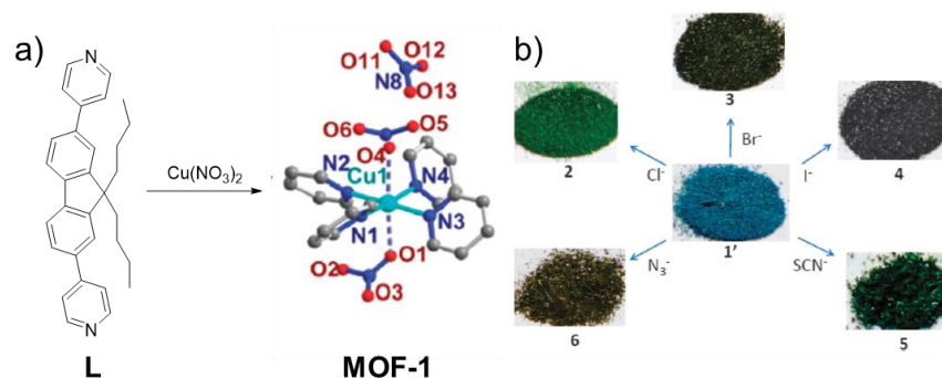
Figure 1-5. a) Synthesis of MOF-1 by ligand L and \text{Cu}^{2+} , b) color change resulted from the anion exchange. 11
