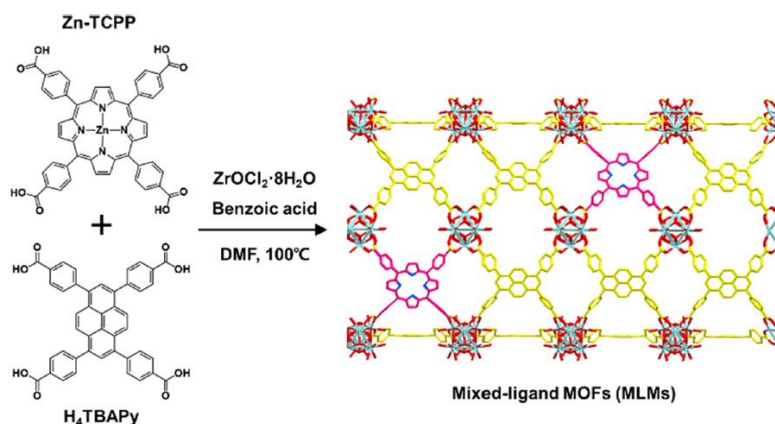
Figure 1-7. Synthesis of class I hybrid MOF with Zn-porphyrin and pyrene as the organic linkers. 13
