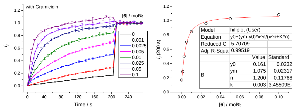
Figure 4-37. Hill plot analysis of H^+/Cl^- symport (or Cl^-/OH^- antiport) facilitated by compound 6 measured in the HPTS assay. NMDG (5 mM) was added before the addition of 6 at 0 s, and detergent was added at 200 s. Compound concentrations are shown as compound-to-lipid molar ratios. Error bars represent standard deviations from at least two repeats.
