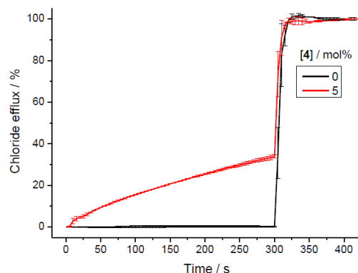
Figure 4-30. \text{Cl}^- efflux facilitated by compound 4 measured in the ISE anion exchange assay. The vesicles were loaded with an internal solution of NaCl (490 mM) buffered at pH 7.2 with 5 mM sodium phosphate salts and suspended in an external solution of \text{NaNO}_3 (490 mM) buffered at pH 7.2 with 5 mM sodium phosphate salts. Compound 4 was added at 0 s, and detergent at 300 s. Compound concentrations are shown as compound-to-lipid molar ratios. Error bars represent standard deviations from at least two repeats.
