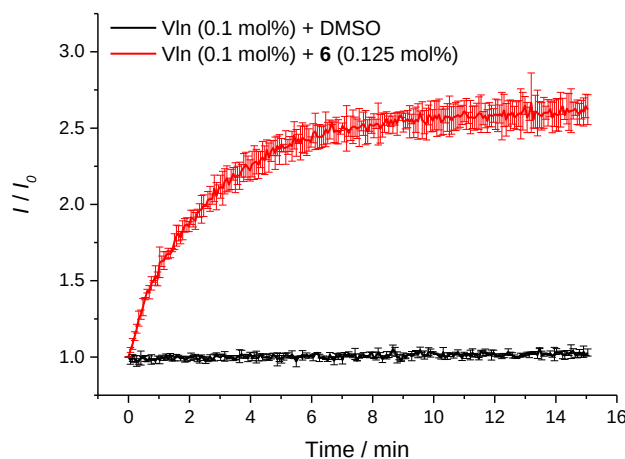
Figure 4-61. KBr efflux facilitated by a combination of Vln and compound 6 . Vln (0.1 mol%) was added, before the addition of 6 at 0 s. Compound concentrations are shown as compound-to-lipid molar ratios. Error bars represent standard deviations from at least two repeats.
