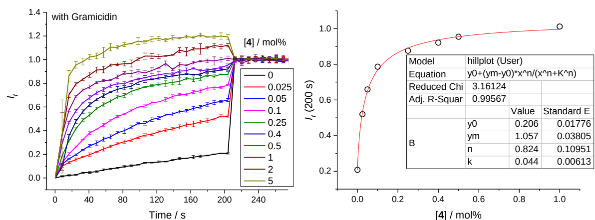
Figure 4-41. Hill plot analysis of H^+/NO_3^- symport (or NO_3^-/OH^- antiport) facilitated by compound 4 measured in the HPTS assay. NMDG (5 mM) was added before the addition of 4 at 0 s, and detergent was added at 200 s. Compound concentrations are shown as compound-to-lipid molar ratios. Error bars represent standard deviations from at least two repeats.
