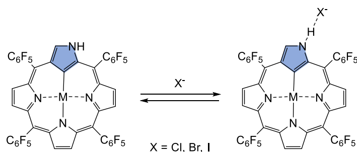
Scheme 1-5. NCP metal complex as halide receptor. 48a
