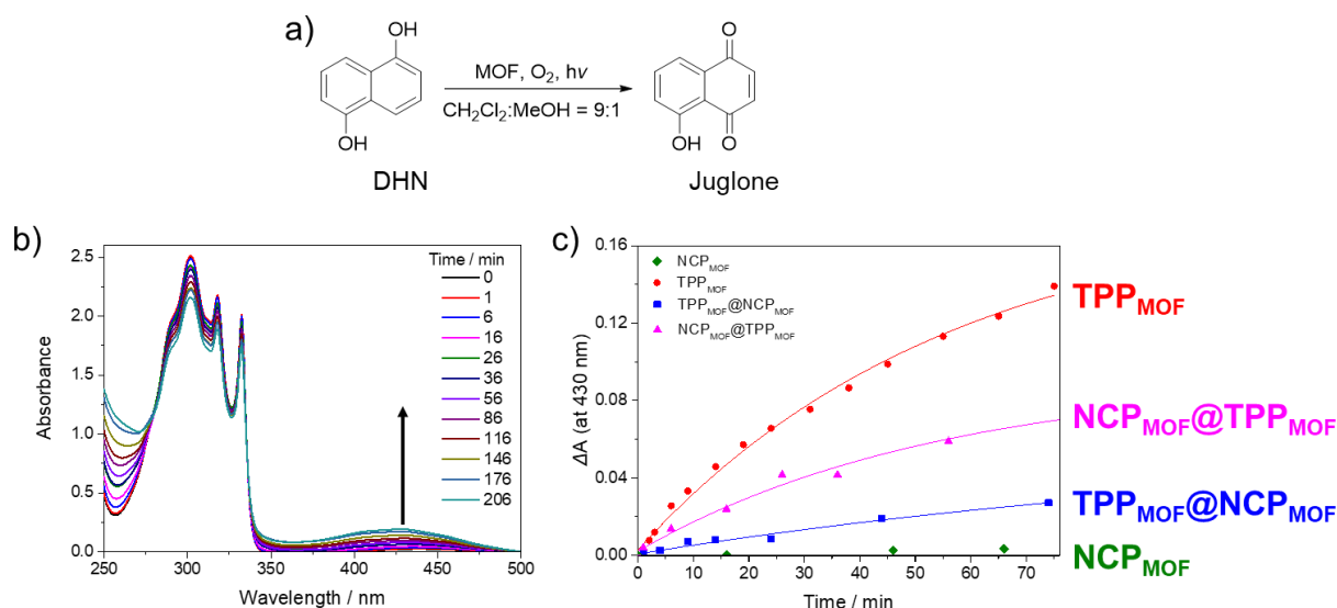
Figure 3-18. The monitoring of the generation of singlet oxygen by observing the change in the spectra of DHN.
