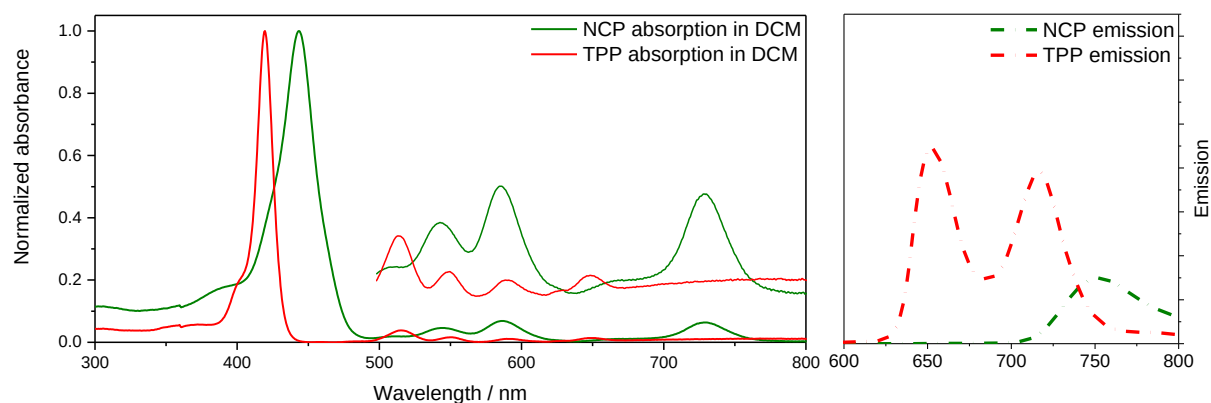
Figure 1-24. Absorption and emission spectra of TPP (red) and NCP (green) in DCM. (TPP: \lambda_{\text{ex}} = 420 nm, NCP: \lambda_{\text{ex}} = 444 nm)
