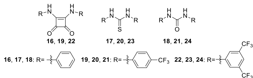
Figure 1-35. Anion transporters based on squaramide ( 16, 19, 22 ), thiourea ( 17, 20, 23 ) and urea ( 18, 21, 24 ). 64
