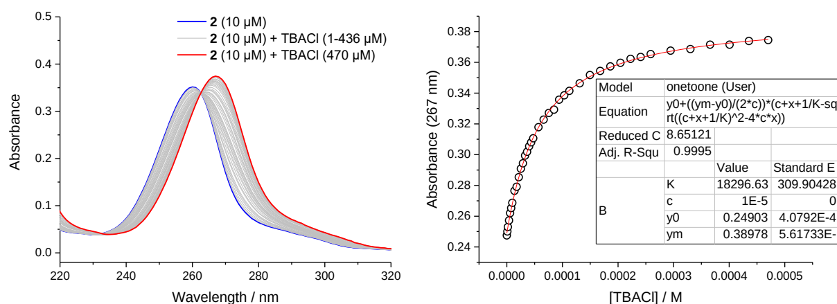
Figure 4-15 UV-vis titration of 2 (10 \mu\text{M} ) with TBACl (0–470 \mu\text{M} ) in \text{CH}_3\text{CN} at 298 K.
