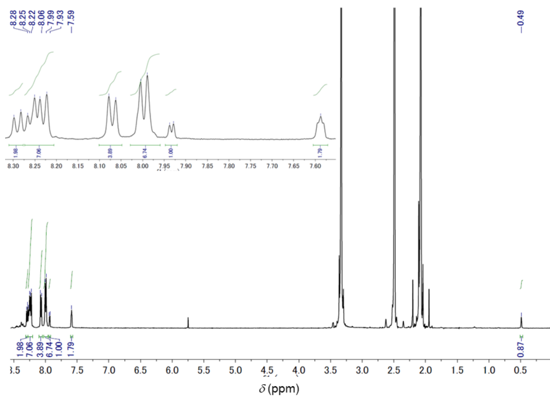
Figure 2-15. 1 H NMR spectrum of 2 in DMSO- d 6 .
