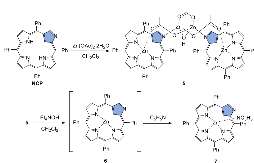
Figure 1-25. The reaction between NCP and zinc acetate. 45
