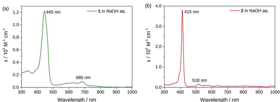
Figure 3-6. UV/vis absorption spectra of (a) 1 and (b) 2 in NaOH aq.
