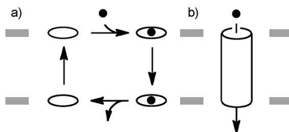
Figure 1-29. Schematic transport mechanism of a) ion carriers and b) ion channels. 58
