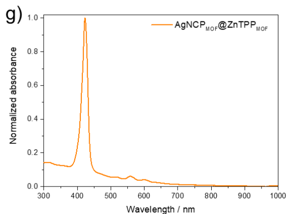
Figure 3-19. Absorption spectra of \text{NCP}_{\text{MOF}} (a), \text{TPP}_{\text{MOF}} (b), mixture ( \text{NCP}_{\text{MOF}}:\text{TPP}_{\text{MOF}}=5:2 ) (c), \text{ZnTPP}_{\text{MOF}} (d), \text{AgNCP}_{\text{MOF}} (e), \text{ZnTPP}_{\text{MOF}}@\text{AgNCP}_{\text{MOF}} (f) and \text{AgNCP}_{\text{MOF}}@\text{ZnTPP}_{\text{MOF}} (g) dissolved in 0.1 M NaOH aqueous solution.
