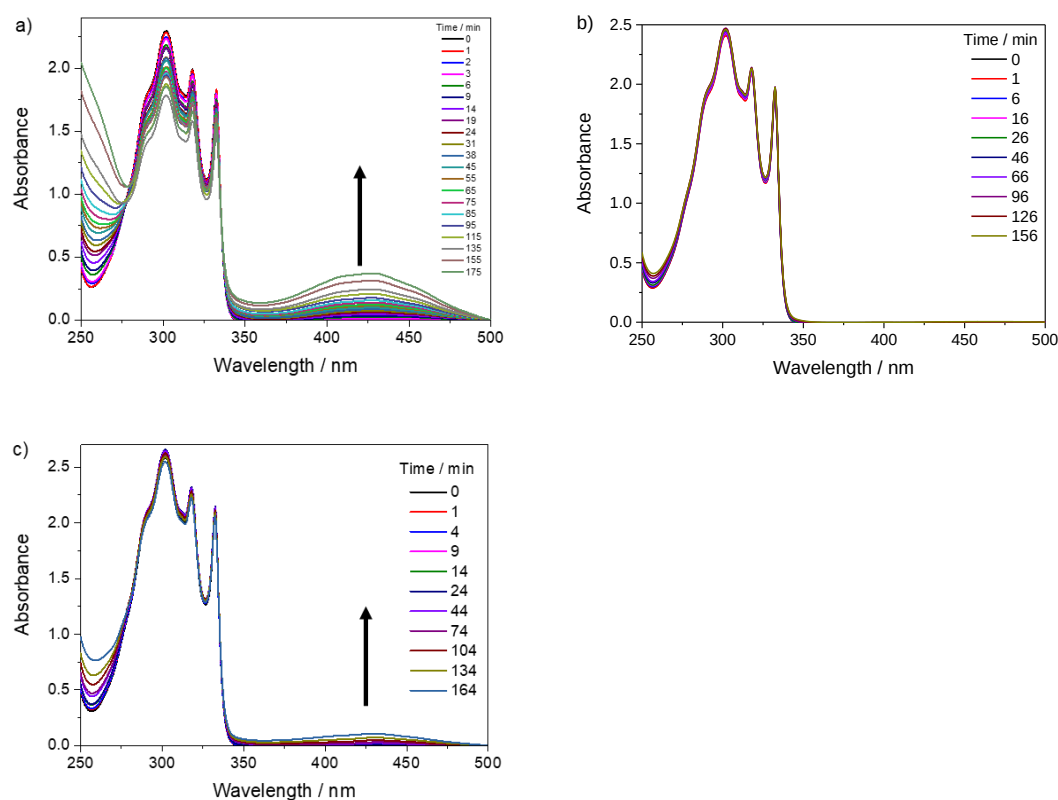
Figure 3-23. Spectral changes of DHN when treated with a) TPP MOF , b) NCP MOF , c) TPP MOF @NCP MOF and irradiated with light at wavelengths at 450–700 nm.
