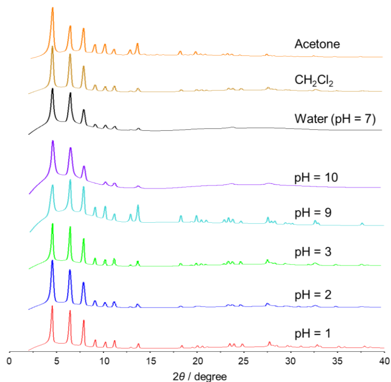
Figure 2-9. Powder X-ray diffraction patterns of \text{NCP}_{\text{MOF}} after immerse in different chemical environments for 24 h.
