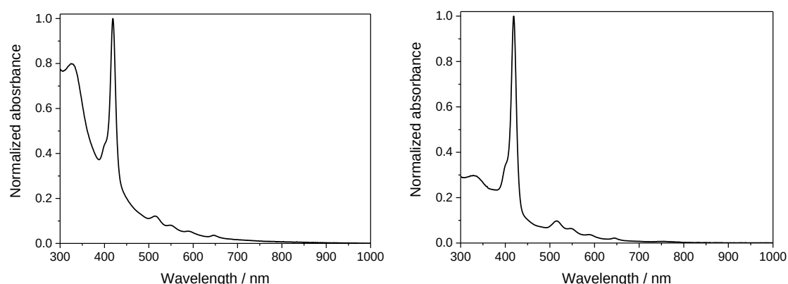
Figure 3-2. UV/vis/NIR spectra of filtrates after NCP MOF @TPP MOF (left) and TPP MOF @NCP MOF (right) was filtered.
