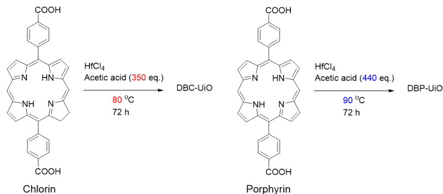
Figure 2-5. Different synthesis conditions for DBC-UiO 18 and DBP-UiO 17 with chlorin and porphyrin as the organic ligands respectively.
