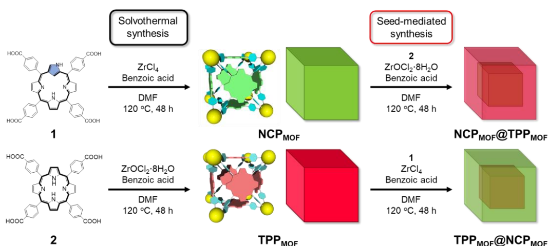
Scheme 3-1. Schematic description for synthetic strategies of hierarchical hybrid MOFs, \text{NCP}_{\text{MOF}}@ \text{TPP}_{\text{MOF}} , and \text{TPP}_{\text{MOF}}@ \text{NCP}_{\text{MOF}} through a seed-mediated ligand exchange reaction.
