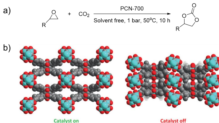
Figure 1-3. a) The reduction of carbon dioxide with epoxide in the presence of PCN-700, b) the catalyst on and catalyst off state of PCN-700. 9
