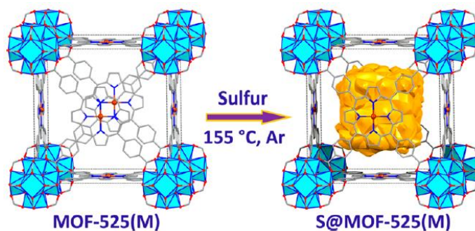
Figure 1-12. Schematic illustration of S@MOF-525 synthesized through the melt-diffusion method at 155 °C under an Ar atmosphere. 18
