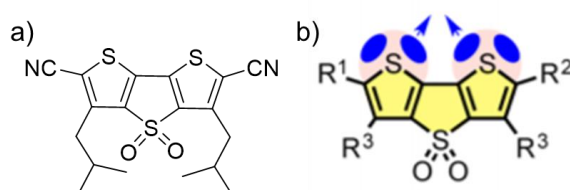
Figure 1-38. a) structure of transporter based on Dithienothiophene and b) diagram the \sigma -hole. 67
