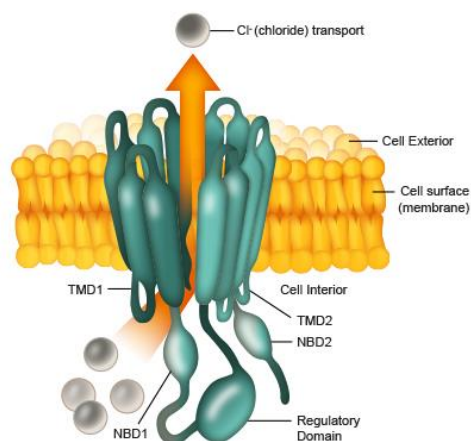
Figure 1-28. Diagram of Cl - transport channel protein. 57
