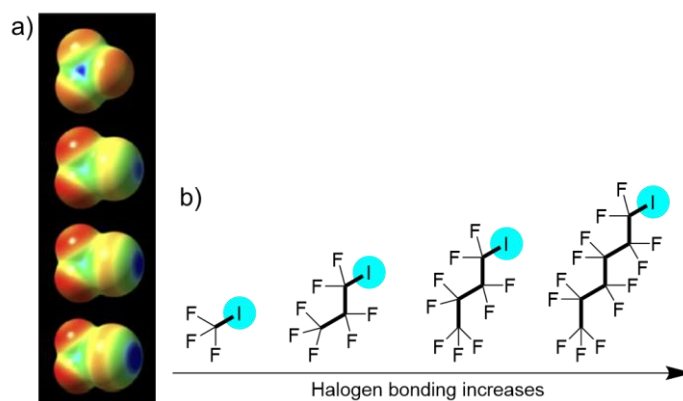
Figure 1-37. a) Electrostatic potential surfaces of \text{CF}_4 , \text{CF}_3\text{Cl} , \text{CF}_3\text{Br} and \text{CF}_3\text{I} (top to bottom), b) enhancement of halogen bonding with the increase of the electron-withdrawing ability of the side chain. 66
