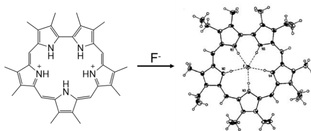
Figure 1-19. Fluoride binding using protonated sapphyrin. 30
