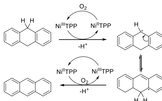
Figure 1-16. A possible reaction pathway for the aerobic dehydrogenation of 9,10-dihydroanthracene. 22
