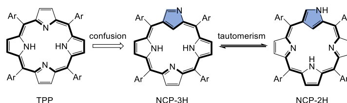
Figure 1-23. Structures of porphyrin and N-confused porphyrin and its NH-tautomerism.
