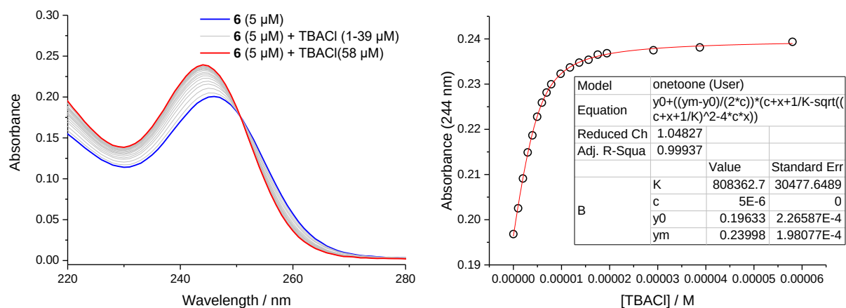
Figure 4-27. UV-vis titration of 6 (5 \mu\text{M} ) with TBACl (0–58 \mu\text{M} ) in \text{CH}_3\text{CN} at 298 K.
