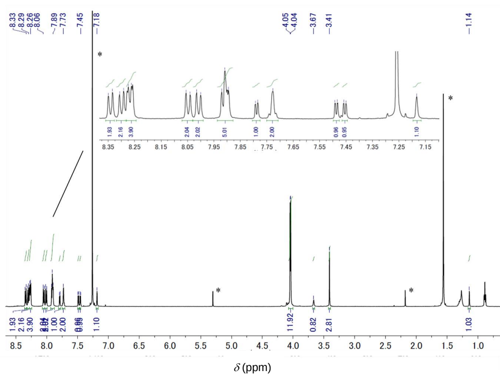
Figure 2-14. 1 H NMR spectrum of 1-Me in CDCl 3 .
