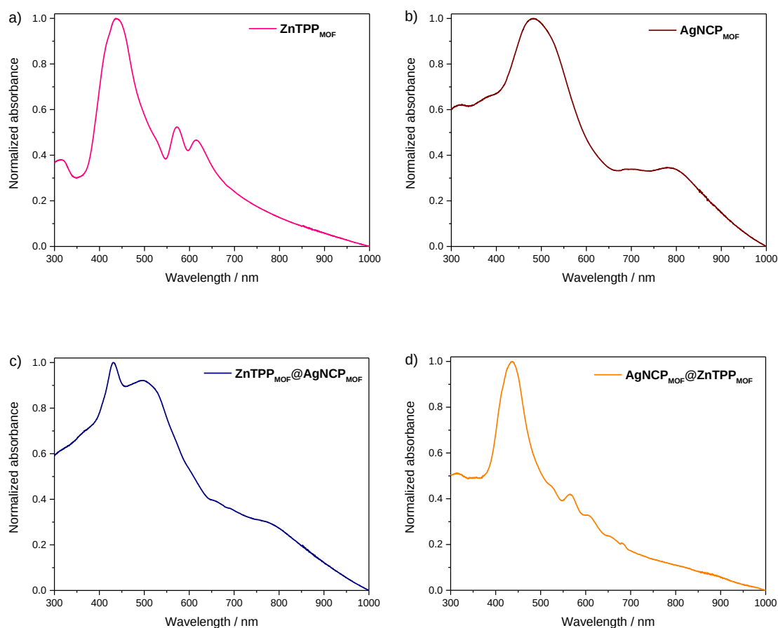
Figure 3-20. UV-vis absorption spectra of the KBr pellet containing (a) \text{ZnTPP}_{\text{MOF}} , (b) \text{AgNCP}_{\text{MOF}} , (c) \text{ZnTPP}_{\text{MOF}}@\text{AgNCP}_{\text{MOF}} and (d) \text{AgNCP}_{\text{MOF}}@\text{ZnTPP}_{\text{MOF}} .
