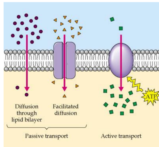
Figure 1-27. Diagram of three types of transmembrane transports. 56a
