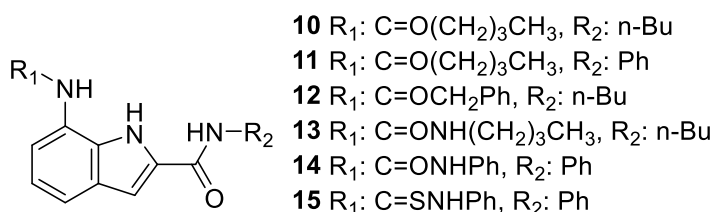
Figure 1-33. A group of simple transporters (compound 10-15 ) based on indoles. 55
