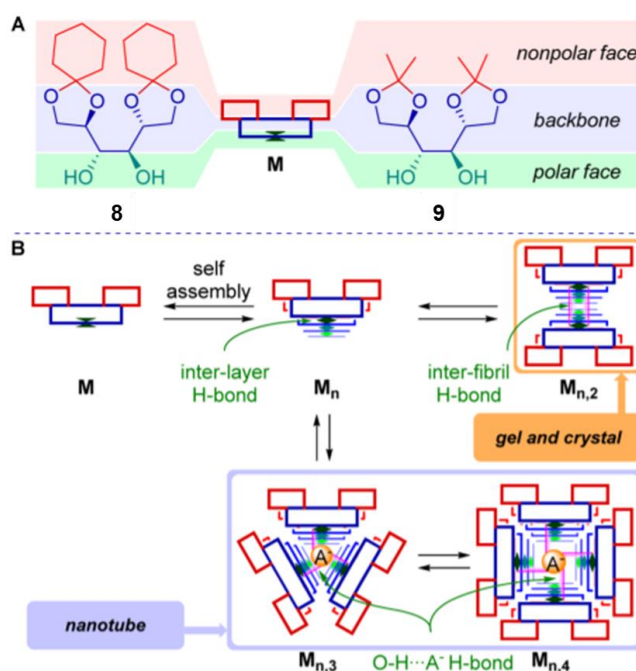
Figure 1-31. Structures of synthetic ion channels constructed from small molecules. 60 A, the molecular design of channel unit compound 8 and 9; B, the self-assembly of channel units in a hydrophobic environment.
