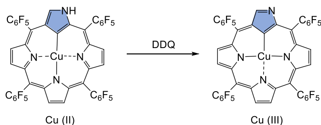
Scheme 1-3. The oxidation of Cu(II)-NCP to Cu(III)-NCP. 46
