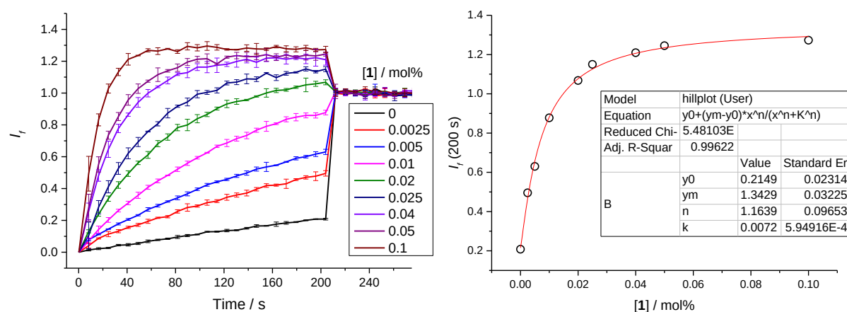
Figure 4-38. Hill plot analysis of H + /NO 3 - symport (or NO 3 - /OH - antiport) facilitated by compound 1 measured in the HPTS assay. NMDG (5 mM) was added before the addition of 1 at 0 s, and detergent was added at 200 s. Compound concentrations are shown as compound-to-lipid molar ratios. Error bars represent standard deviations from at least two repeats.
