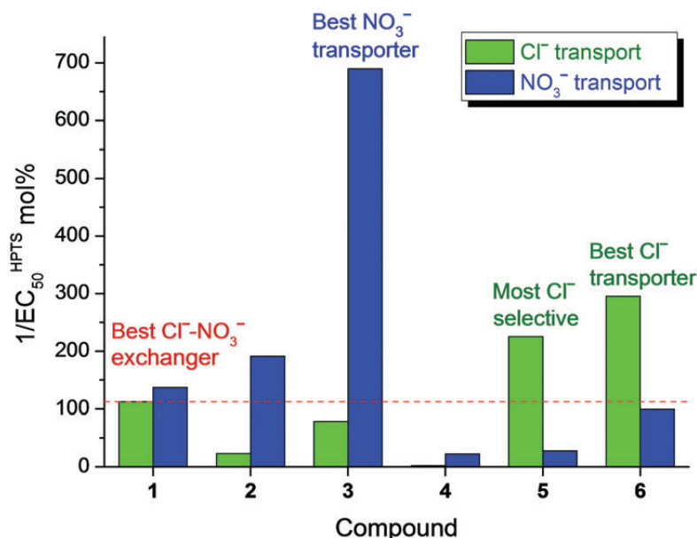
Figure 4-5. Histogram showing activities of 1–6 in facilitating uniport of Cl − (green bars) and NO 3 − (blue bars). Activities are expressed as reciprocal of EC 50 values (at 200 s) determined in the HPTS assay. The red dashed line shows that compound 1 has the highest activity in facilitating the slower anion uniport process, which explains its highest activity in the Cl − –NO 3 − exchange assay.
