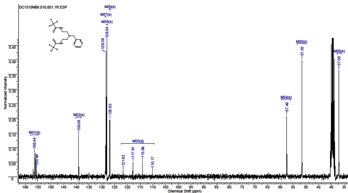
Figure 4-11. 13 C NMR (75 MHz) spectrum of 4 in DMSO- d 6 .
