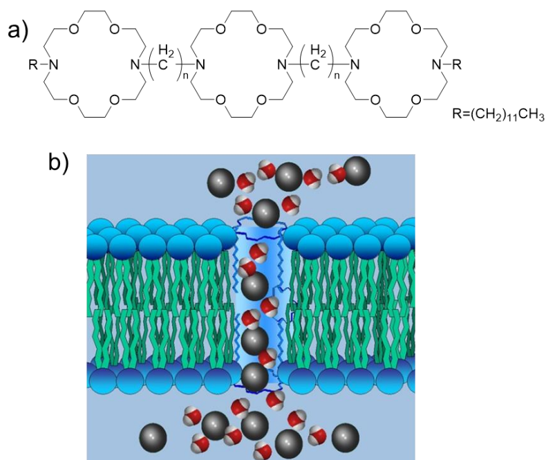
Figure 1-30. (top) The molecular structure of ion channel based on crown ether, (bottom) schematic of ion transport in cell membrane. 59
