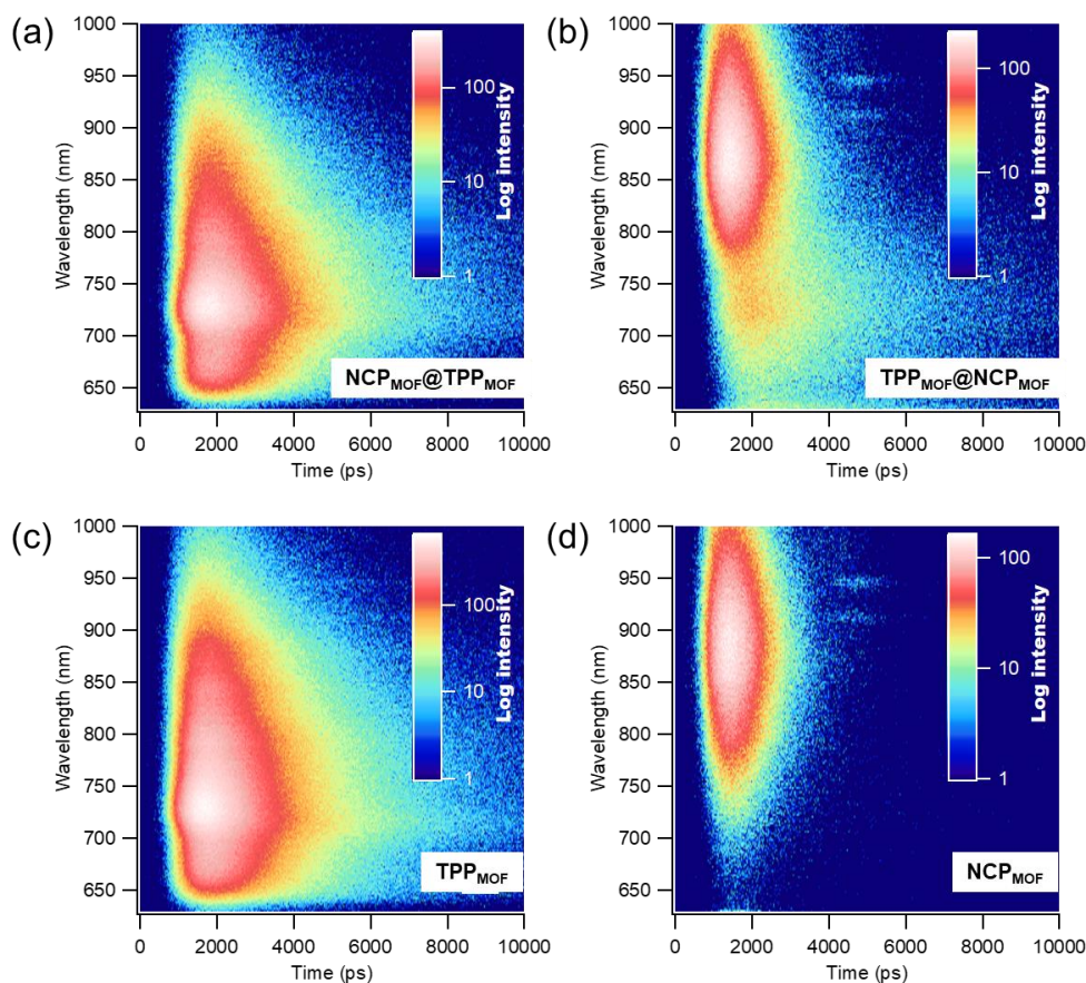
Figure 3-14. Time-resolved 2D fluorescence spectra of the hybrid MOFs; (a) NCP MOF @TPP MOF and (b) TPP MOF @NCP MOF . The data for the reference of (c) TPP MOF and (d) NCP MOF are shown. The excitation was subjected at \lambda_{\text{ex}} = 532 nm.
