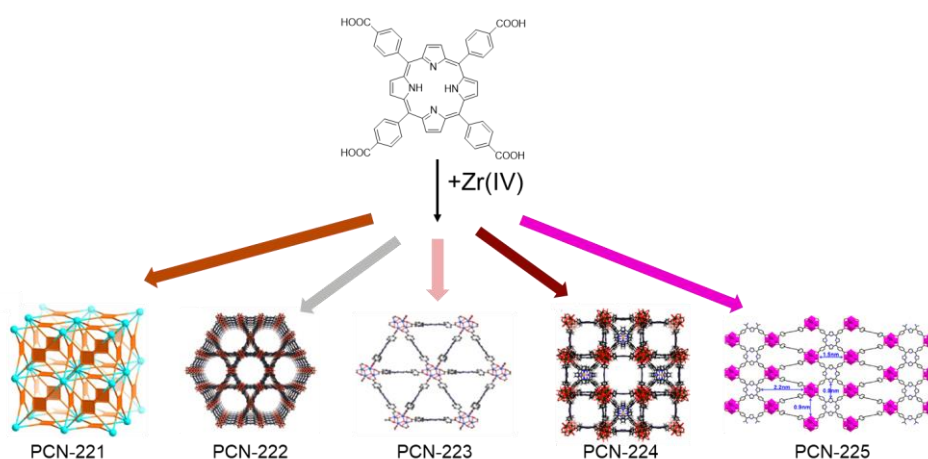
Figure 1-21. Topologies of PCN series of MOFs based on porphyrin and Zr(IV) as the building block. 35
