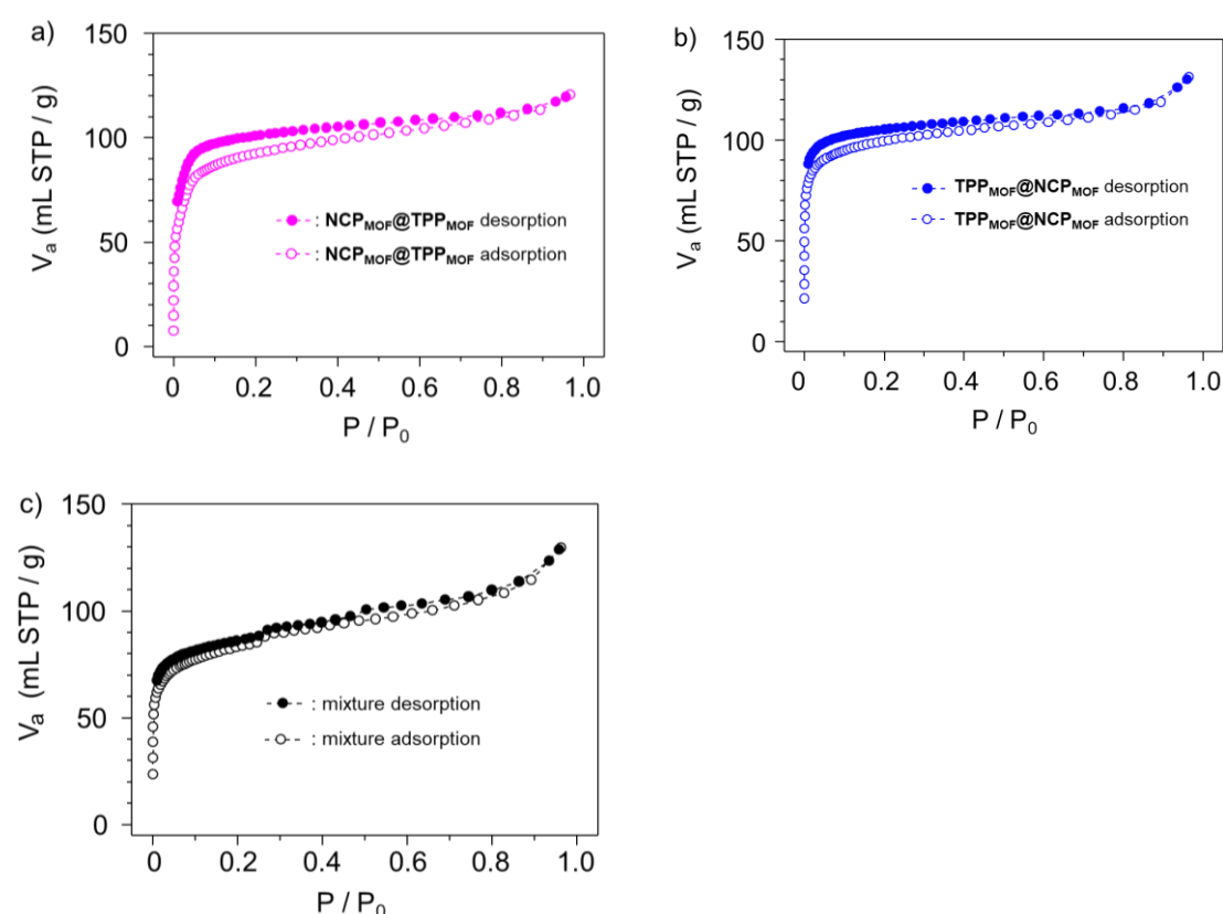
Figure 3-8. \text{N}_2 adsorption isotherms of a) \text{NCP}_{\text{MOF}}@\text{TPP}_{\text{MOF}} , b) \text{TPP}_{\text{MOF}}@\text{NCP}_{\text{MOF}} and c) mixture ( \text{NCP}_{\text{MOF}} : \text{TPP}_{\text{MOF}} = 5:2 ) at 77 K.
