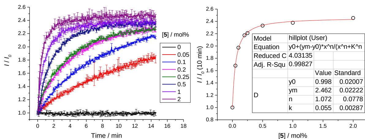
Figure 4-48. Hill plot analysis of \text{Cl}^- transport facilitated by compound 5 measured in the Osmotic assay. Vln (0.1 mol%) was added, before the addition of 5 at 0 s. Compound concentrations are shown as compound-
