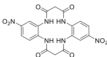
Figure 1-34. structure of cyclic transporter molecule. 63
