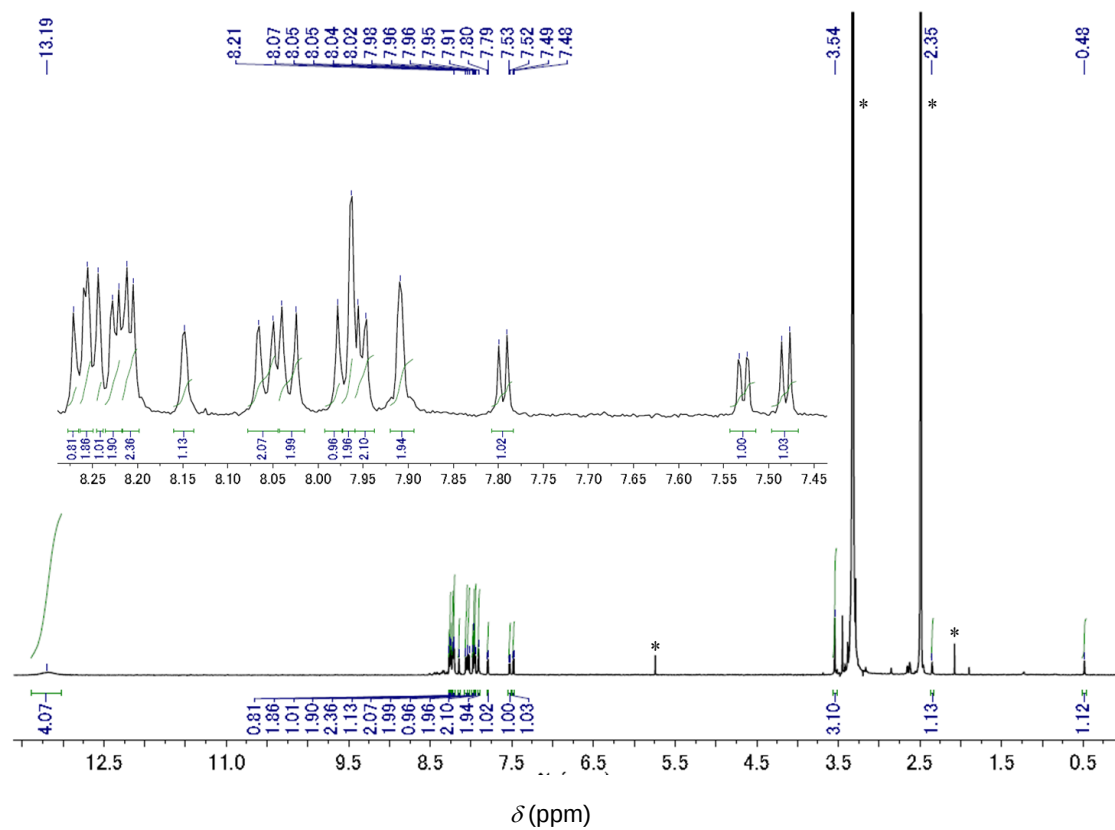
Figure 2-16. 1 H NMR spectrum of 2-Me in DMSO- d 6 .
