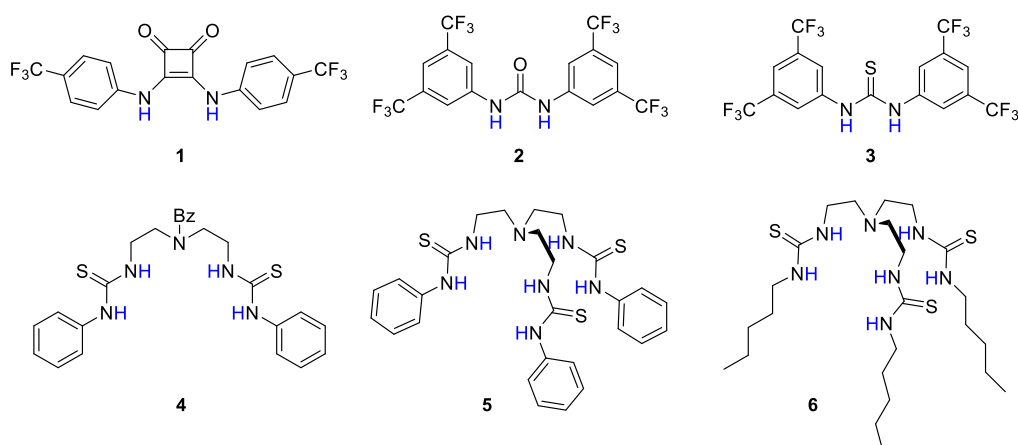
Figure 4-3. Structures of anion transporters 1–6 .
