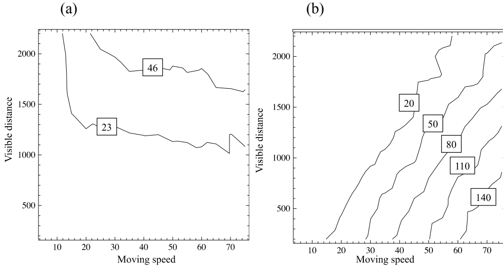
Figure 2. Results of simulations shown in contour plots. (a) Number of food items consumed. The horizontal axis is movement speed v , and the vertical axis is visible distance R . More food items are consumed with longer visual distances R and faster movement speeds v . (b) Number of collisions. Axes are the same as in (a). The risk of collision is higher for short visual distances R and faster movement speeds v . Parameters are: r = 30 , f = 40 .
