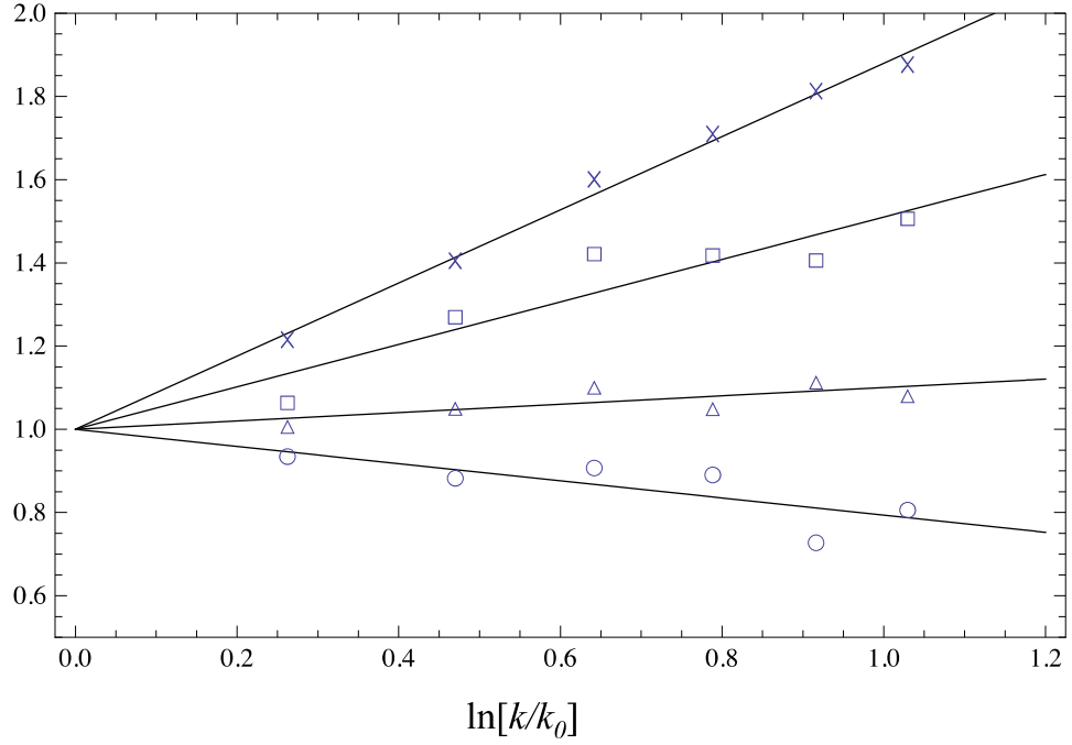
Figure 5. Speed sensitivity \alpha depends on four parameters ( r, f, c , and d ). I chose the standard values of parameters as: f = 40 , r = 20 , c = 3 , and d = 3 . I increased the four parameters (e.g., k ) by multiplying them by 1.3, 1.6, 1.9, 2.1, 2.4, and 2.7, with the other parameters unchanged. The horizontal axis is the change in the logarithm of k (i.e., \ln[k/k_0] ), and the vertical axis is the change in \alpha (i.e., \alpha/\alpha_0 ). Different symbols represent different parameters that were changed: crosses represent the number of obstacles r ; circles represent the number of food items f ; triangles represent the cost of eyes c ; and squares represent the damage by collisions d .
