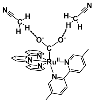
Figure 9. Speculated structure of the CO 2 -bound [Ru_Me] + forming intermolecular hydrogen bond with MeCN molecules.
