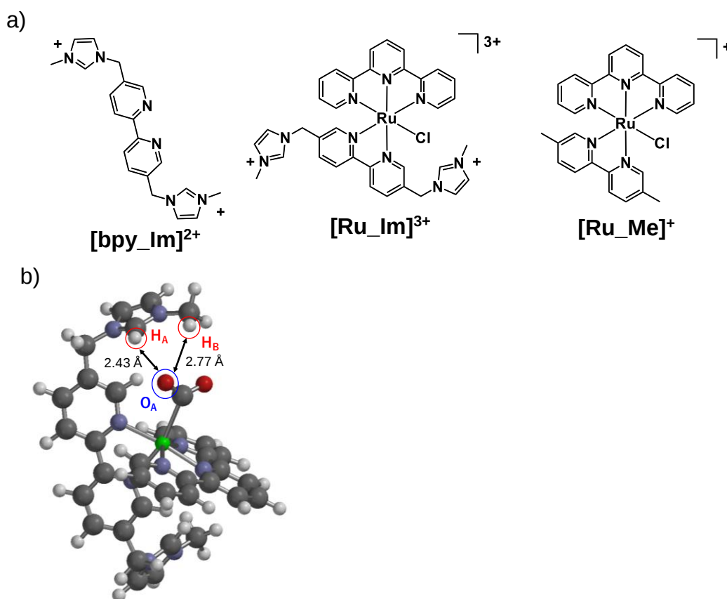
Figure 2. a) Molecular structures of compounds studied in this work. b) A structure of the CO 2 -bound [Ru_Im] 3+ computed by MMFF94.
