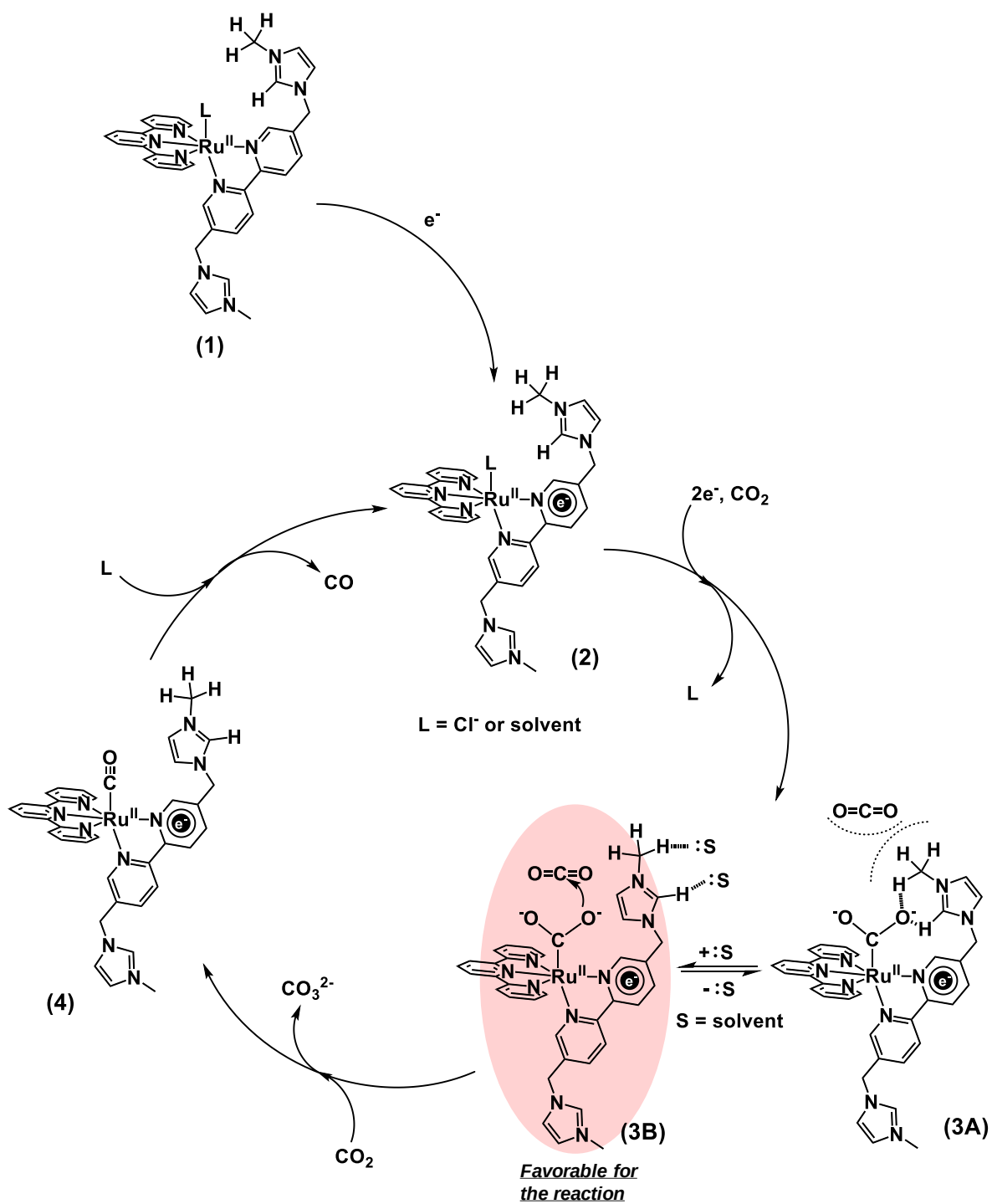
Figure 11. A speculated catalytic cycle for [\text{Ru\_Im}]^{3+} .
