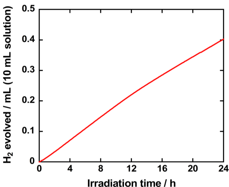
Figure 15. Photochemical H 2 production from an aqueous acetate buffer solution (pH 5.0, 10 mL; at 20 °C under Ar) containing 0.1 mM [\text{PtCl}_2(\text{bpyMV2})]^{4+} , 0.1 M NaCl, and 30 mM EDTA.
