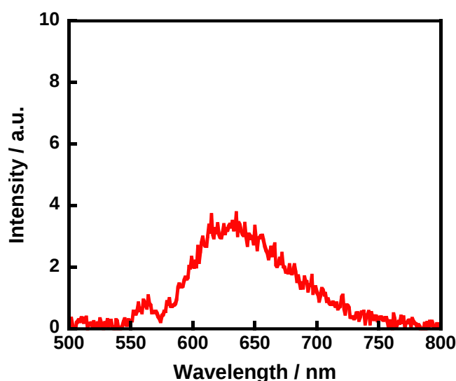
Figure 8. An emission spectrum recorded for an aqueous acetate buffer solution (0.1 M, pH 5.0) of [Ru(bpy)MV2]_3(PF_6)_{14} at 20 °C under Ar. The excitation wavelength was 470 nm and the solution had 0.05 of absorbance at 470 nm.
