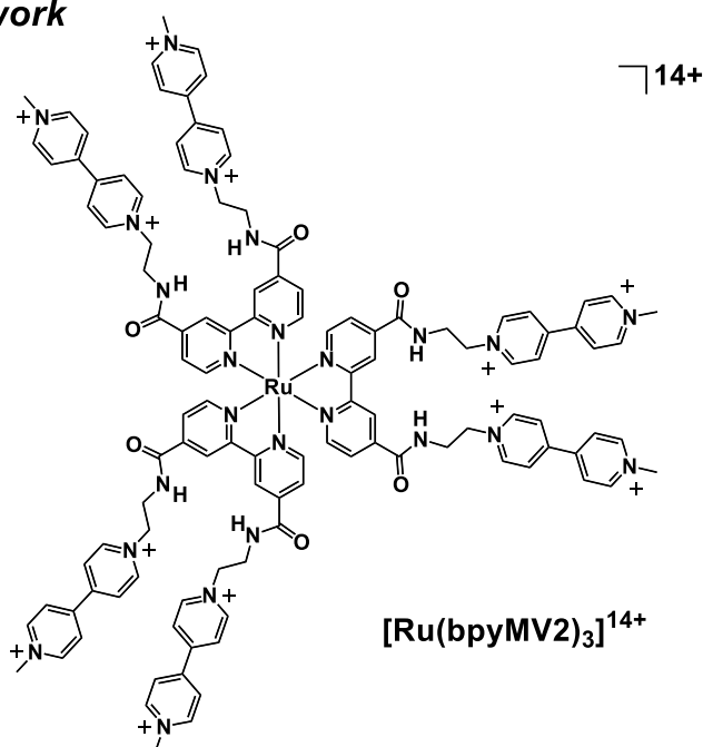
Figure 2. A molecular structure of [\text{Ru}(\text{bpyMV2})_3]^{14+} studied in this work.
