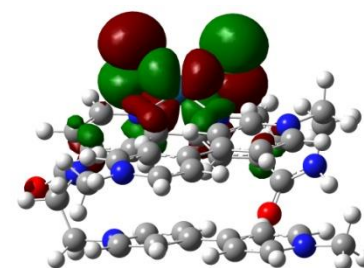
MO193 \alpha (HOMO-1)
