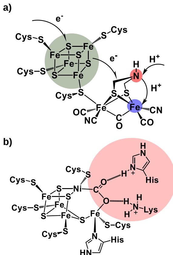
Figure 1. Structures of catalytic active centers of a) [FeFe]-hydrogenase and b) \text{CO}_2 -bound CO-dehydrogenase.
