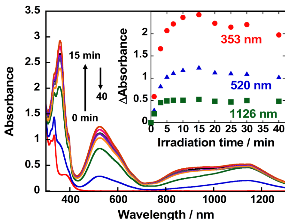
Figure 8. Spectral changes during the photolysis of an aqueous acetate buffer solution (pH 5.0; at 20 °C under Ar) containing 0.1 mM [\text{PtCl}_2(\text{bpyMV2})]^{4+} , 0.1 M NaCl, and 30 mM EDTA. Inset: Absorbance changes at 353 nm (red), 520 nm (blue), and 1126 nm (green) during photolysis.
