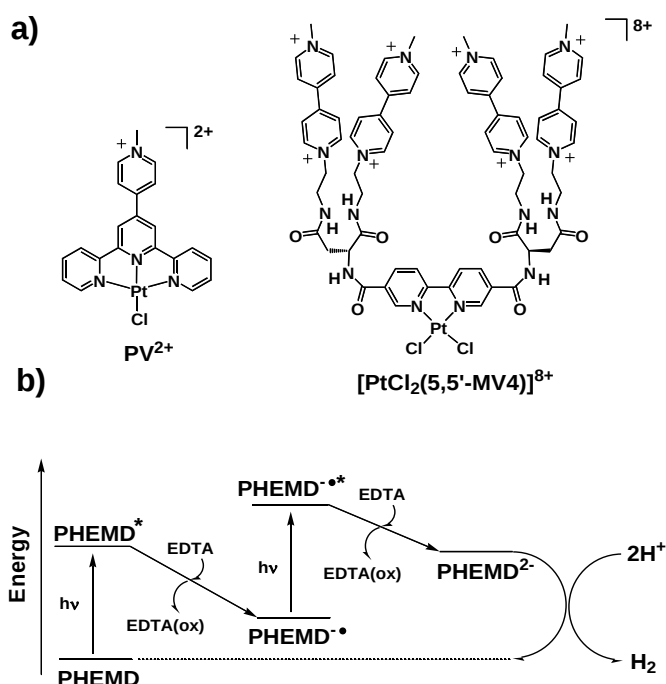
Figure 1. a) Examples of PHEMDs . b) Z-scheme photosynthesis by a PHEMD .
