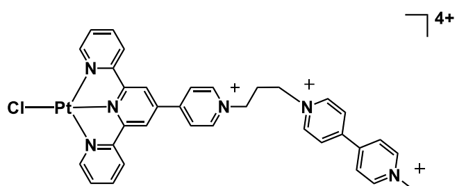
[Pt(L-C1-MV1)Cl] 4+
