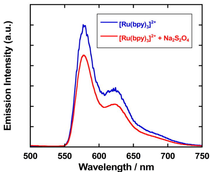
Figure 22. Emission spectra (excitation at 425 nm) of 0.01 mM [\text{Ru}(\text{bpy})_3](\text{NO}_3)_2 \cdot 3\text{H}_2\text{O} before (blue line) and after (red line) adding \text{Na}_2\text{S}_2\text{O}_4 . The solution was prepared by dissolving the compound in a 1:2 mixture of water and ethylene glycol (0.25 mL) and was sealed in a quartz EPR tube under He. Other conditions are same to those described above. Note that the emission intensity was quite sensitive to the manually tuned position of each sample so that quantitative comparison of the emission intensities does not make sense.
