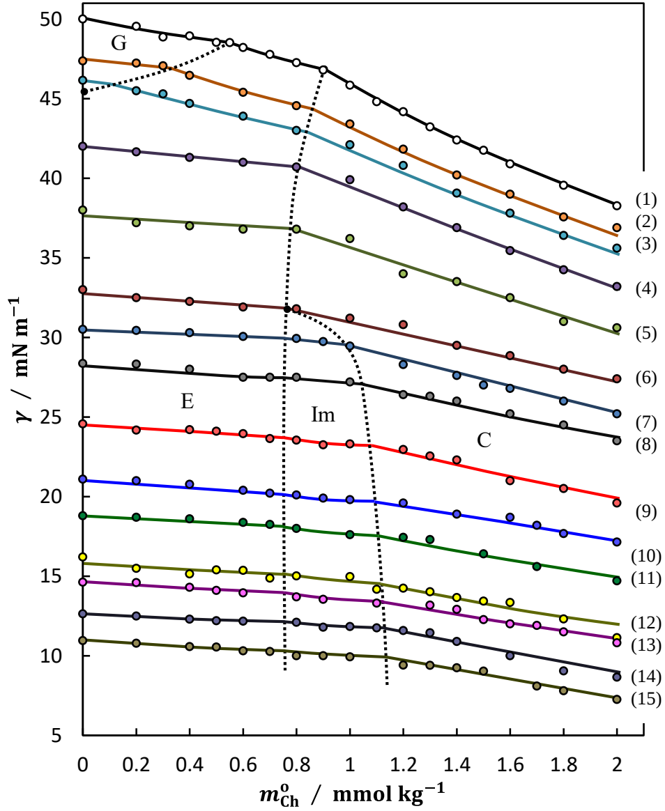
Figure 2-13. The \gamma vs. m_{\text{Ch}}^0 curves at given (1) m_{\text{PC}}^w = 0 (pure Chol system), (2) 0.001, (3) 0.0015, (4) 0.002, (5) 0.003, (6) 0.004, (7) 0.005, (8) 0.007, (9) 0.01, (10) 0.015, (11) 0.02, (12) 0.03, (13) 0.04, (14) 0.05, and (15) at 0.06 mmol kg -1 . The dotted lines connect the phase transition points of the film.
