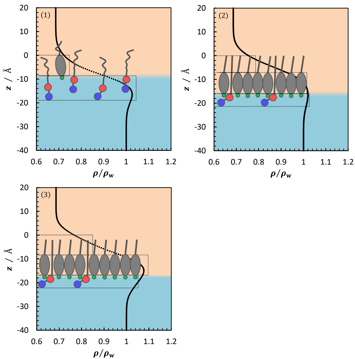
Figure 2-26. The electron density profiles normal to the interface under m_{\text{PC}}^{\text{w}} = 0.002
