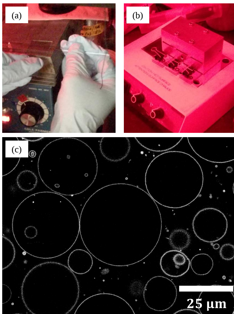
Figure 4-2. The procedure of GUVs Preparation. (a) Lipid solution was spread onto ITO glass on hotplate at \sim 55^{\circ}\text{C} . (b) Setup of heating and application of AC field. The clip fastening two ITO glasses connects to AC field apparatus. (c) Typical GUVs image obtained as a result of this procedure.
