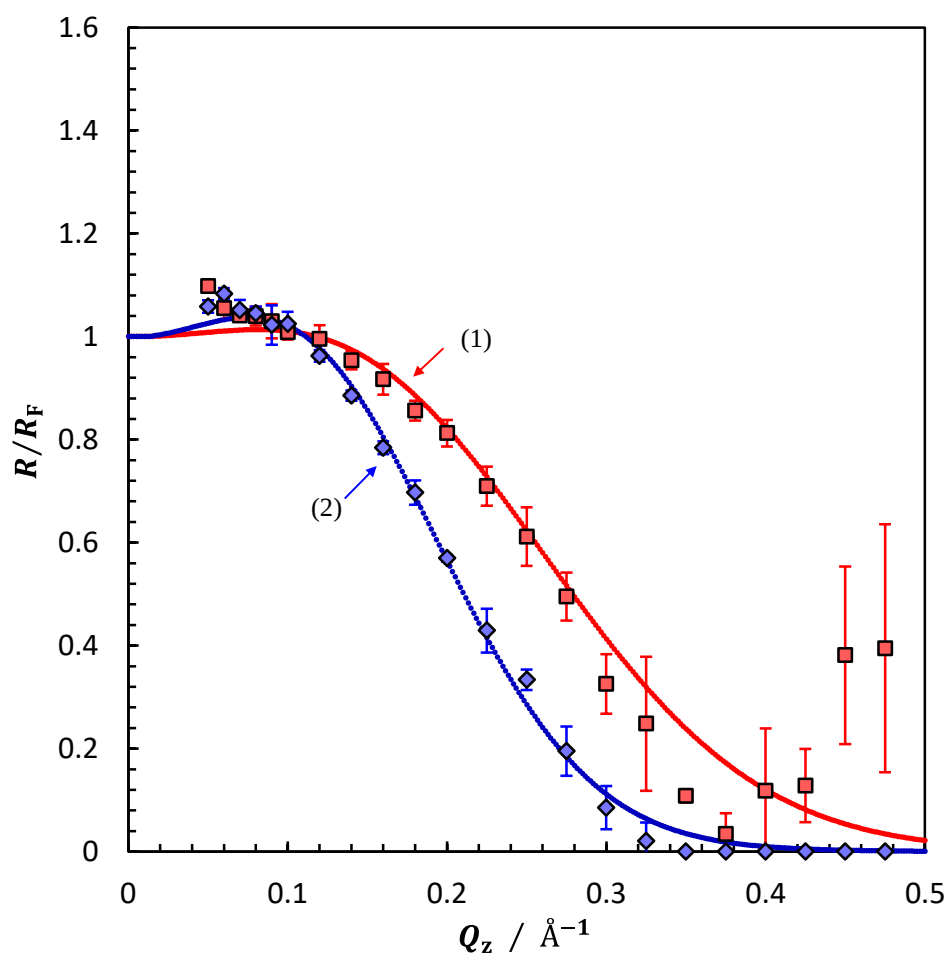
Figure 2-7. The R/R_F vs. Q_z plots in the pure C14PC system (1) at m_{\text{PC}}^w = 0.005 and (2) at 0.03 \text{ mmol kg}^{-1} . The dotted lines represent the fitting curves.
