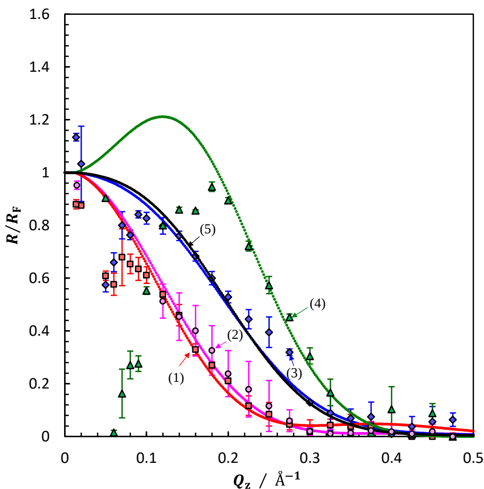
Figure 3-7-2. The R/R_F vs. Q_z plots under fixed X_{\text{Ch}} = 0.90 at (1) m = 0.4 , (2) 0.8 , (3) 1.2 , and (4) at 4.4 \text{ mmol kg}^{-1} . The dotted lines except black one represent the fitting curves by the slab model. The black dotted line (5) was resulted from domain fitting by the incoherent model with C_{\text{XR}} = 0.42 . It is noted that the domain fitting was carried out using the fitting curves instead of corresponding plots because the plots have defects at low Q_z .
