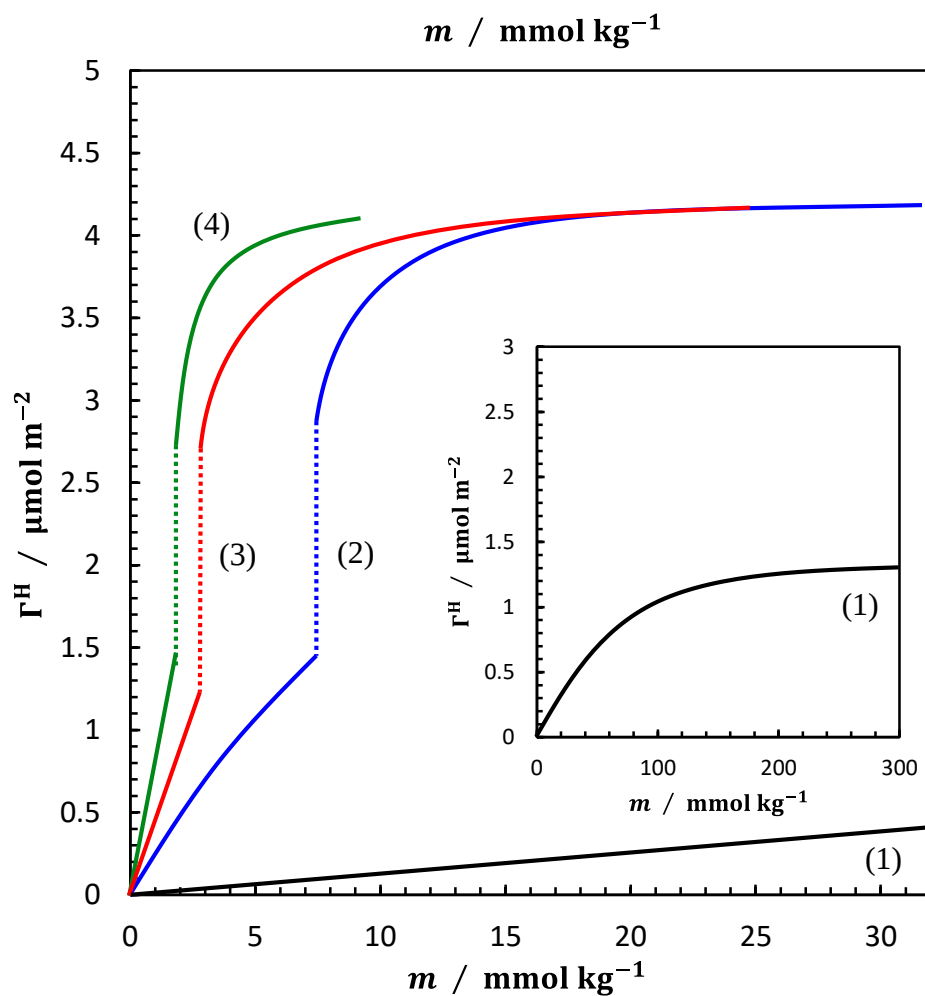
Figure 3-3-1. The \Gamma^H vs. m curves at given (1) X_{Ch} = 0 (pure MePa system), (2) 0.10, (3) 0.21, and (4) at 0.40. The inset shows the reduced curve 1.
