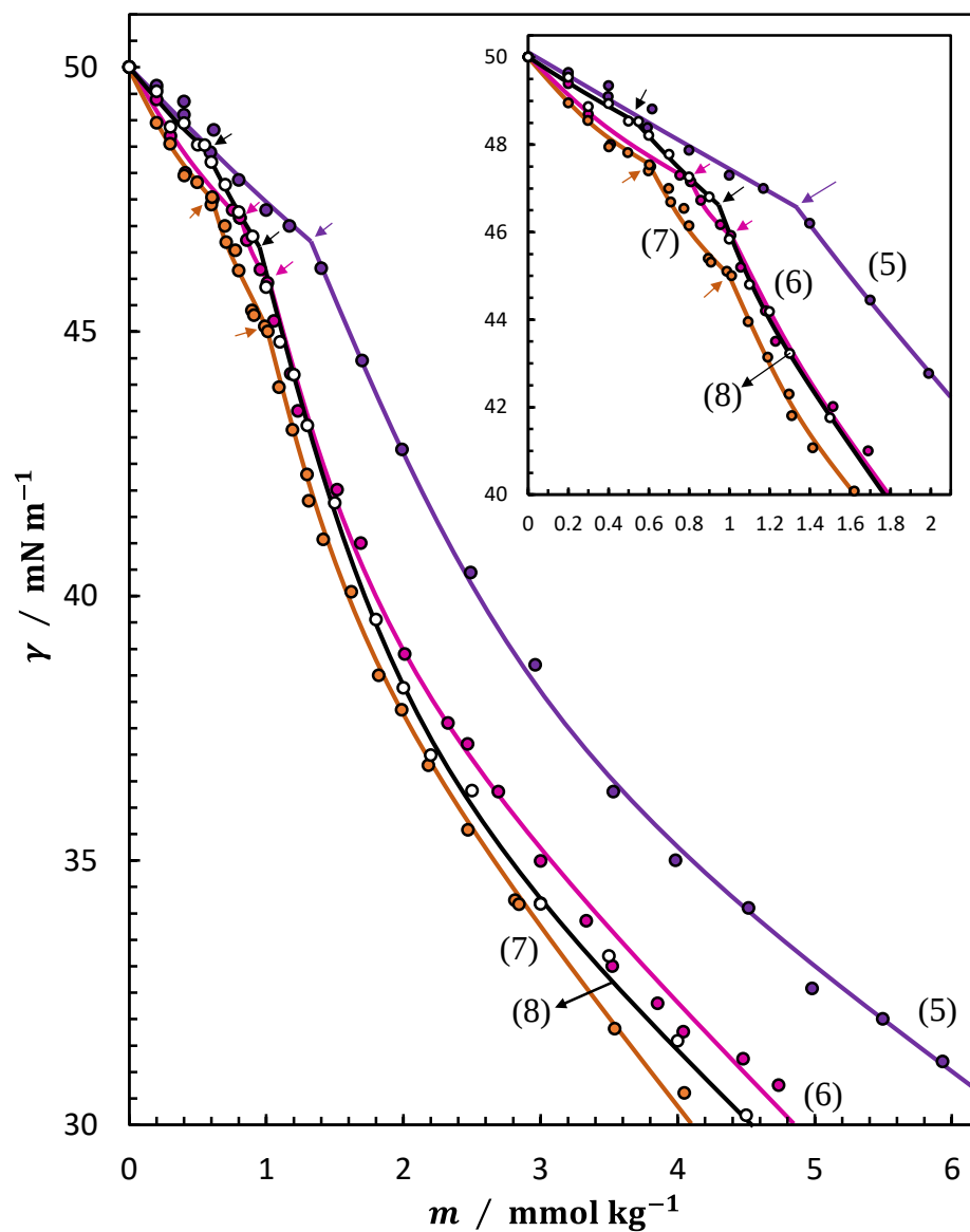
Figure 3-1-2. The \gamma vs. m curves at given (5) X_{\text{Ch}} = 0.61 , (6) 0.79, (7) 0.90, and (8) at 1 (pure Chol system). The arrows indicate the phase transition points. The curves at low m are manifested in the inset.
