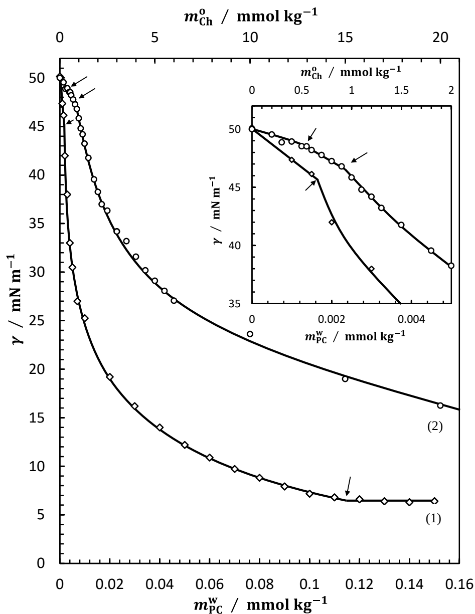
Figure 2-4. (1) The \gamma vs. m_{\text{PC}}^w curve in the pure C14PC, and (2) the \gamma vs. m_{\text{Ch}}^o curve in the pure Chol systems. Arrows indicate the kink points corresponding to the phase transition points and CMC. The inset expands the phase transition points on both curves.
